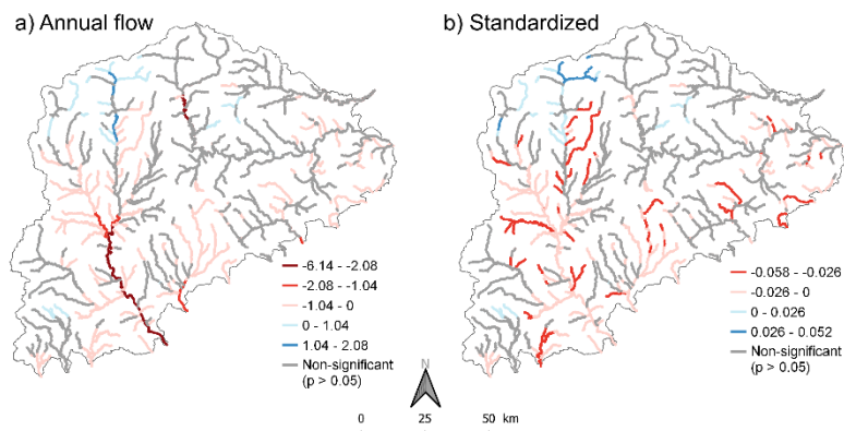
305 Figure 4: Spatial distribution of Sen's slope (a, units \text{hm}^3/\text{year} ) and standardized Sen's slope (b, units \text{year}^{-1} ) for the hydrological indicator total annual flow.
