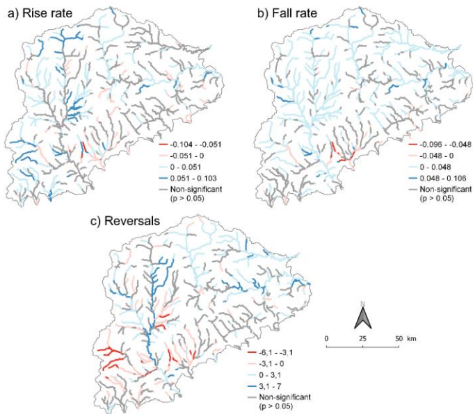
Figure 8: Spatial distribution of Sen's slope for the hydrological indicators rise rate (a), fall rate (b) and number of flow reversals (c). The former's Sen's slopes units are number of reversals/year for the last indicator, while the Sen's slope is they are standardized for the rise and fall rates indicators (units year -1 ).
