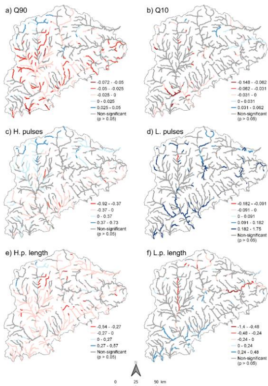
Figure 6: Spatial distribution of Sen's slope for the hydrological indicators Q90 (a), Q10 (b), number of high and low flow pulses (c-d), and their mean duration (e-f). The Sen's slopes for Q90 and Q10 are standardized (a-b, units year -1 ), while the units for the other indicators are number of events/year (c-d) and days/year (e-f).
