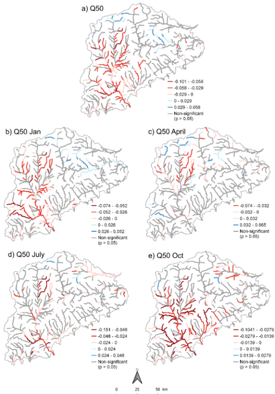
Figure 5: Spatial distribution of standardized Sen's slope (units \text{year}^{-1} ) for the hydrological indicators annual Q50 (a) and Q50 in January (b), in April (c), in July (d), and in October (e), representative of the different seasonal flow patterns.
