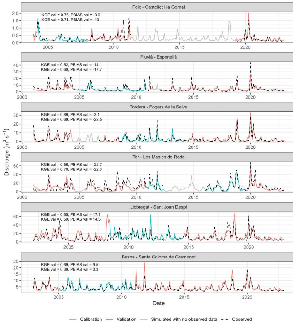
Figure 2: Observed and simulated daily-monthly streamflow for the period 2001-2022 in the six main rivers of SWAT+CRBD. Individual KGE and PBIAS values for both the calibration and validation periods are also shown.
