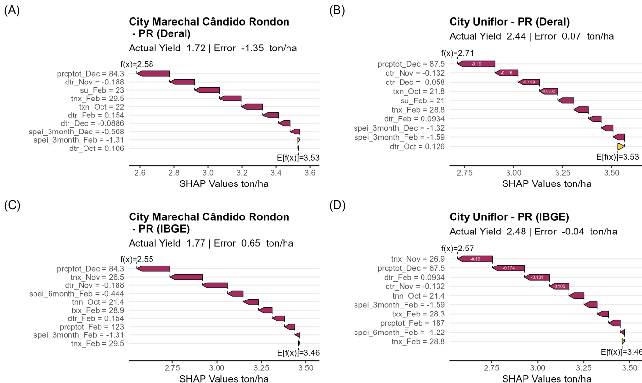
Figure 5. SHAP waterfall plot visualizing the key CID contributions to crop yield losses for the state of Paraná (PR) in 2019, a drought year. Monthly Maximum Value of Daily Minimum Temperature (tnx), Minimum Value of Daily Maximum Temperature (txn), Minimum Value of Daily Minimum (tnn), Maximum Value of Daily Maximum (tnx), Percentage of days when TX > 90th percentile, Standardized Precipitation Evapotranspiration Index (SPEI), Total Precipitation (prcptot), Daily temperature range (DTR)
