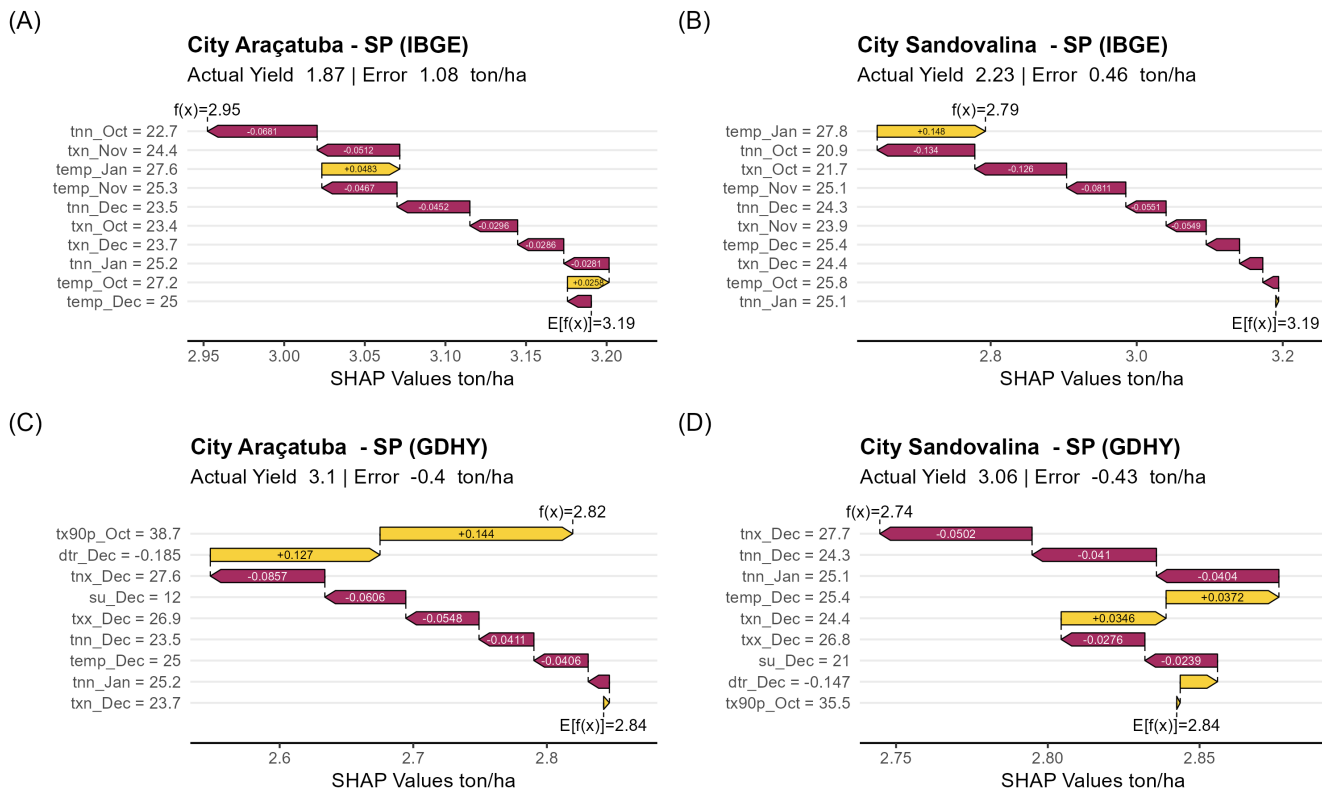
Figure 6. SHAP waterfall plot visualizing the key CID contributions to crop yield losses for the state of São Paulo (SP) in 2015, a drought year. Monthly Maximum Value of Daily Minimum Temperature (tnx), Minimum Value of Daily Maximum Temperature (txn), Minimum Value of Daily Minimum (tnn), Maximum Value of Daily Maximum (txx), Percentage of days when TX > 90th percentile, Standardized Precipitation Evapotranspiration Index (SPEI), Total Precipitation (prctot), Daily temperature range (DTR)
