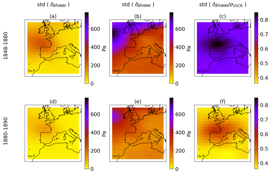
Figure 6. Time-standard deviation of \delta\mu_{\text{HMM}} (a,d), \delta\mu_{\text{HMM}} (b,e) and \delta\mu_{\text{HMM}}/\sigma_{20\text{CR}} (c,f) computed from \delta October to March, for years 1848-1880 (a,b,c) and 1880-1890 (d,e,f). Probabilities p_{\text{HMM}} and p_{\text{HMM}} make use of data from Brest tide gauge.
