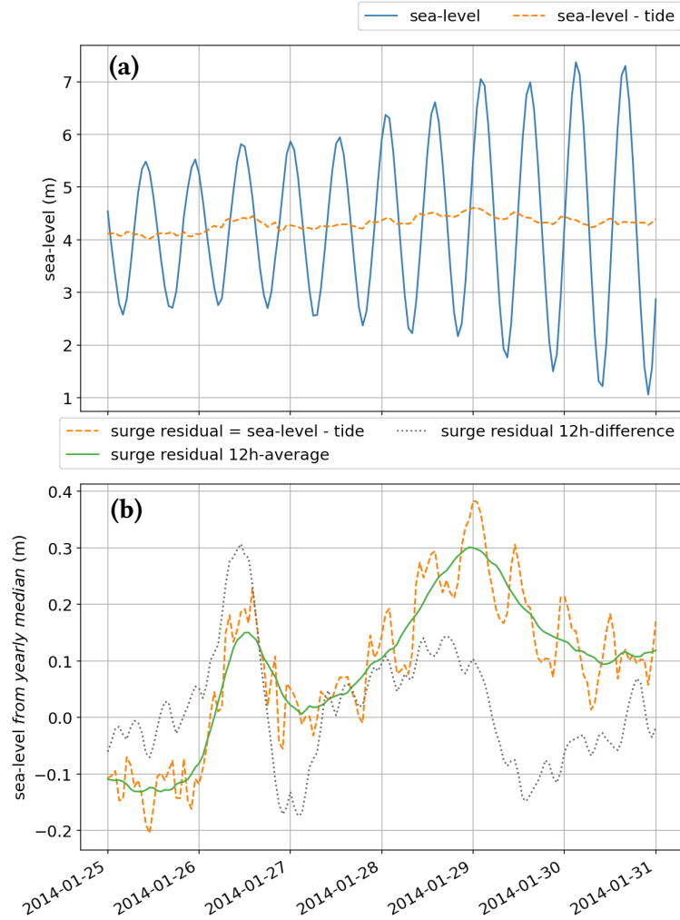
Figure 2. An example output of the different stages of preprocessing of the sea-level signal used in this work. (a) Raw level Sea-level before (full, blue line) and after (dashed, orange line) removing the tidal part of the signal. (b) Sea-level after removing the yearly median value: the Zero-median surge residual h(t) (1h sampling, orange dashed curve), the its centered 12h-average of the surge \bar{h}^{-12h}(t) (green full curve), and the 12h difference between 3h-averages of the surge residual \Delta\bar{h}^{-3h}(t) (gray dotted curve).
