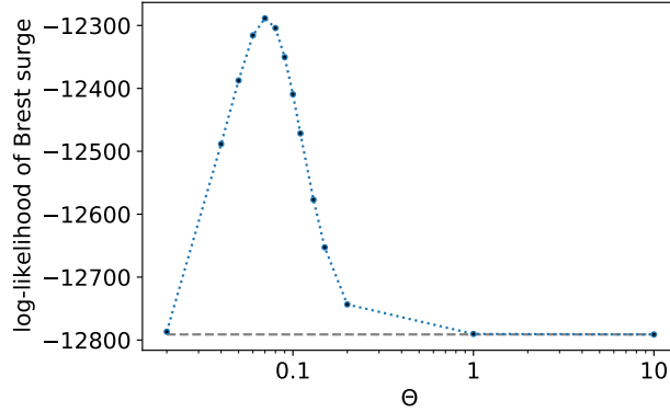
Figure 4. Log-likelihood of Brest surges surge residuals (dotted blue line) as a function of parameter \Theta defined in Eq. (14). For comparison, the log-likelihood of the simple model without Hidden Markov Model ( \Theta \rightarrow +\infty ) is also shown (dashed grey line). The log-likelihood was estimated using data from year 1885 for a first estimation of optimal parameter \Theta . Values of \Theta used for estimation are 0.02, 0.04, 0.05, 0.06, 0.07, 0.08, 0.09, 0.1, 0.11, 0.13, 0.15, 0.2, 1, and 10, with 0.07 giving the largest log-likelihood.
