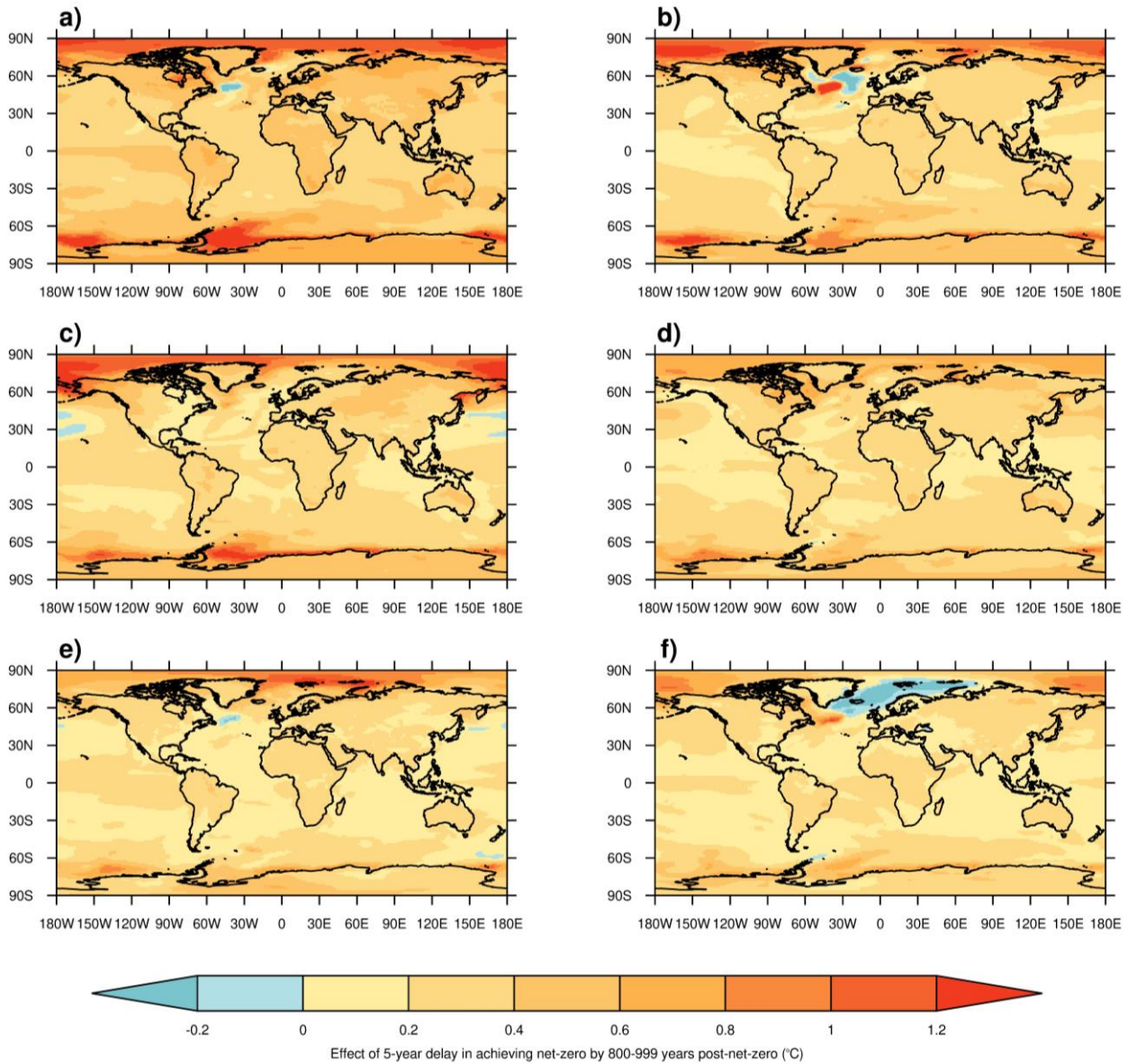
Figure A3. Maps of annual-average temperature differences between net-zero simulations where emissions cessation is delayed five years in years 800-999 post emissions cessation for a) NZ2060-NZ2055, b) NZ2055-NZ2050, c) NZ2050-NZ2045, d) NZ2045-NZ2040, e) NZ2040-NZ2035, and f) NZ2035-NZ2030.
