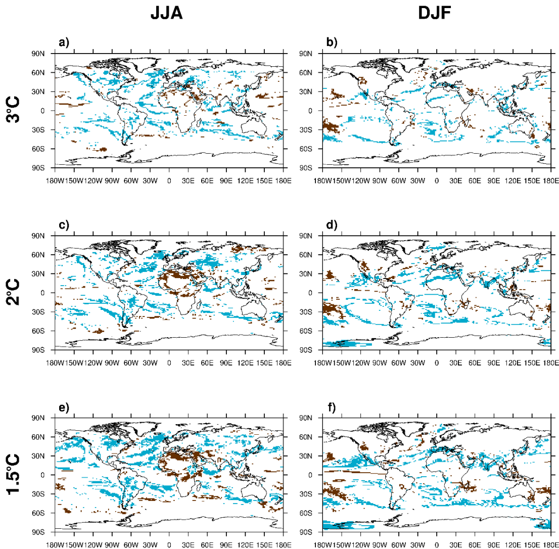
625 Figure A7. Locations of differences in precipitation trends under transient and stabilised climate changes where the difference is large enough for the stabilised climate to be similar to the 1850-1900 baseline period ( p > 0.05 ), for a), b) 3°C, c), d) 2°C and e), f) 1.5°C global warming levels in JJA and DJF respectively. Locations in blue are drier under SSP5-8.5 but are significantly wetter ( p < 0.05 ) by 650-1000 years after emissions cessation at the same global warming level and have experienced a return to 1850-1900 seasonal precipitation variability. Locations in brown are wetter under SSP5-8.5 but are significantly drier ( p < 0.05 ) by 650-1000 years after emissions cessation at the same global warming level and have experienced a return to 1850-1900 seasonal precipitation variability.
