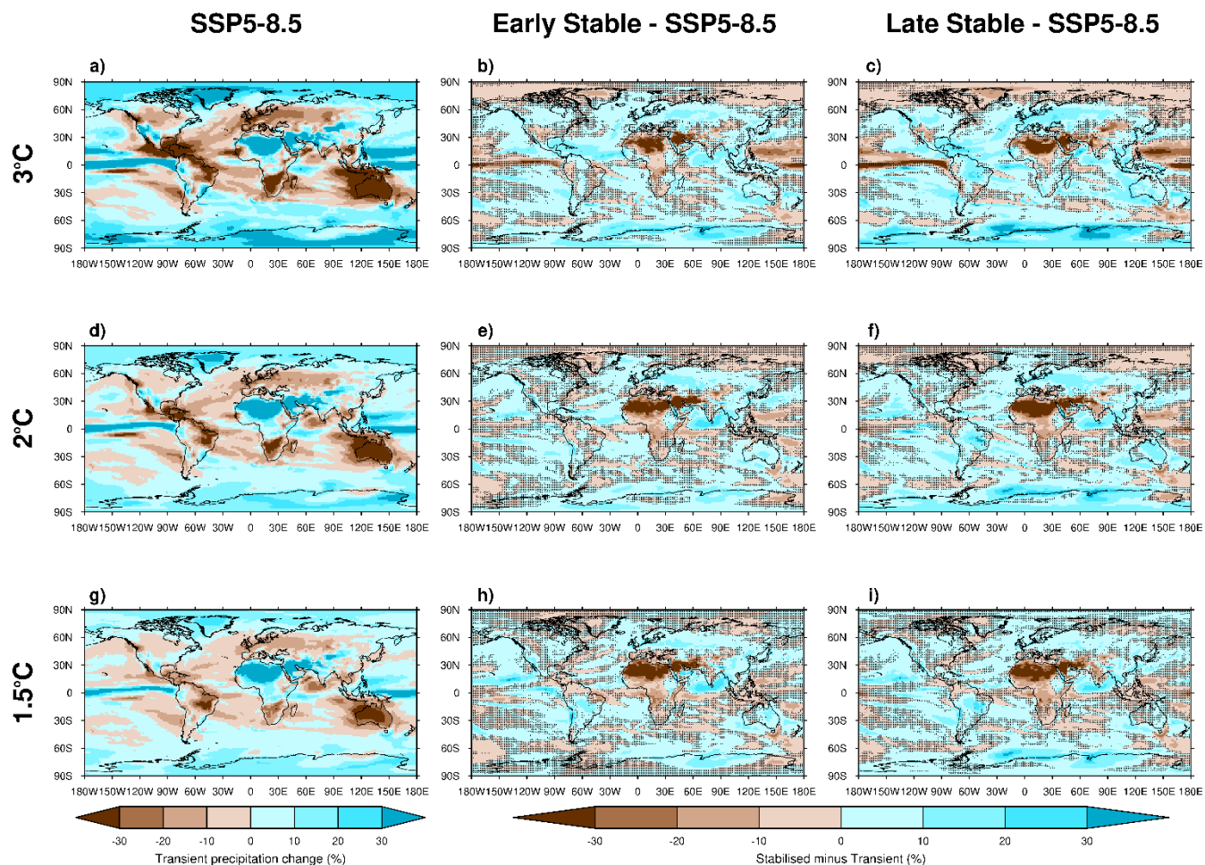
435 Figure 10. Change in boreal summer (JJA) average precipitation at a) 3°C, d) 2°C and g) 1.5°C global warming levels in SSP5-8.5 simulations relative to the 1850-1900 baseline. The difference in JJA average precipitation between global warming levels extracted between 100 and 450 years after emissions cessation and SSP5-8.5 at b) 3°C, e) 2°C and h) 1.5°C global warming levels. The difference in JJA average precipitation between global warming levels extracted between 650 and 1000 years after emissions cessation and SSP5-8.5 at c) 3°C, f) 2°C and i) 1.5°C global warming levels. 440 b), c), e), f), h), i) Stippling shows where distributions are not significantly different at the 5% level using a Kolmogorov- Smirnov test.
