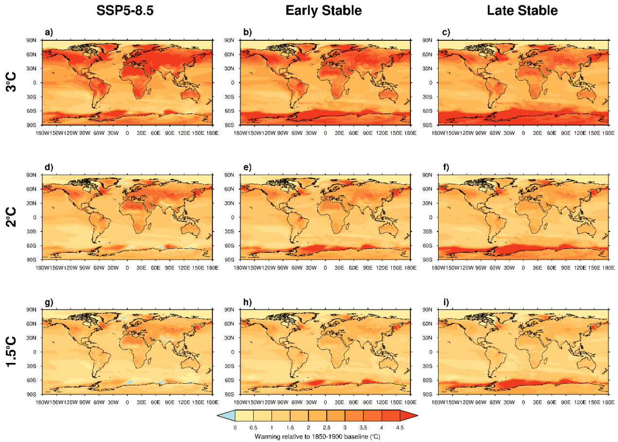
Figure A5. Warming in boreal summer (JJA) average temperatures at a)-c) 3°C, d)-f) 2°C and g)-i) 1.5°C global warming levels in a), d), g) SSP5-8.5 simulations, b), e), h) net-zero simulation warming levels extracted between 100 and 450 years after emissions cessation, and c), f), i) net-zero simulation warming levels extracted between 650 and 1000 years after emissions cessation, relative to the 1850-1900 baseline.
