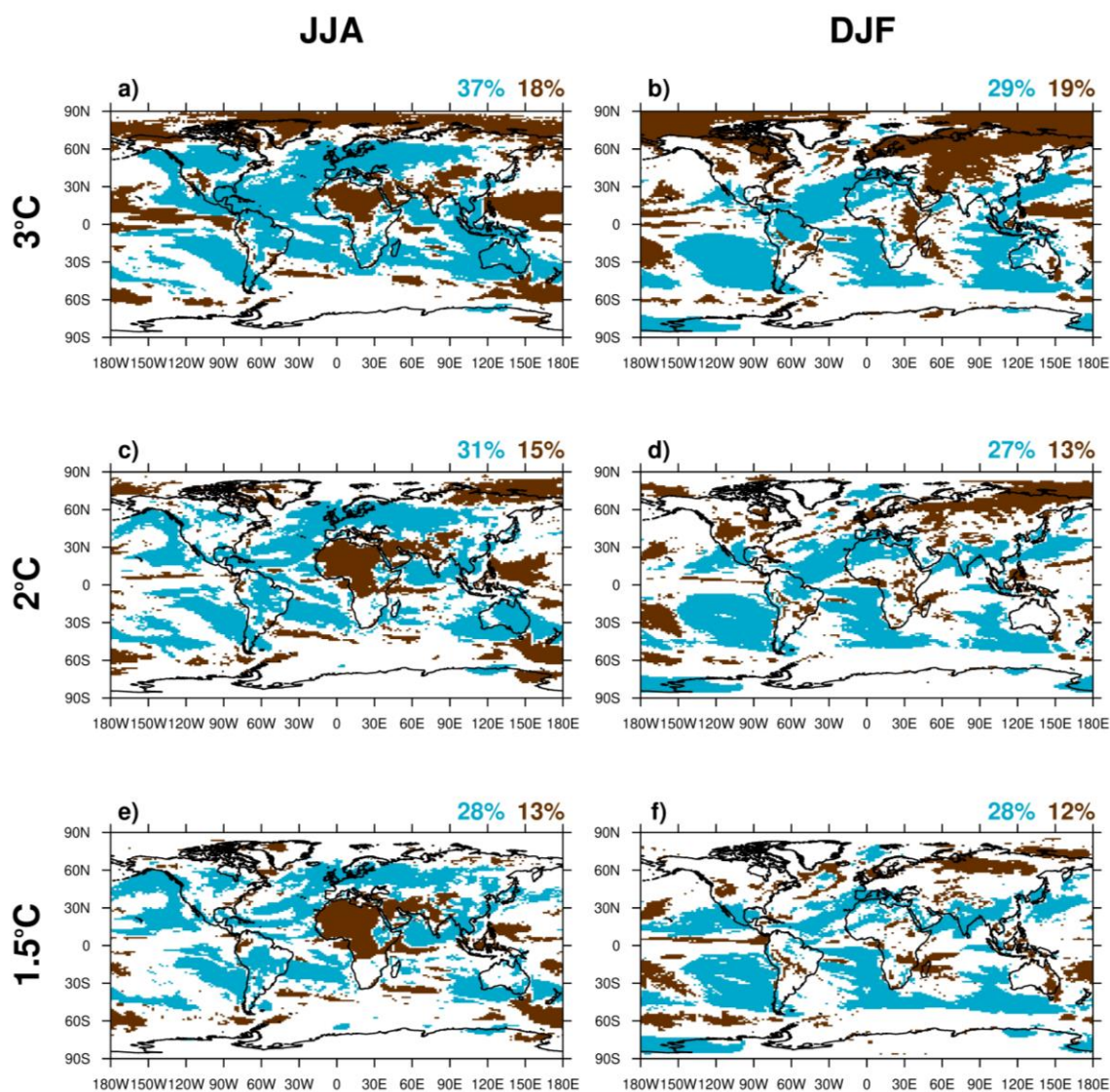
460 Figure 12. Locations of differences in precipitation trends under transient and stabilised climate changes for a), b) 3°C, c), d) 2°C and e), f) 1.5°C global warming levels in JJA and DJF respectively. Locations in blue are drier under SSP5-8.5 but are significantly wetter ( p < 0.05 ) by 650-1000 years after emissions cessation at the same global warming level. Locations in brown are wetter under SSP5-8.5 but are significantly drier ( p < 0.05 ) by 650-1000 years after emissions cessation at the same global warming level. Percentage of the global surface with significant precipitation changes are shown for significant increase under stabilisation relative to SSP5-8.5 (blue) and significant decrease under stabilisation relative to SSP5-8.5 (brown).
