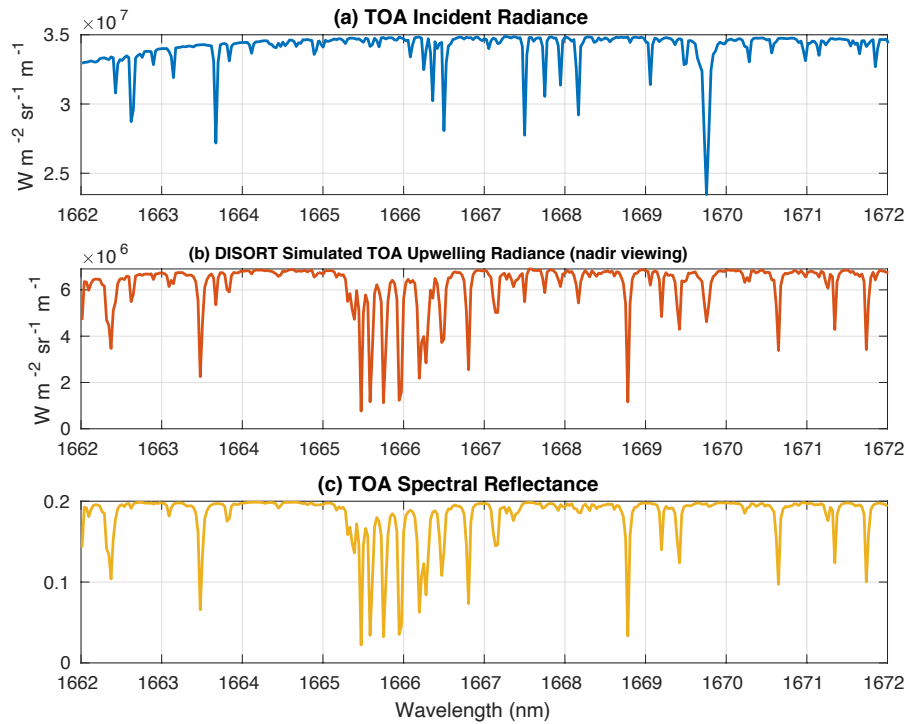
Figure 1. (a) TOA incoming solar radiance; (b) Simulated TOA upward radiance (nadir viewing); (c) Spectral reflectance (nadir viewing). Spectra are simulated with a surface albedo of 0.2 and a solar zenith angle of 60°.
