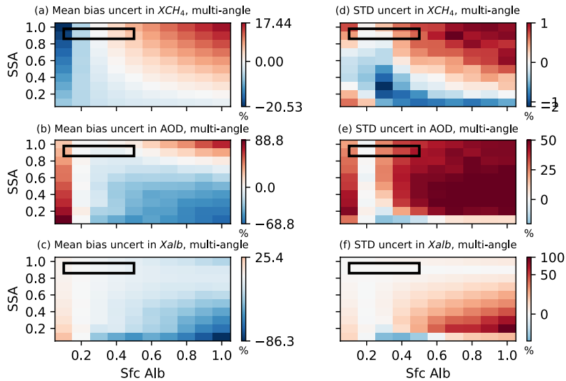
745 Figure 16. Uncertainties induced by surface albedo in mean bias (left column) and standard deviations (STD) (right column) of retrieved \Delta X_{CH_4} , AOD, and X_{alb} , assuming 0.2 surface albedo in retrieval. The simulated truth of \Delta X_{CH_4} and AOD are 0.1 ppm and 0.1, respectively. The scattering angle ranges from 100°-140°. The black box represents the typical values for aerosol optical property and surface albedo ranges (sfc alb \in [0.1, 0.5] and SSA \in [0.86, 0.98]) in the observation.
