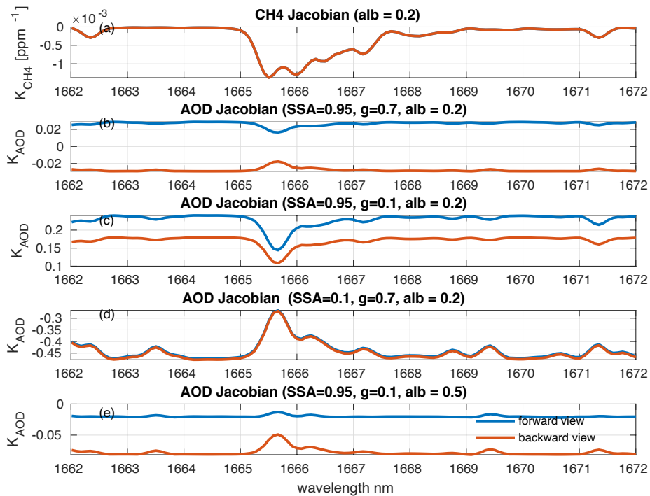
290 Figure 5. Jacobian of TOA reflectance with respect to (a) methane mixing ratio; (b) AOD with an SSA of 0.95, a g of 0.7, and a surface albedo of 0.2; (c) AOD with an SSA of 0.95, a g of 0.1, and a surface albedo of 0.2; (d) AOD with an SSA of 0.1, a g of 0.7, and a surface albedo of 0.2; (e) AOD with a SSA of 0.95, a g of 0.1, and a surface albedo of 0.5. Aerosols are concentrated near the surface and the forward and backward viewing angle settings follow Table 1.
