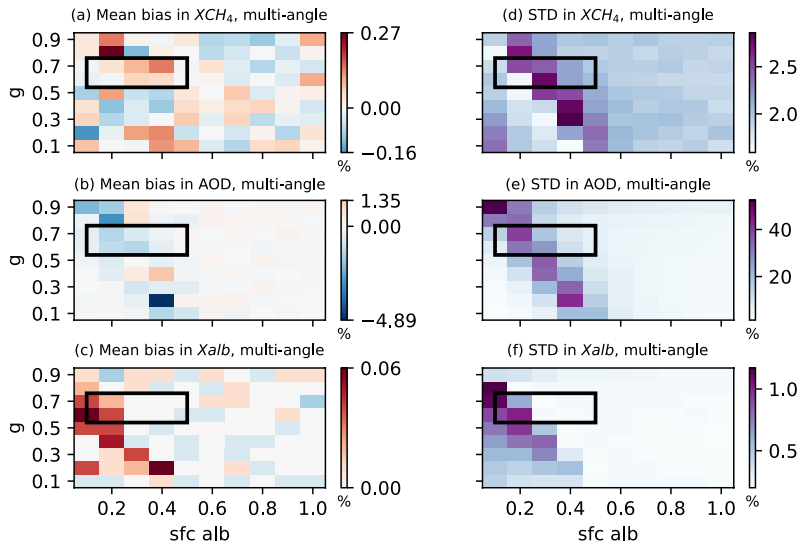
520 Figure 11. Mean bias (left column) and standard deviations (STD) (right column) of retrieved \Delta X_{CH_4} , AOD, and X_{alb} as a function of surface albedo and aerosol g when aerosol SSA is 0.95. The simulated truth of \Delta X_{CH_4} and AOD are 0.1 ppm and 0.1, respectively. The scattering angle ranges from 100^\circ – 140^\circ . The black box represents the typical values for aerosol optical property and surface albedo ranges ( sfc\ alb \in [0.1, 0.5] and g \in [0.54, 0.76] ) in the observation.
