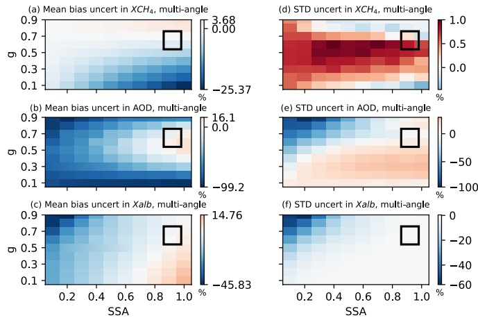
710 Figure 14. Uncertainties induced by aerosol type in mean bias (left column) and standard deviations (STD) (right column) of retrieved \Delta X_{CH_4} , AOD, and X_{alb} , assuming aerosols with an SSA of 0.95 and a g of 0.7 in the retrieval. The simulated truth of \Delta X_{CH_4} , AOD, and X_{alb} are 0.1 ppm, 0.1, and 0.2, respectively. The scattering angle ranges from 100^\circ - 140^\circ . The black box represents the typical values for aerosol optical property ranges (SSA \in [0.86, 0.98] and g \in [0.54, 0.76]) in the observation.
