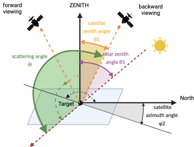
Figure 2. Schematic of a given solar and viewing geometry, as well as corresponding scattering angle for forward and backward viewing modes. Solar zenith angle \theta_1 , satellite zenith angle \theta_2 , and satellite azimuth angles \varphi_2 are indicated by the purple, orange, and black double arrow curves. Scattering angle \Theta is represented by the green double arrow curves. The viewing angles are depicted using solid and dashed double-arrow curves for the backward and forward viewing modes, respectively. In this case, the satellite azimuth angles are 0^\circ and 180^\circ for the backward and forward viewing directions (angles relative to the north-facing vector).
