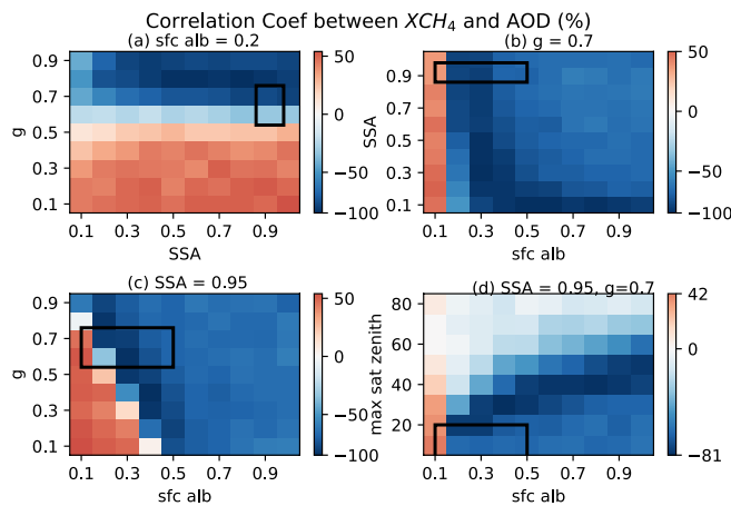
Figure 13. Correlation coefficient (%) between simultaneously retrieved methane enhancement ( \Delta X_{CH_4} ) and aerosol optical depth (AOD) under varying aerosol types and surface albedo values. (a) fix surface albedo as 0.2; (b) fix aerosol g as 0.7; (c) fix aerosol SSA as 0.95. For (a)-(c), the maximum magnitude of the satellite zenith angle is 20°. (d) fix
