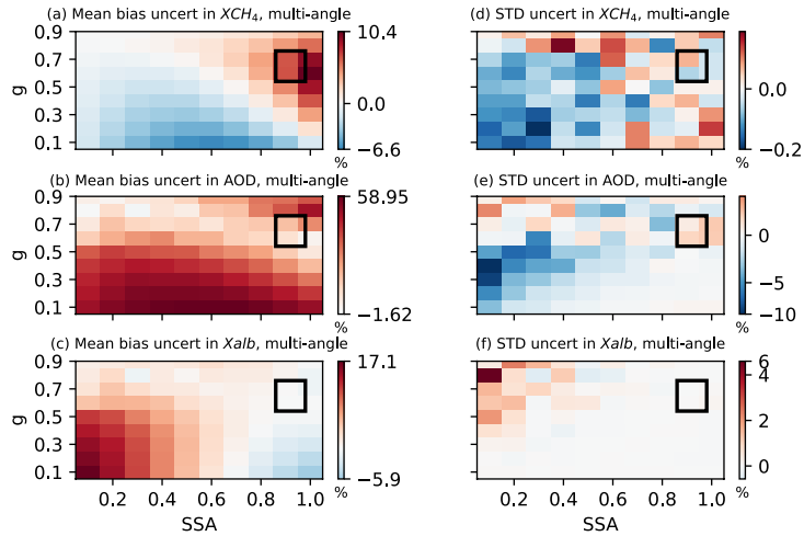
Figure 15. Uncertainties induced by aerosol height distributions in mean bias (left column) and standard deviations (STD) (right column) of retrieved \Delta X_{CH_4} , AOD, and X_{alb} , assuming near-surface aerosols in retrieval. The simulated truth of \Delta X_{CH_4} , AOD, and X_{alb} are 0.1 ppm, 0.1, and 0.2, respectively. The scattering angle ranges from 100°-140°. The black box represents the typical values for aerosol optical property ranges (SSA \in [0.86, 0.98] and g \in [0.54, 0.76]) in the observation.
