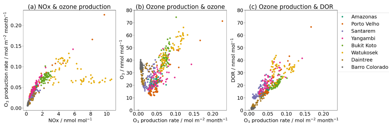
365 Fig. 7: Relationship between monthly mean ozone production rate at the surface at each remote site for (a) surface NO x concentration, (b) surface ozone concentration and (c) the diurnal ozone range (DOR).
