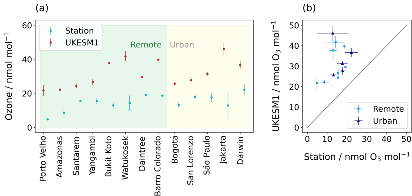
245 Figure 2: Mean annual ozone concentration at each site compared to in the corresponding gridcell of UKESM1 (a) by site and (b) showing the correlation between model and observations. Bars represent 1 standard deviation based on annual means and represent interannual variability. Missing bars in the observations are due to insufficient data.
