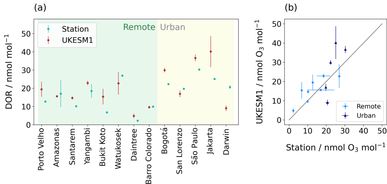
270 Figure 3: Mean Diurnal Ozone Range (DOR) at each site compared to the corresponding gridcell of UKESM1 (a) by site and (b) 275 showing the correlation between model and observations. Bars represent 1 standard deviations using annual means to indicate interannual variability. Missing bars in the observations are due to insufficient data.
