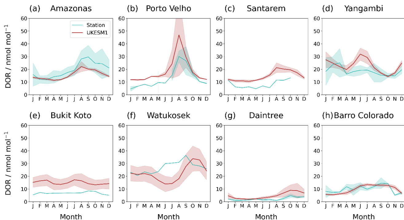
355 Figure 6: Mean monthly Diurnal Ozone Range (DOR) at each site (blue solid line) compared to in the corresponding gridcell of UKESM1 (red solid line). Shading covers 1 standard deviation except at the TOAR I sites (Santarem, Bukit Koto, Watukosek) where diurnal cycle data were only available as a monthly climatology.
