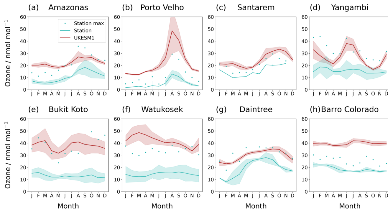
335 Figure 5: Mean monthly ozone concentration at each site (blue solid line) compared to in the corresponding gridcell of UKESM1 (red solid line). Shading covers 1 standard deviation using monthly means to indicate interannual variability. The maximum ozone concentration recorded in each month using daily means is shown for observations (blue circles).
