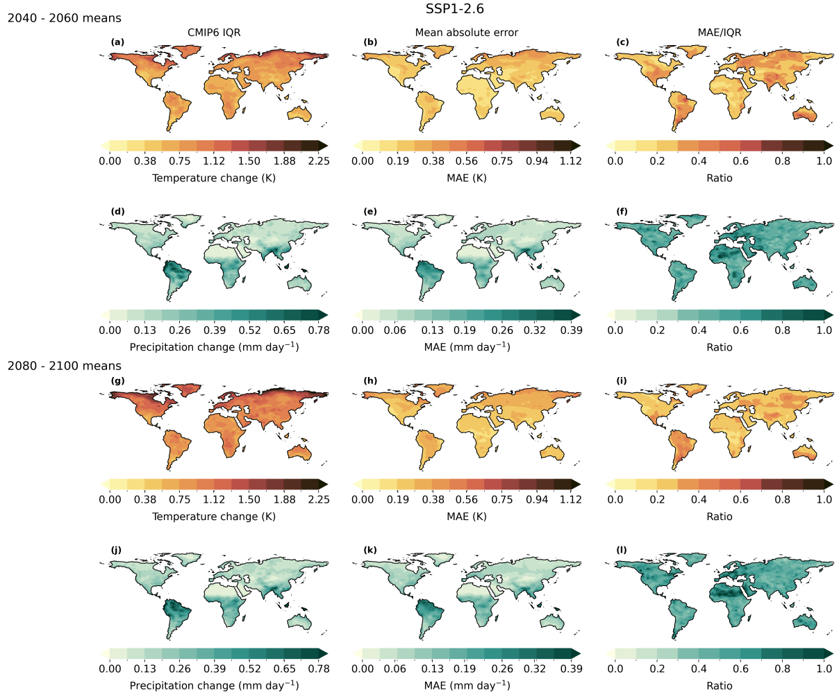
Figure 5. Evaluation of the interquartile range (IQR) of predictions (left column) and of the mean absolute model-to-model error (MAE) for SSP1-2.6 for temperature (a,b,e,f) (a-c, g-i) and precipitation (c,d,g,h) (d-f, j-l). Maps (a-d) (a-f) highlight mid-century predictions, and (e-h) (g-l) show those for the end of century. The middle column shows the MAE and the right hand column shows the ratio of MAE to IQR.
