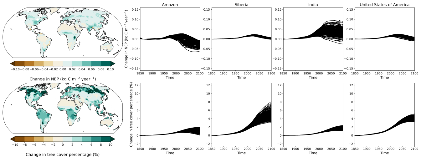
Figure 9. Maps of net ecosystem production (top) and tree fraction (bottom) with timeseries showing the median and uncertainty ranges PRIME output for each ensemble member for each study region: Amazon, Siberia, India and the USA (labelled) for SSP1-2.6 between 1850–2100.
