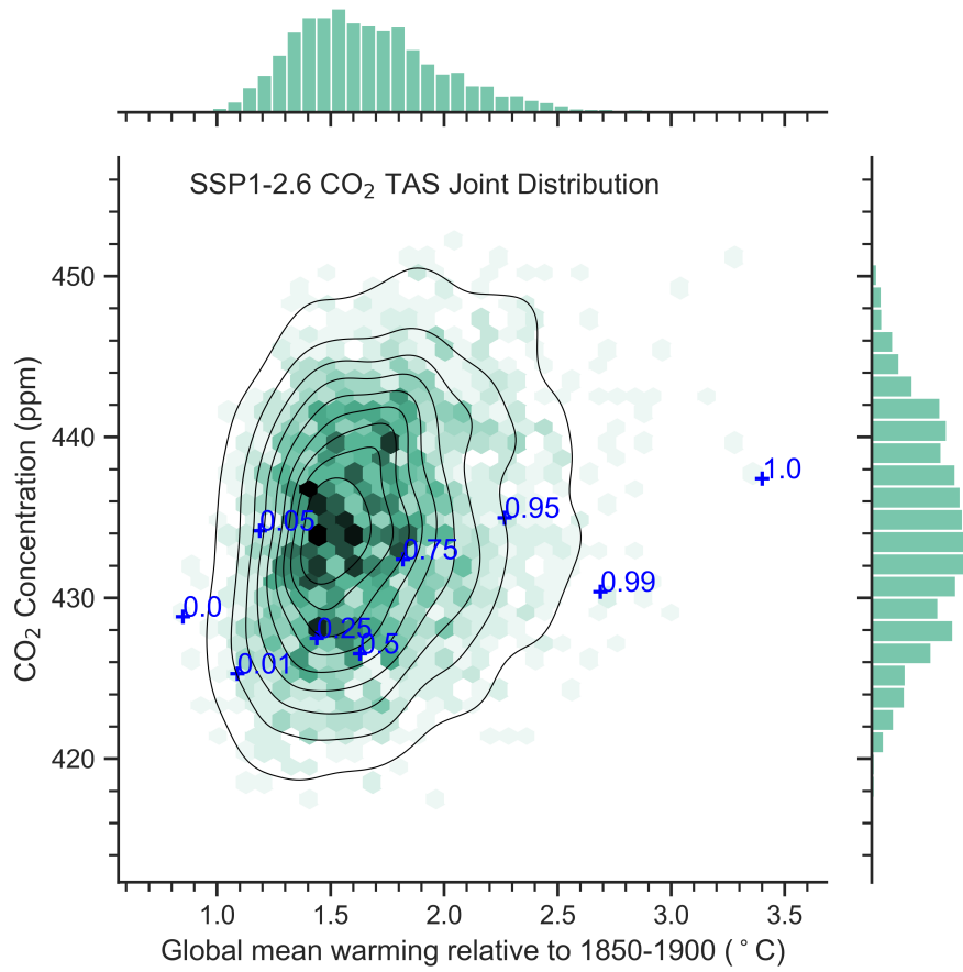
Figure 3. Joint frequency distribution from the FaIR simulations of global temperature rise and CO 2 concentration in 2100 for SSP1-2.6 emissions and the sub-selected percentiles (blue crosses) used to drive the JULES impacts model. Shades of green denote the density of points with individual histograms above and to the right of the main panel. 10% confidence intervals are shown by the contours.
