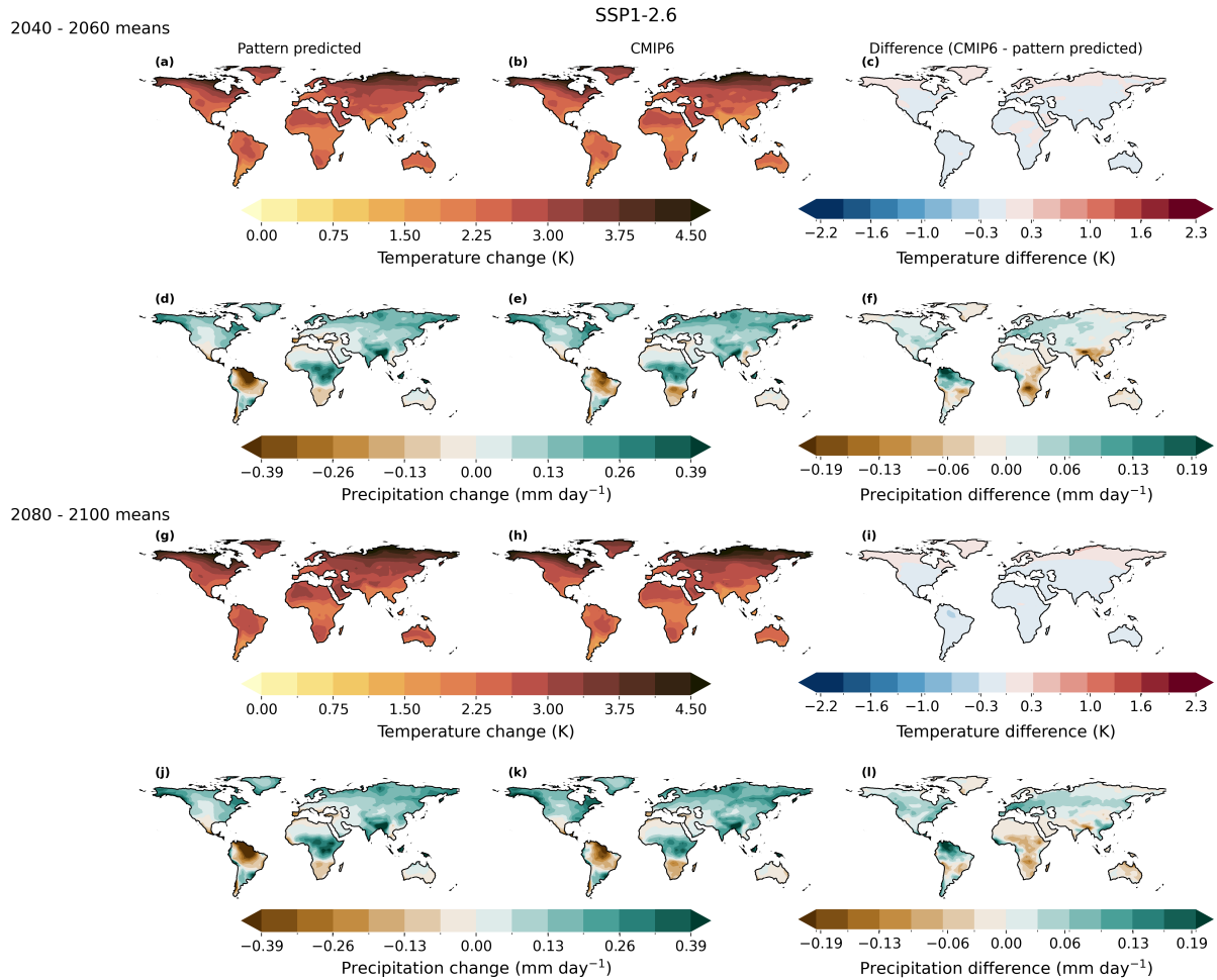
Figure 4. Evaluation of the pattern predicted ensemble means-mean anomalies compared to the CMIP6 ensemble mean anomalies for near-surface air temperature ( a-c, g-i ) and precipitation ( d-f, j-l ) for SSP1-2.6. Maps ( a-f ) highlight mid-century predictions, and ( g-l ) show those for the end of century. The right hand column shows the difference between the predictions (left hand column) and CMIP6 (middle column). The colourbar magnitude for the differences is not the same as that for the anomalies, in order to show that the detail in the prediction error, which is small compared to the change induced by the scenario.
