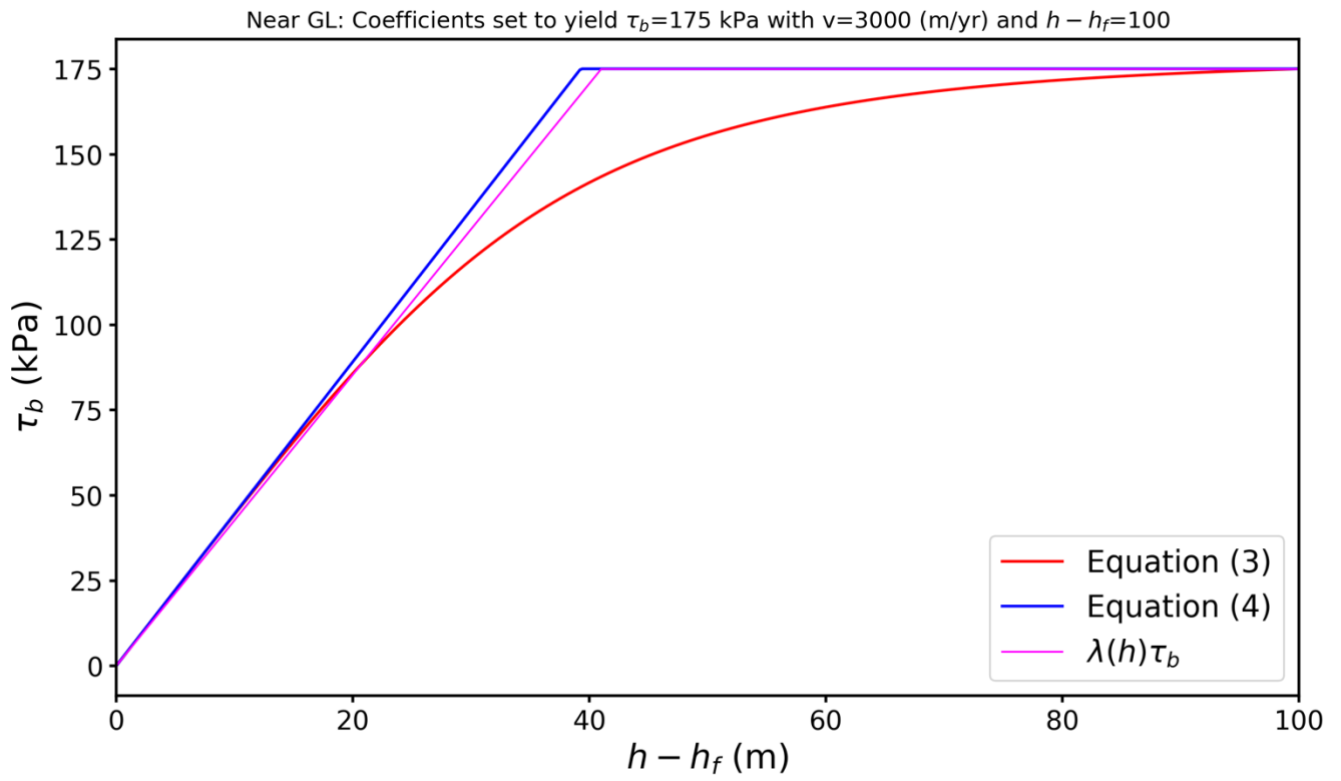
800 Figure 3. Example of the decrease in basal resistance as ice approaches flotation for the different friction laws described in the text.
