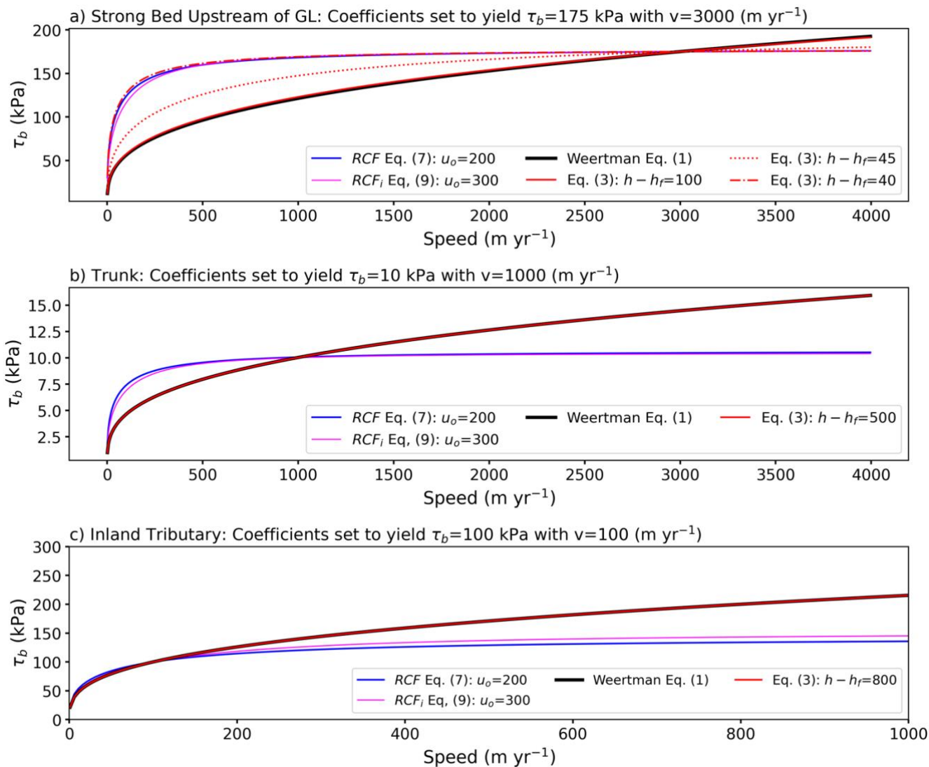
790 Figure 1. Basal shear stress ( \tau_b ) as a function of speed for conditions representative of flow a) for the strong area upstream of the grounding line, b) on the weak main trunk farther inland, and c) slow inland tributary flow. In each case, the sliding coefficients have been selected to produce the same speed basal resistance at a nominal reference speed. For the near-grounding-line case, the transition to full Coulomb friction begins at h - h_f \approx 40 m (red dotted curve) with mixed conditions occurring at h - h_f = 45 (red dot-dashed line).
