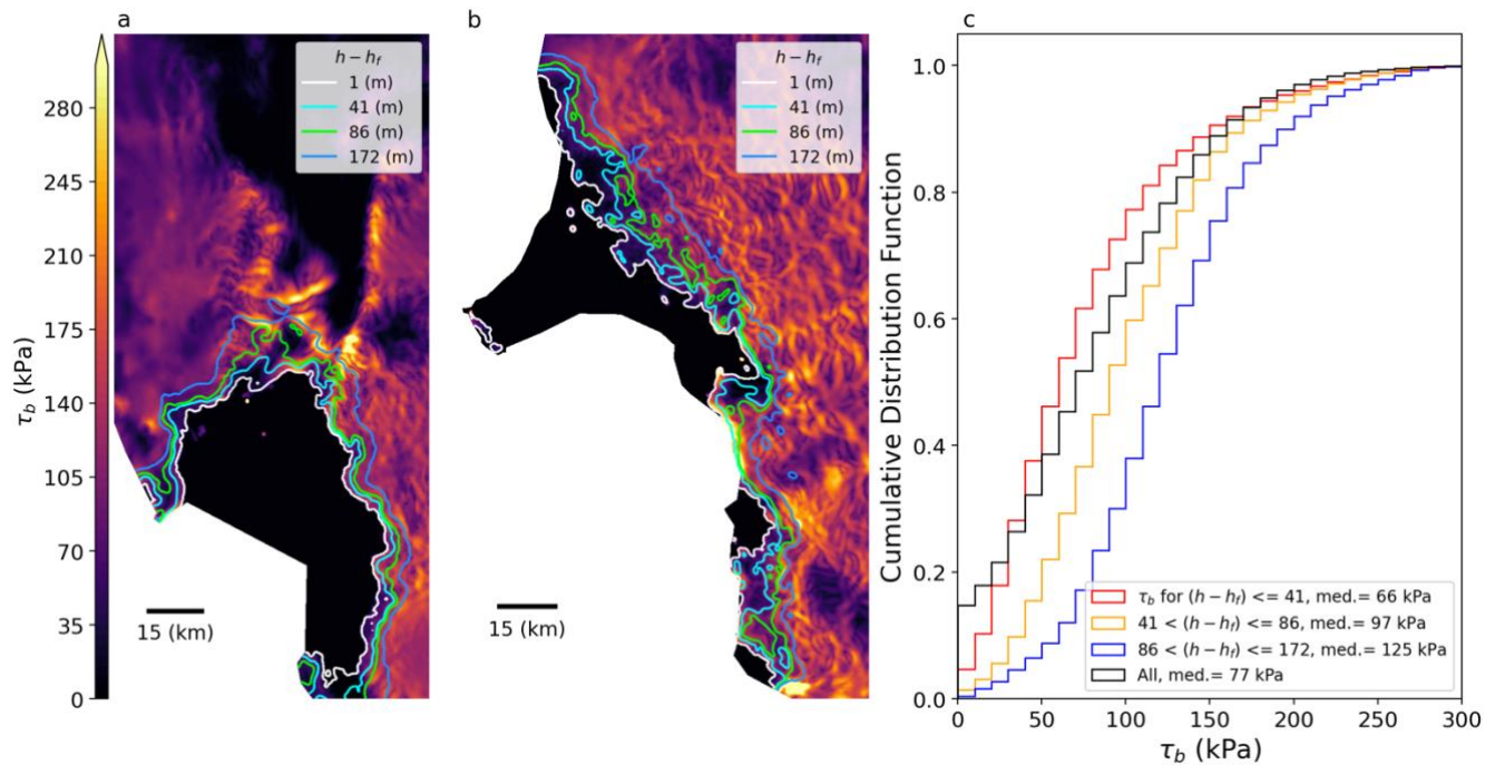
795 Figure 2. Height above flotation ( h - h_f ) contours plotted over inferred basal shear stress ( \tau_b from RCFi inversion) for (a) Pine Island and (b) Thwaites glaciers. (c) Cumulative distribution functions for \tau_b for bands defined by h - h_f . Note the contour values correspond to the value of h_T used in our simulations.
