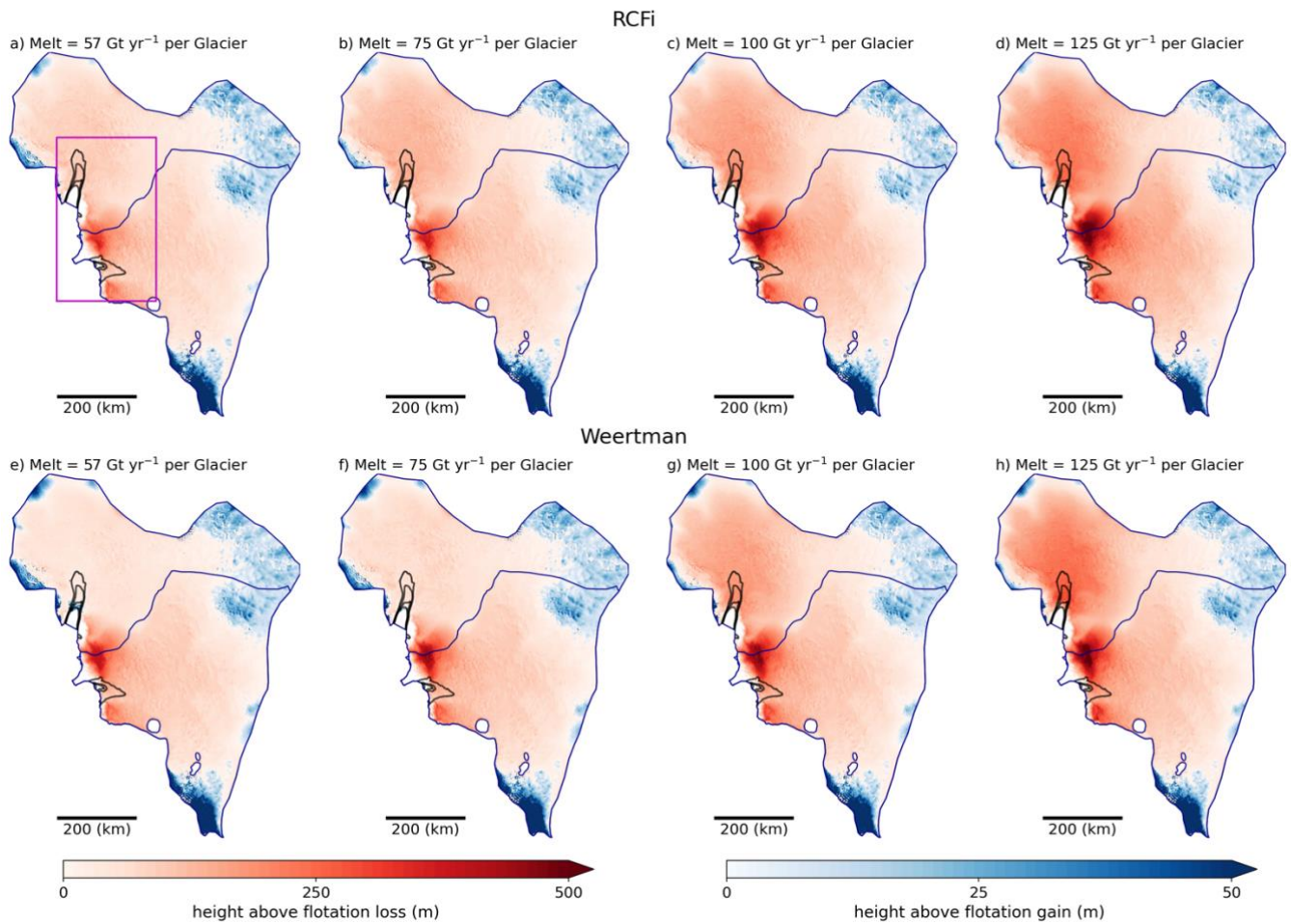
Figure 8. Simulated 200-year VAF loss/gain for h_T=41 m averaged over 30 ensemble members for RCFi with melt applied to each glacier of a) 57 Gt/yr, b) 75 Gt/yr, c) 100 Gt/yr, and d) 125 Gt/yr, and for Weertman sliding with melt of e) 57 Gt/yr, f) 75 Gt/yr, g) 100 Gt/yr, and h) 125 Gt/yr. Speed at 1000 m/yr intervals are shown in black and basin boundaries are shown in blue. The magenta box in panel a indicates the area shown in more detail in Figure 9.
