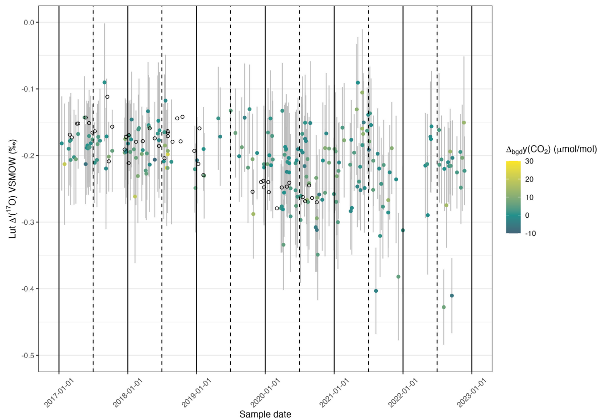
Figure C2. \Delta^{17}\text{O} record of Lutjewad from SICAS flask measurements (filled circles) and DI-IRMS flask measurements of duplicate flasks from the IMAU (open circles). The combined uncertainties of the SICAS measurements are shown as the grey error bars ( \pm 1-\sigma ) and include measurement uncertainty, repeatability and accuracy and introduced uncertainty as a consequence of the calibration method used. The difference in amount fraction between the sample and the background curve, or \Delta\text{CO}_2 , is indicated by the colour of the data points.
