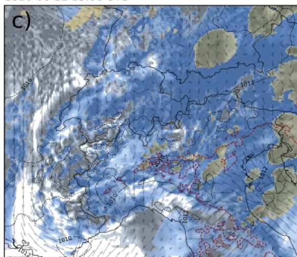
340 Figure 3: Analysis of (a) - (c) cloud cover (cloud fraction from 0 to 1) at low atmospheric levels (L), mid-levels (M), and high levels (H) as well as (total column) precipitable water (red dashed contour lines at 25 kg/m 2 ), sea level pressure (smoothed dashed lines; hPa), and wind (grey vectors, every 8th in each direction is shown) (d) as in Figure 2c. Simulations are with WRF NODA domain 03 for instances in time indicated on top of each panel.
