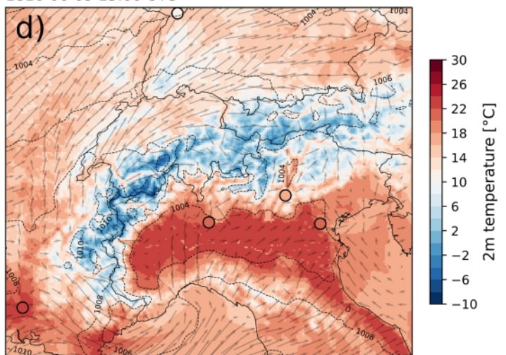
340 Figure 3: Analysis of (a) - (c) cloud cover (cloud fraction from 0 to 1) at low atmospheric levels (L), mid-levels (M), and high levels (H) as well as (total column) precipitable water (red dashed contour lines at 25 kg/m 2 ), sea level pressure (smoothed dashed lines; hPa), and wind (grey vectors, every 8th in each direction is shown) (d) as in Figure 2c. Simulations are with WRF NODA domain 03 for instances in time indicated on top of each panel.
