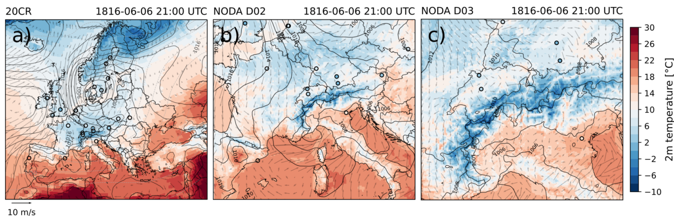
310 Figure 2: Analysis of (a) - (c) temperature at 2 meters above ground (shade: degrees Celsius), 10-meter wind (grey vectors; reference vector approx. 10 \text{ ms}^{-1} ), mean sea level pressure (black contours; hPa) and geopotential height at 500 hPa (light grey dashed contours, meters) over Europe and the Alps on 6 June 1816 21:00 as calculated from 20CR in (a) and the WRF domains 02 (b) and 03 (c). Station observations of temperature are indicated as filled circles.
