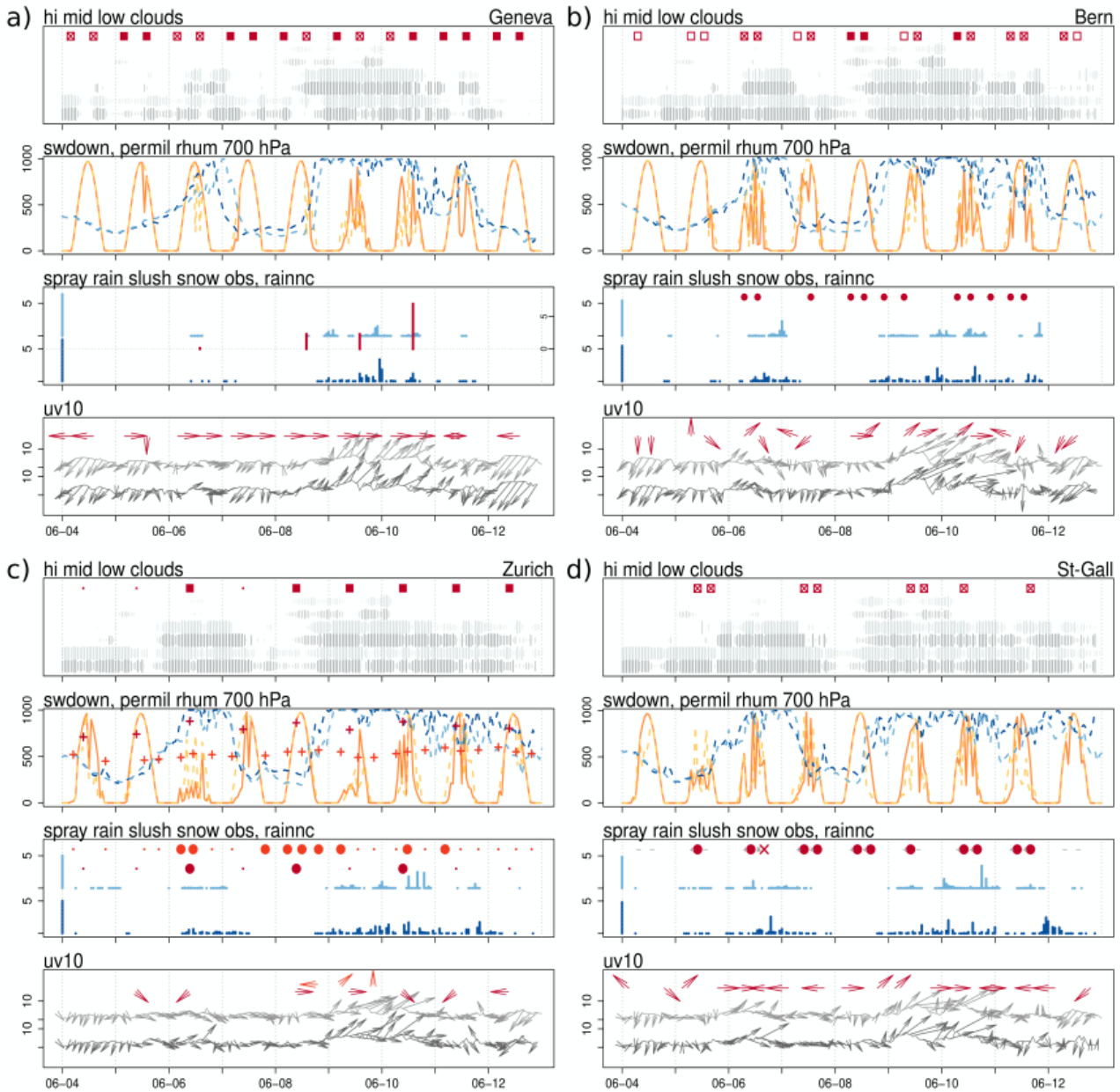
Figure 5: Metograms of station observations and measurements (red colors) for a) Geneva b) Bern c) Zurich and d) St. Gall with WRF NODA (lighter colors, grey, blue, orange) and DA (darker colors) simulations output for the nearest grid point, for the period between 4 and 12 June 1816 (x-axis). Top panels show observed cloud cover (red squares from ‘bright’ with no fill to ‘mixed’ with cross and ‘covered’ with fill) vs. simulated low, mid- and upper level cloud fraction (larger bars indicate more cloudiness). Second row panels show simulations of downward short wave flux at ground surface (orange lines; W/m 2 ) and relative humidity at 700 hPa (dashed blue line; permil). Red crosses (dark for observer Escher, light for Feer) indicate the relative humidity measurements on the ground for Zurich. Third row panels show thrice-daily observations of precipitation (red dots; red vertical bars for Geneva measurements in mm; darker red dots for Zurich stand for observer Escher, lighter for Feer; red cross for ‘rain and snow’ added for St. Gall on 6 June 1816) vs. simulated precipitation (blue vertical bars, mm). Bottom panels show observations of wind direction (red vectors at unit length; north is up) vs. simulated wind direction (grey wind vectors; north is up) and velocity (black line and vector length; m/s at 10 m above ground).
