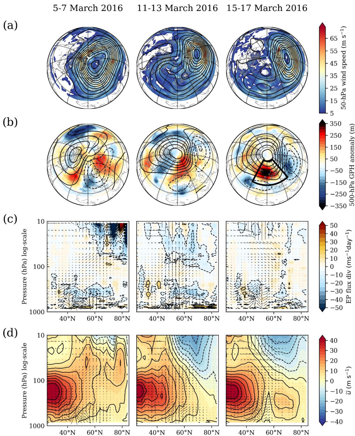
595 Figure A9: Same as for Fig. A1, but for the 2016 SSW. The three-day averaged parameters are shown for the three dates: during the SPV displacement (left), during the split (center) and after the split (right). Black box indicates defined Euro-Atlantic blocking region.
