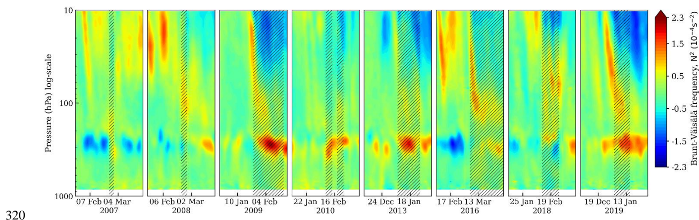
Figure 7: Time-height evolution of the anomalous static stability or the Brunt Väisälä frequency, N^2 , (75-90° N) within a +/- 30 day timeframe relative to each of the SSW events from 2007 to 2019. Hatched regions indicate dates when the zonal-mean zonal wind at 60° N and 10 hPa is negative.
