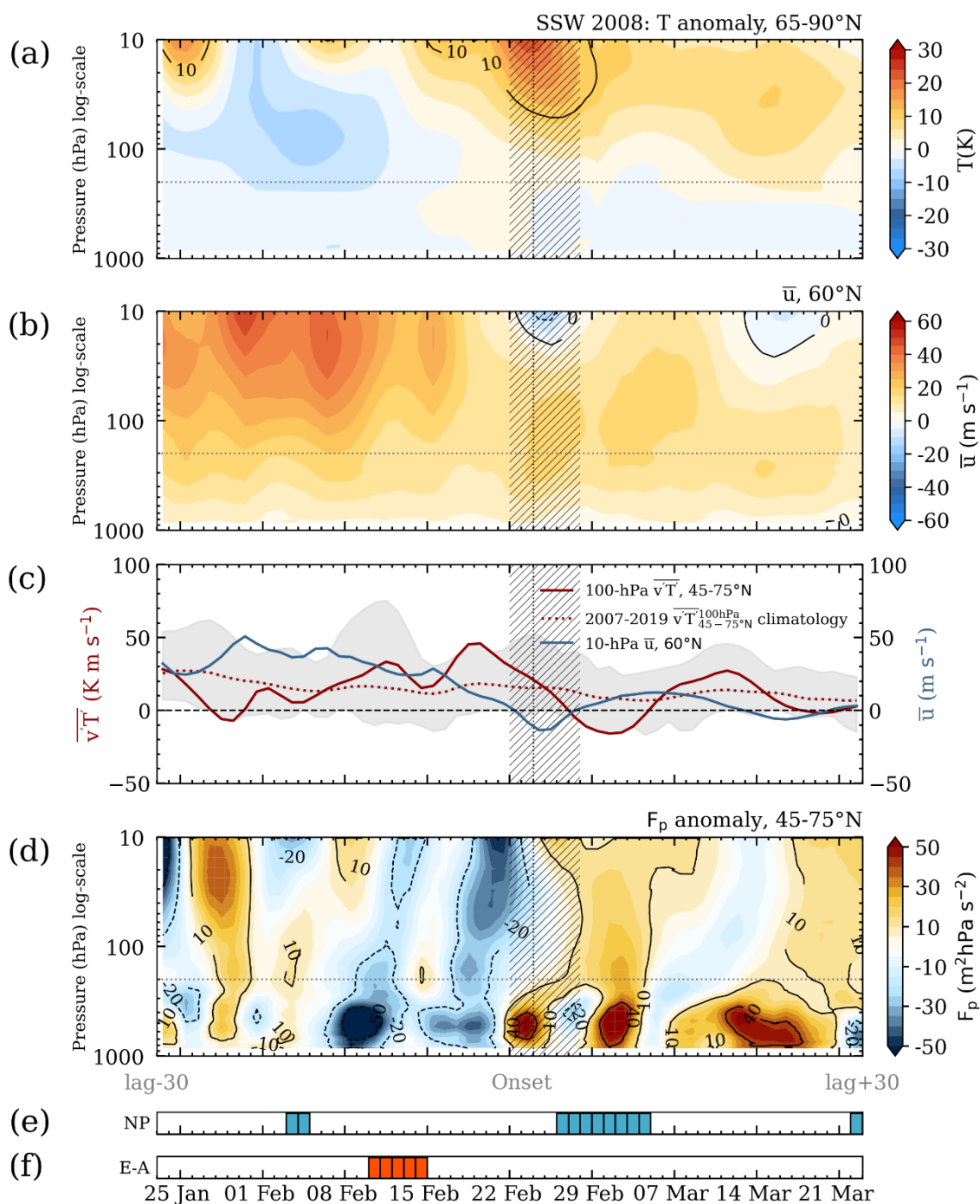
180 Figure 3: Time-height evolution of (a) area-weighted temperature anomaly averaged over 65-90° N, (b) zonal wind at 60° N, (c) 100 hPa eddy meridional heat flux averaged over 45-75° N (red solid line), its daily climatology (red dotted line) and zonal-mean zonal wind at 60° N and 10 hPa (blue solid line). Grey shading covers the region between daily minimum and maximum of the heat flux for the period 2007-
