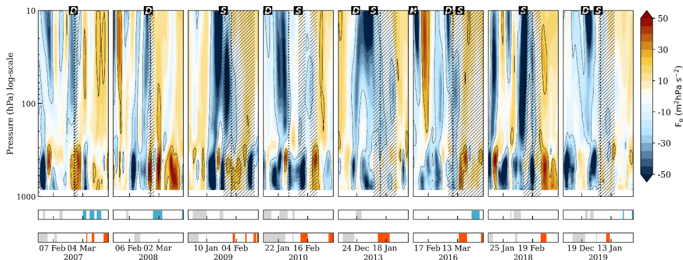
Figure 6: Time-height evolution of the anomaly of the vertical component of the Eliassen–Palm flux ( 45\text{--}75^\circ\text{ N} ) within a \pm 30 day timeframe relative to each of the SSW events from 2007 to 2019. Hatched regions indicate dates when the zonal-mean zonal wind at 60^\circ\text{ N} and 10 hPa is negative, and the vertical dotted lines indicate the start of SSW recovery phase. Letters D and S indicate the approximate start of the SPV displacement and split, respectively. Letter M indicates the minor SSW event. The lower panels show the blocking index for the North Pacific (blue) and Euro-Atlantic region (orange). The blocking events before the SSWs are greyed out.
