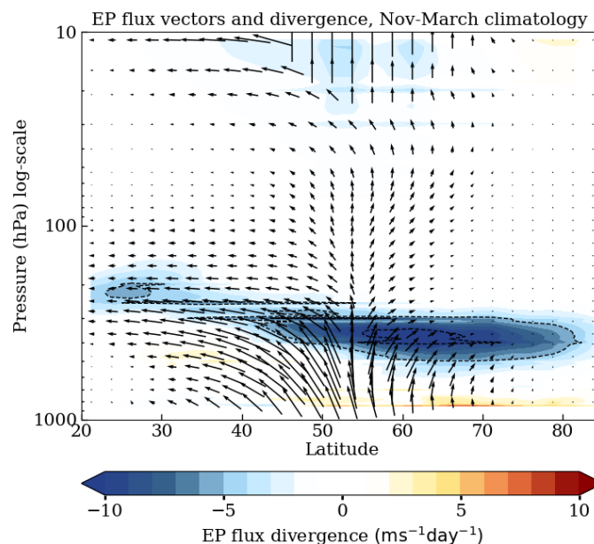
125 Figure 1: Climatological Eliassen–Palm flux vectors and divergence (shading) for November to March from 2006 to 2019. The vectors are plotted for every 5 th pressure level.
