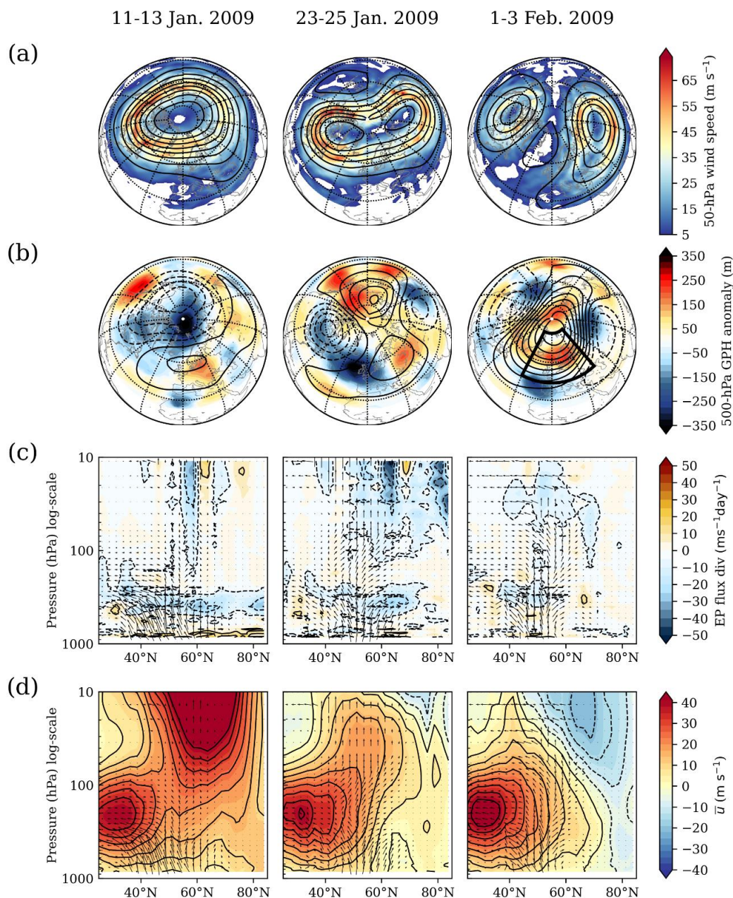
Figure A3: Same as for Fig. A1, but for the 2009 SSW. The three-day averaged parameters are shown for the three dates: before the SPV split (left), during the split (center) and after the split (right). The black box indicates the selected Euro-Atlantic blocking region.
