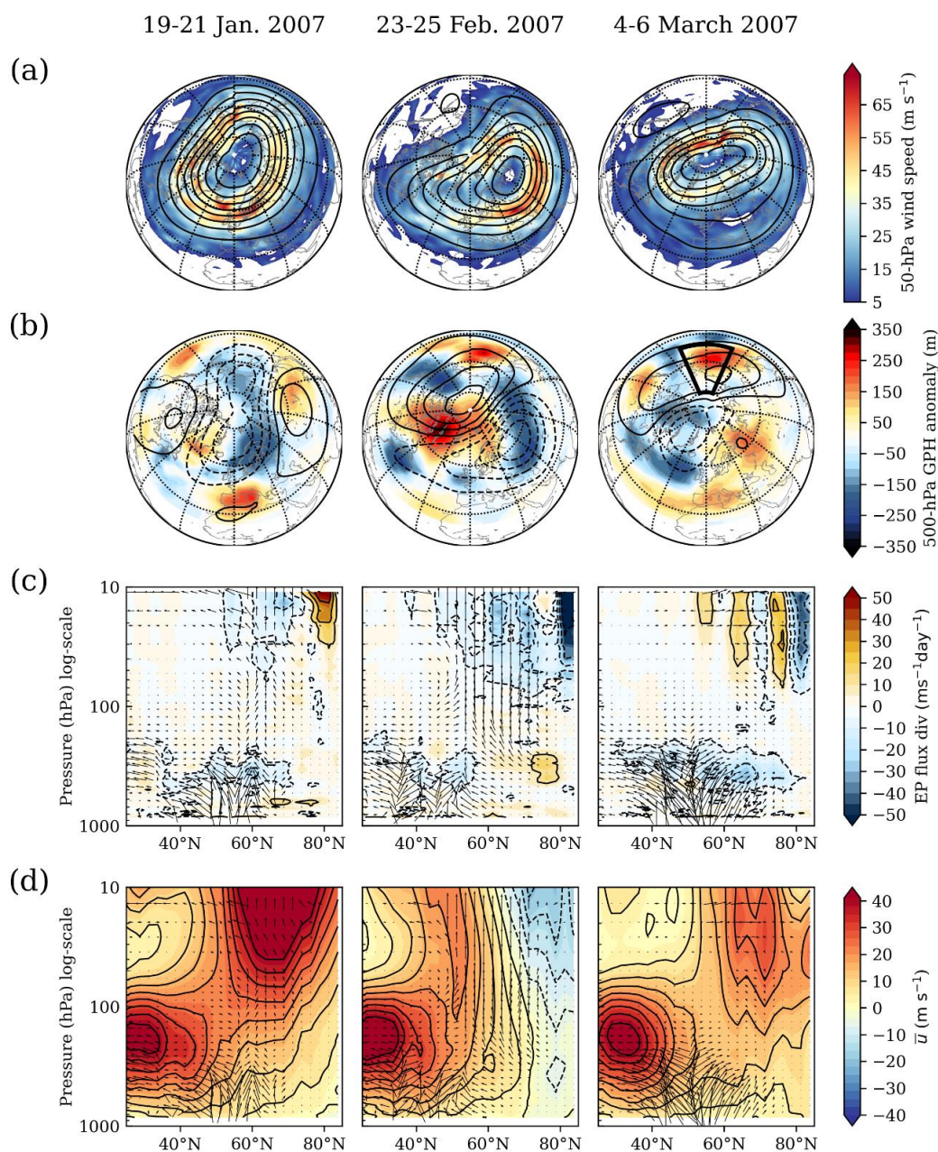
555 Figure A1: Evolution of the SSW 2007 shown for the three dates: before the SPV displacement (left), during its displacement (center) and during its recovery (right). (a) 50 hPa wind speed (shading) and 50 hPa geopotential height (contours). (b) 500 hPa geopotential height anomaly (shading) and 50 hPa geopotential height anomaly (contours). The black box indicates the selected North Pacific blocking region. (c) Meridional cross-sections of Eliassen–Palm flux vectors and divergence (shading). (d) Meridional cross-sections of Eliassen–Palm flux vectors and zonal wind (shading). The vectors plotted for every 5th pressure level.
