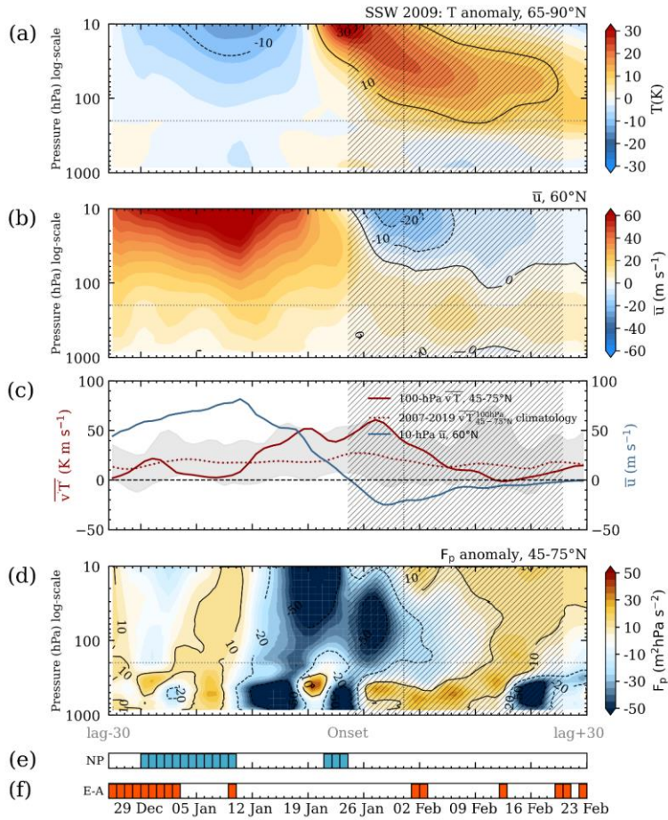
670 Figure A4: Same as Fig. A2, but for the 2009 SSW. The time interval is shown for +/- 30 days from the central date (24 January).
