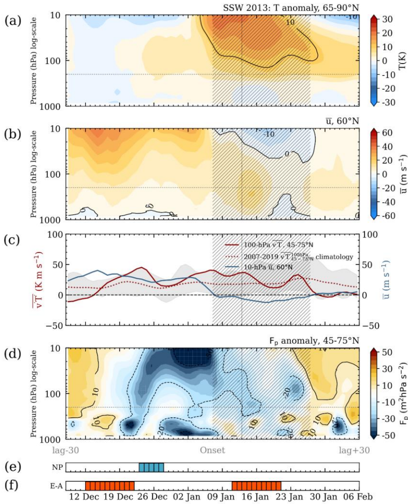
Figure A8: Same as for Fig. A2, but for the 2013 SSW. The time interval is shown for \pm 30 days from the central date (7 January).
