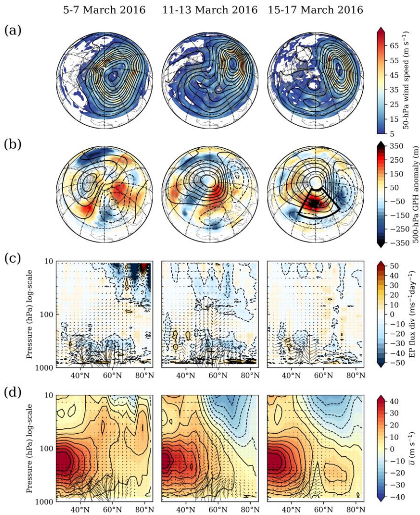
690 Figure A9: Same as for Fig. A1, but for the 2016 SSW. The three-day averaged parameters are shown for the three dates: during the SPV displacement (left), during the split (center) and after the split (right). Black box indicates defined Euro-Atlantic blocking region.
