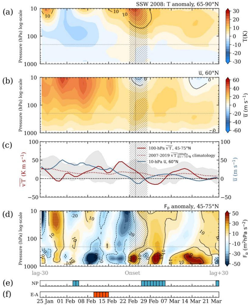
220 Figure 3: Time-height evolution of (a) area-weighted temperature anomaly averaged over 65-90° N, (b) zonal wind at 60° N, (c) 100 hPa eddy meridional heat flux averaged over 45-75° N (red solid line), its daily climatology (red dotted line) and zonal-mean zonal wind at 60° N and 10 225 hPa (blue solid line). Grey shading covers the region between daily minimum and maximum of the heat flux for the period 2007-2019. Time- height evolution of (d) anomaly of vertical component of Eliassen–Palm flux averaged over 45-75° N, (e) blocking index for the North Pacific region, (f) blocking index for the Euro-Atlantic region. Hatched region indicates dates when the zonal-mean zonal wind at 60° N and 10 hPa is 230 negative, and the vertical dotted line indicates the day, when the polar (80-90° N) temperature anomaly reaches its maximum, i.e., the start of SSW recovery phase. The dotted horizontal line indicates 200 hPa (an approximate level of extratropical tropopause). The time interval is shown for +/- 30 days from the central date (22 February) of the 2008 SSW.
