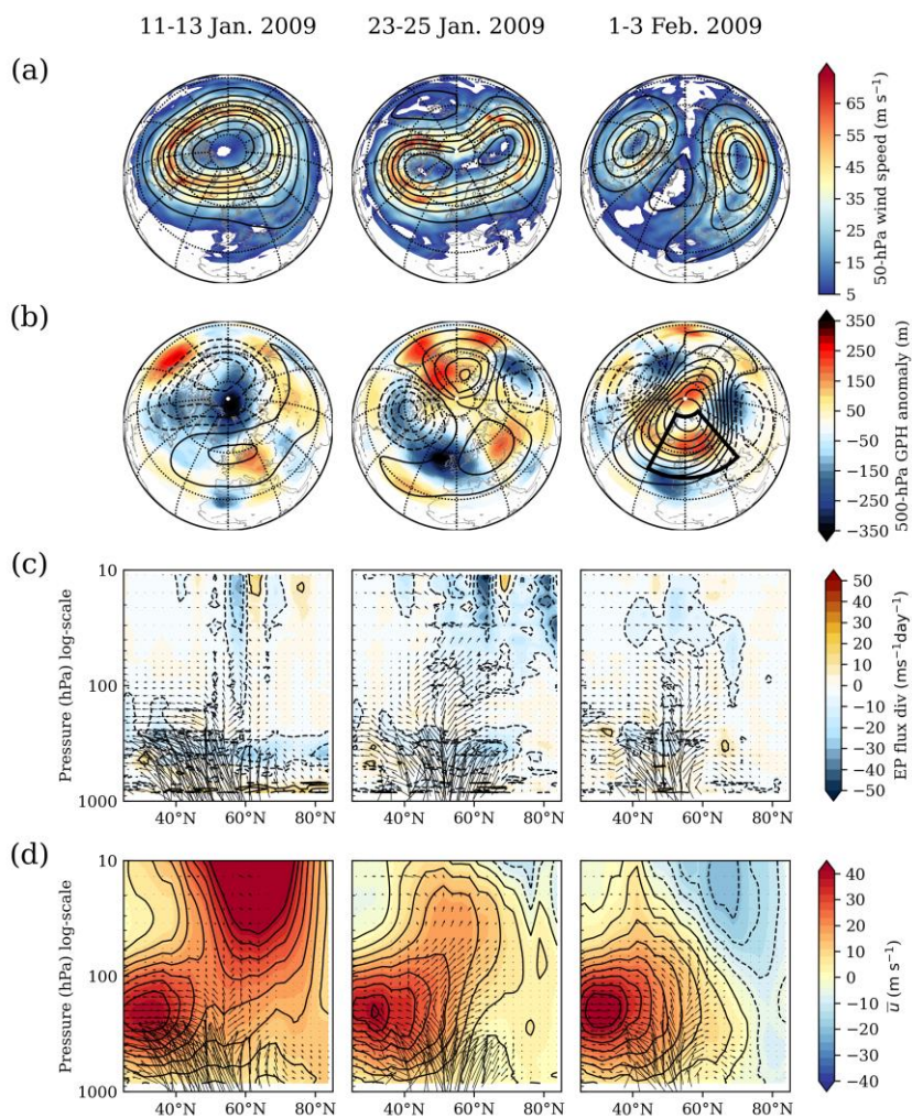
665 Figure A3: Same as for Fig. A1, but for the 2009 SSW. The three-day averaged parameters are shown for the three dates: before the SPV split (left), during the split (center) and after the split (right). The black box indicates the selected Euro-Atlantic blocking region.
