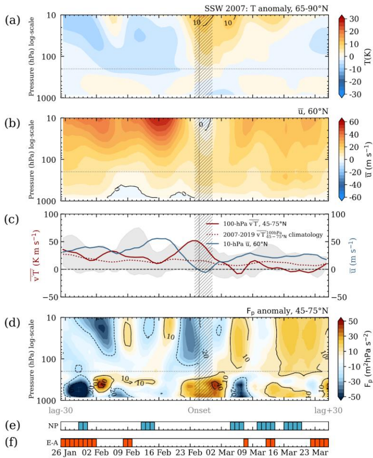
655 Figure A2: Time-height evolution of (a) area-weighted temperature anomaly averaged over 65-90° N, (b) zonal wind at 60° N, (c) 100 hPa eddy meridional heat flux averaged over 45-75° N (red solid line), its daily climatology (red dotted line) and zonal-mean zonal wind at 60° N and 10 660 hPa (blue solid line). Grey shading covers the region between daily minimum and maximum of the heat flux for the period 2007-2019. Time- height evolution of (d) anomaly of vertical component of Eliassen-Palm flux averaged over 45-75° N, (e) blocking index for the North Pacific region, (f) blocking index for the Euro-Atlantic region. Hatched region indicates dates when the zonal-mean zonal wind at 60° N and 10 hPa is negative, and the vertical dotted line indicates the day, when the polar (80-90° N) temperature anomaly reaches its maximum, i.e., the start of SSW recovery phase. The dotted horizontal line indicates 200 hPa (an approximate level of extratropical tropopause). The time interval is shown for +/- 30 days from the central date (24 February) of the 2007 SSW.
