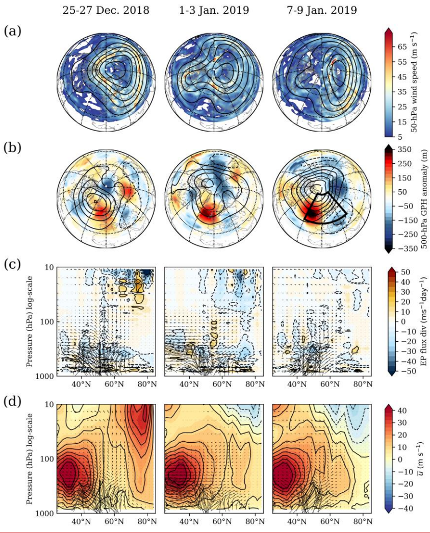
300 Figure 4: Same as for Fig. 2, but for the 2019 SSW. The three-day averaged parameters are shown for the three dates: during the SPV displacement (left), during the split (center) and after the SPV split (right). The black box indicates the selected Euro-Atlantic blocking region.
