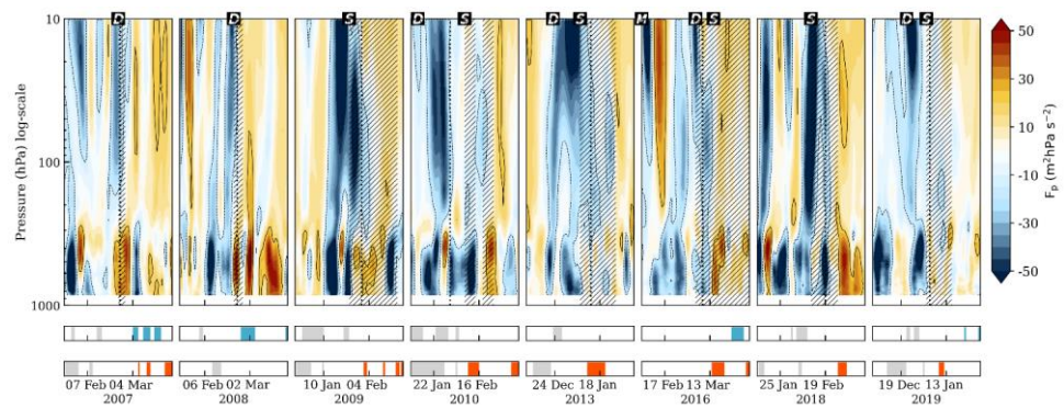
340 Figure 6: Time-height evolution of the anomaly of the vertical component of the Eliassen–Palm flux (45-75° N) within a +/- 30 day timeframe relative to each of the SSW events from 2007 to 2019. Hatched regions indicate dates when the zonal-mean zonal wind at 60° N and 10 hPa is negative, and the vertical dotted lines indicate the start of SSW recovery phase. Letters D and S indicate the approximate start of the SPV displacement and split, respectively. Letter M indicates the minor SSW event. The lower panels show the blocking index for the North Pacific (blue) and Euro-Atlantic region (orange). The blocking events before the SSWs are greyed out.
