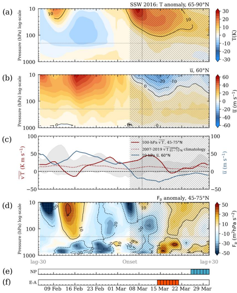
Figure A10: Same as for Fig. A2, but for the 2016 SSW. The time interval is shown for \pm 30 days from the central date (5 March).
