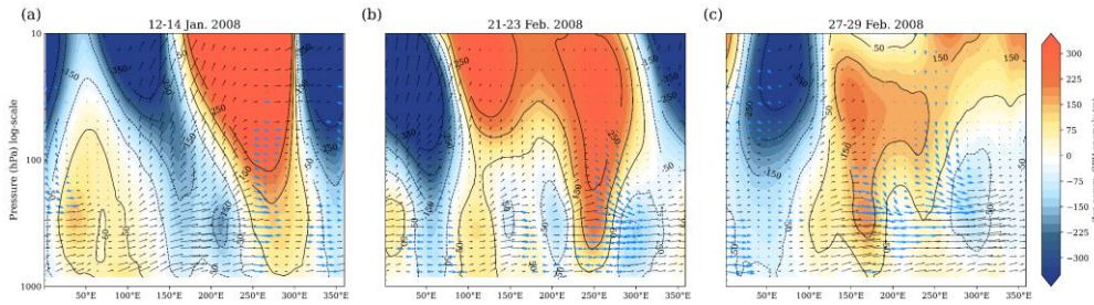
720 Figure B1. Evolution of the vertical and zonal components of the 3D Plumb flux (arrows), shown for the SSW 2008: before the SPV displacement (12-14 Jan.), during its displacement (21-23 Feb.) and during its recovery (27-29 Feb.) The vectors are plotted for every 5th longitude and pressure level. Blue vectors denote where the vertical component of Plumb flux is negative. Shading indicates the zonally asymmetric component of the geopotential height anomaly.
