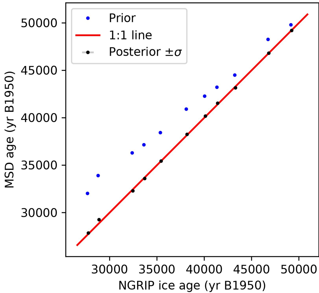
Figure 6: Synchronisation graph for the NGRIP-MSD site pair as produced by Paleochrono-1.1 in the AICC2023-Hulu dating experiment. Blue: prior scenario. Black: posterior scenario after optimization by Paleochrono-1.1. Red: the 1:1 line for comparison.
