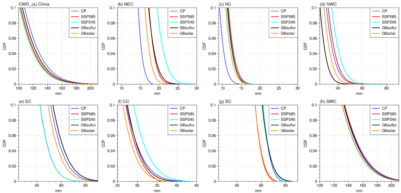
Figure 8. Same as Figure 5, but for CWD in China and 7 subregions.
