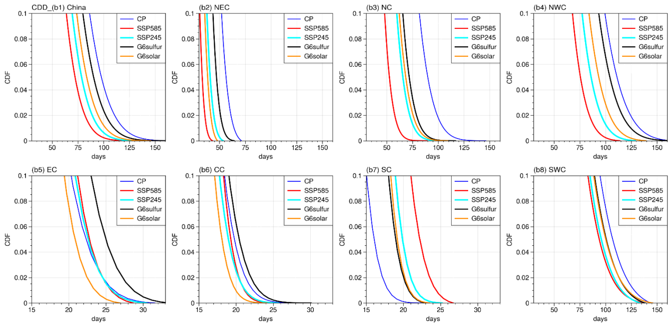
Figure 11. Same as Figure 5, but for DD (a1-a8) and CDD (b1-b8) in China and 7 subregions.
