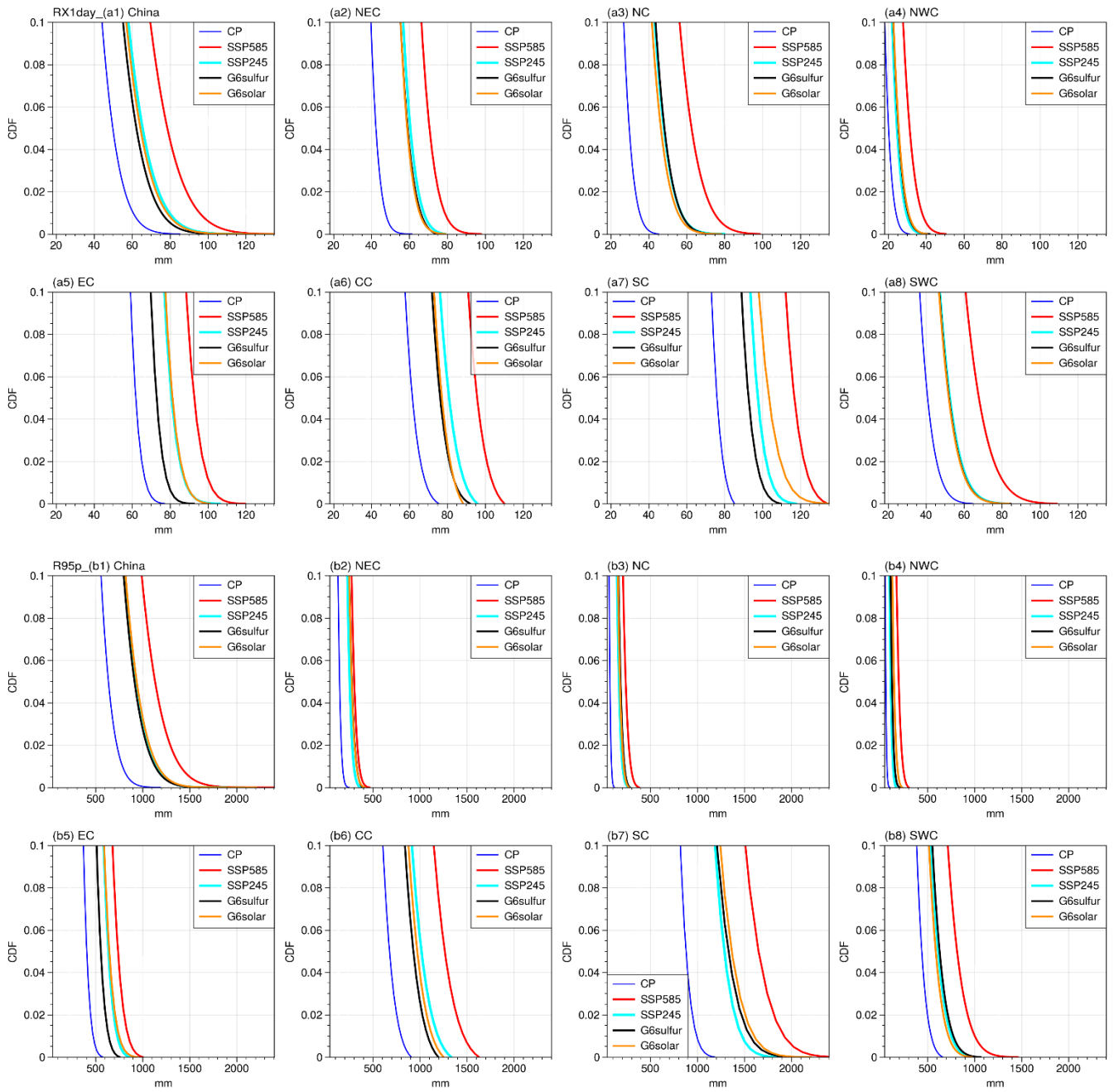
325 Figure 5. Cumulative distribution functions of RX1day (a1-a8) and R95p (b1-b8) in China and 7 subregions for different scenarios. The same processing was applied to all CDFs figures.
