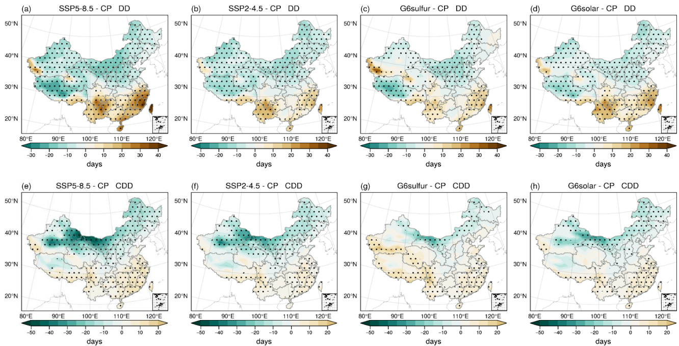
430 Figure 9. Same as Figure 3, but for (a-d) DD (days) and (e-h) CDD (days).
