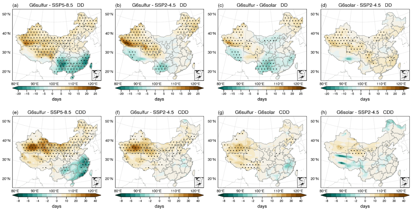
445 Figure 10. Same as Figure 4, but for (a-d) DD (days) and (e-h) CDD (days).
