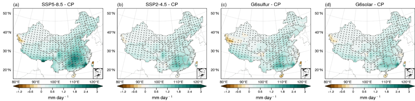
190 Figure 2. Relative changes in land precipitation ( \text{mm day}^{-1} ) of the period 2071-2100 compared to that of the CP (1981-2010) (a) SSP5-8.5, (b) SSP2-4.5, (c) G6sulfur, and (d) G6solar. The dotted areas indicate where the difference is statistically significant at the 95% confidence level using a Wilcoxon rank sum test.
