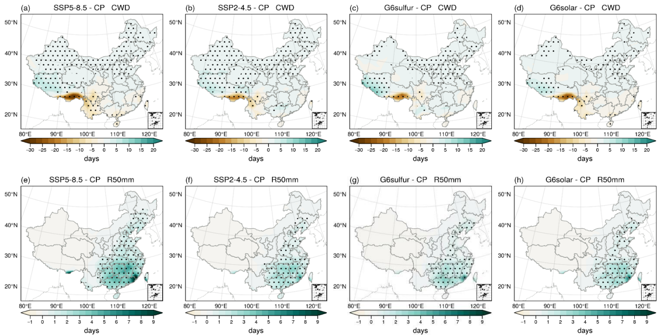
Figure 6. Same as Figure 3, but for CWD (a-d) and R50mm (e-h).
