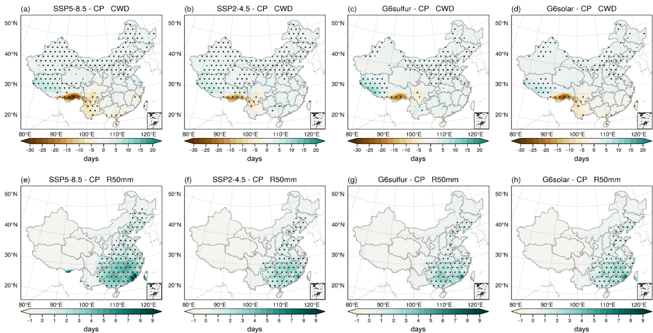
Figure 6. Same as Figure 3, but for CWD (a-d) and R50mm (e-h).
