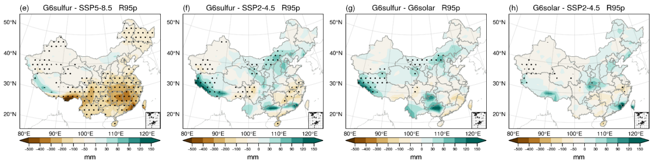
Figure 4. Differences in RX1Day (a-c) and R95p (d-f) for the future period of 2071 – 2100 between G6sulfur and SSP5-8.5 (a, e), SSP2-4.5 (b, f), and G6solar (c, g), as well as between G6solar and SSP2-4.5 (d, h). The dotted areas indicate where the difference is statistically significant at the 95% confidence level using a Wilcoxon rank sum test.
