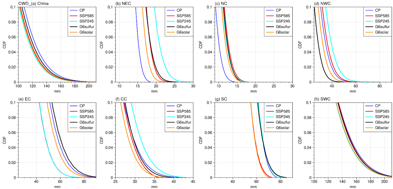
450 Figure 8. Same as Figure 5, but for CWD in China and 7 subregions.
