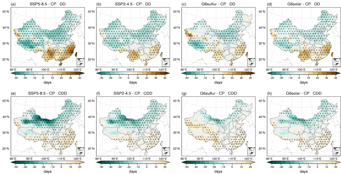
Figure 9. Same as Figure 3, but for (a-d) DD (days) and (e-h) CDD (days).
