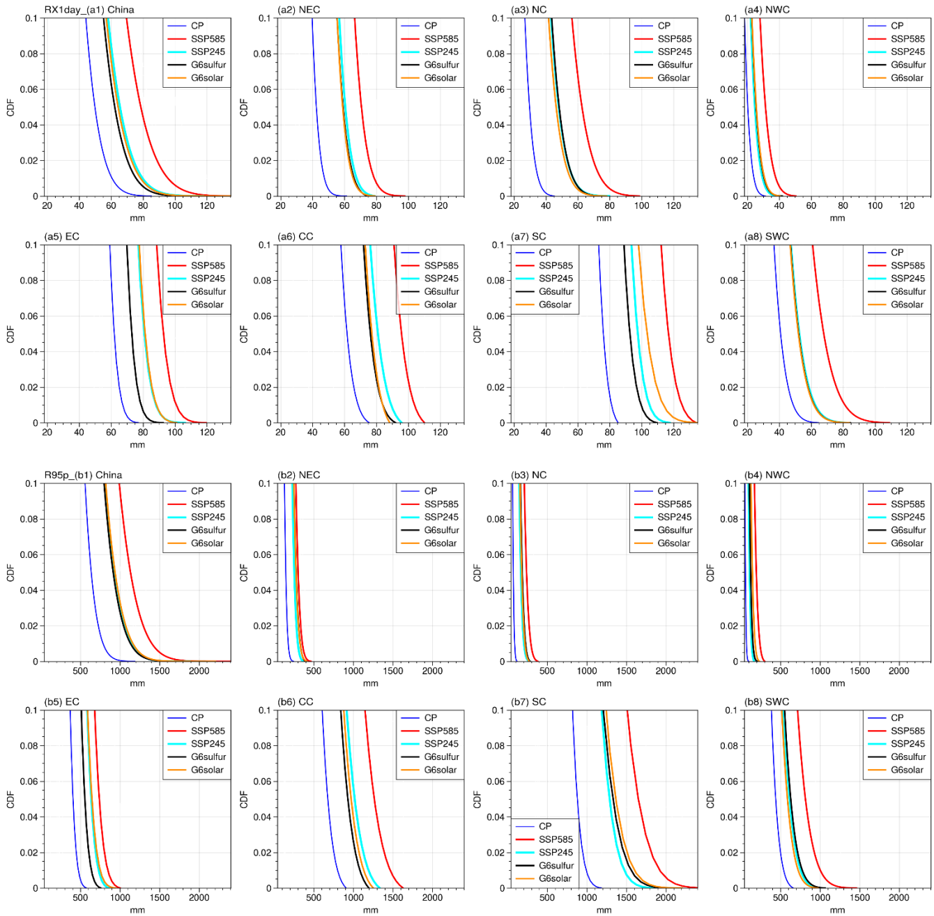
Figure 5. Cumulative distribution functions of RX1day (a1-a8) and R95p (b1-b8) in China and 7 subregions for different scenarios. The same processing was applied to all CDFs figures.
