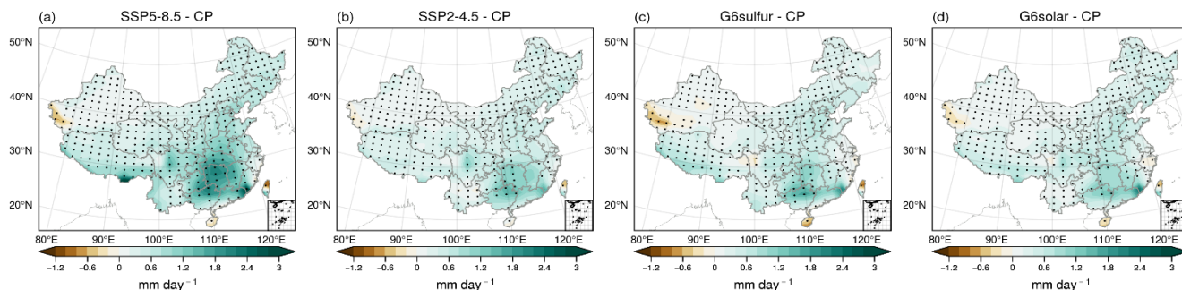
Figure 2. Relative changes in land precipitation (mm day -1 ) of the period 2071-2100 compared to that of the CP (1981-2010) (a) SSP5-8.5, (b) SSP2-4.5, (c) G6sulfur, and (d) G6solar. The dotted areas indicate where the difference is statistically significant at the 95% confidence level using a Wilcoxon rank sum test.
