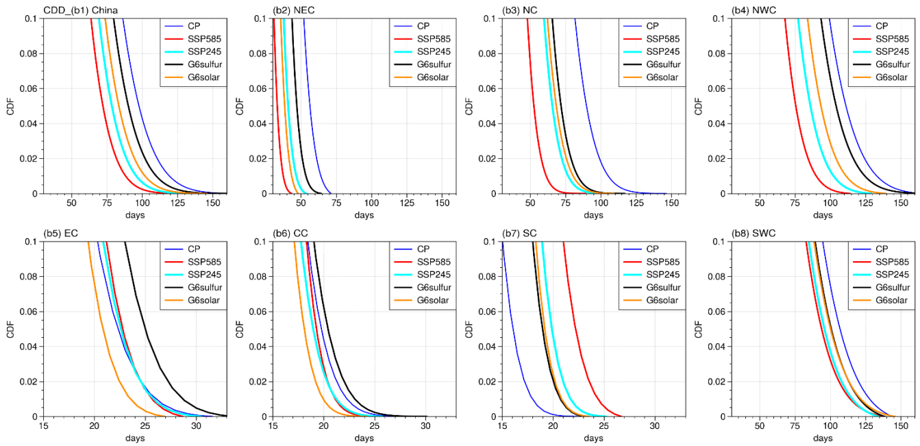
Figure 11. Same as Figure 5, but for DD (a1-a8) and CDD (b1-b8) in China and 7 subregions.
