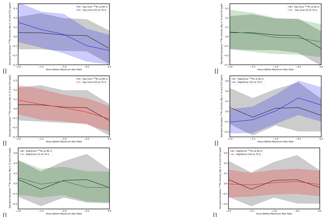
Figure S1. Composite plot with ATTO data in rain event-normalized representation, which shows data from two hours before to the time of the maximum rain rate for January 2019 to December 2020. Variations are presented as a number of standard deviations. The upper panel corresponds to the daytime, and the bottom panel for the nighttime calculations. All data was collected at the top of the Instant tower at height. All figures show the variation ^{222}\text{Rn} combined with Figure A) and D) \text{CO}_2 , during the day and night, B) and E) \text{CO} , during the day and night and C) and F) \text{CH}_4 , during the day and night
