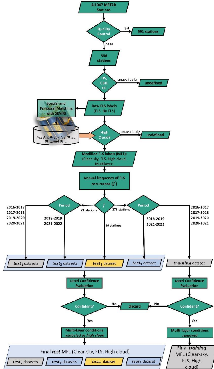
Figure A1. Schematic description of the process followed in Sect. 2 for creation of the MFL (Modified FLS Labels) included the datasets “training”, “test 1 ”, “test 2 ”, “test 3 ”, and “test 4 ”.
