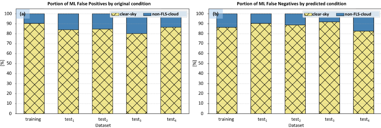
415 Figure 3. Detailed information on false-positive and false-negative (see Appendix B) predictions of the FLS ML technique across training, test 1 , test 2 , test 3 , test 4 datasets. Panel (a) shows the percentage of false-positive instances that were clear-sky and non-FLS-cloud contaminated according to the ground truth dataset (i.e., MFL). Panel (b) shows the percentage of false-negative instances that were categorized as clear-sky and non-FLS-cloud by the ML algorithm.
