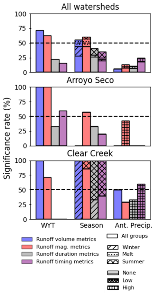
Figure 7: Summary plots of the relative significance rates of four runoff event metric groups (colored bars) with respect to three time-varying hydrologic controls (x-axis) for all watersheds (top panel), Arroyo Seco, and Clear Creek (bottom panel) under undisturbed conditions. The 50% relative significance rate is indicated
