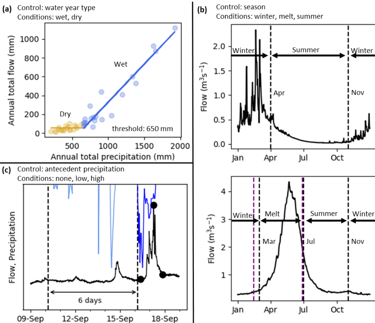
225 Figure 4: Example hydrologic condition identification for time-varying hydrologic controls. (a) Water year type wet (blue) and dry (orange) years for Arroyo Seco. The ordinary least squares linear regression lines for above and below the threshold are shown. (b) Seasons (vertical dashed) delineated from the undisturbed average annual hydrograph for a no-snow watershed (top) with winter and summer (Arroyo Seco) and a snow dominated watershed (bottom) with winter, melt, and summer (Clear Creek). The minimum and maximum snow melt dates are shown consecutively (purple dashed). (c) The six-day prior to rainfall start antecedent
