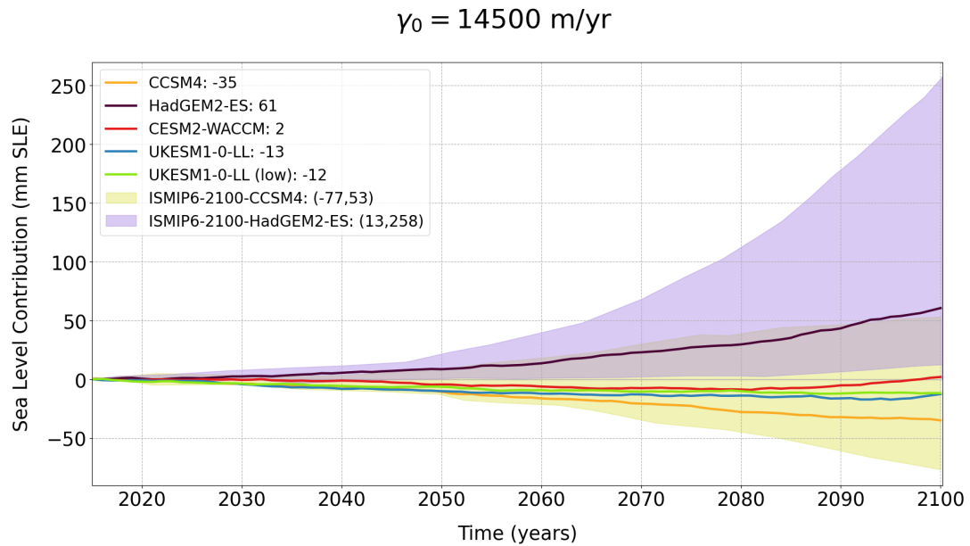
Figure A10. Sea level contribution (mm SLE) for the experiments carried out with five GCM forcings under high-emission scenarios, until the year 2100 for the medium value of \gamma_0 . Solid lines represent the curve for the values of \gamma_0 and the shading the overall results from Seroussi et al. (2020) with different ice-sheet models for the forcings given by CCSM4 and HadGEM2-ES.
