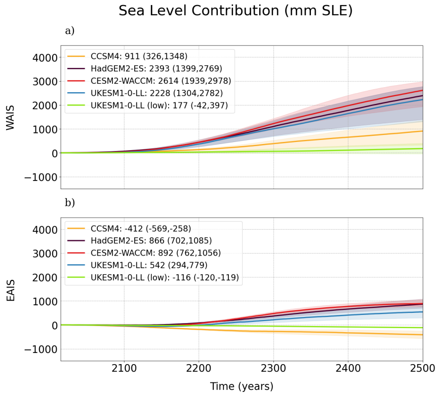
Figure 7. Evolution of the sea-level contribution (mm SLE) from the two main regions of Antarctica, the WAIS (including the Antarctic Peninsula, a) and the EAIS (b), relative to the control run, since the start of the simulations in 2015 to year 2500.
