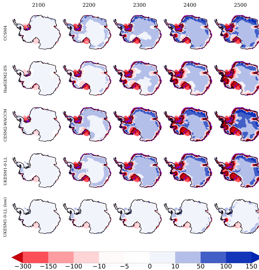
Figure 8. Ice thickness anomalies (in m) for the years 2100, 2200, 2300, 2400 and 2500 with respect to the start of the simulations for the set of five experiments carried out with the medium value of \gamma_0 . The grounding line is represented by black and violet colours for 2500 and 2015 respectively. To show negative anomalies in the WAIS, no masking has been implemented as time evolves, keeping the original coastlines.
