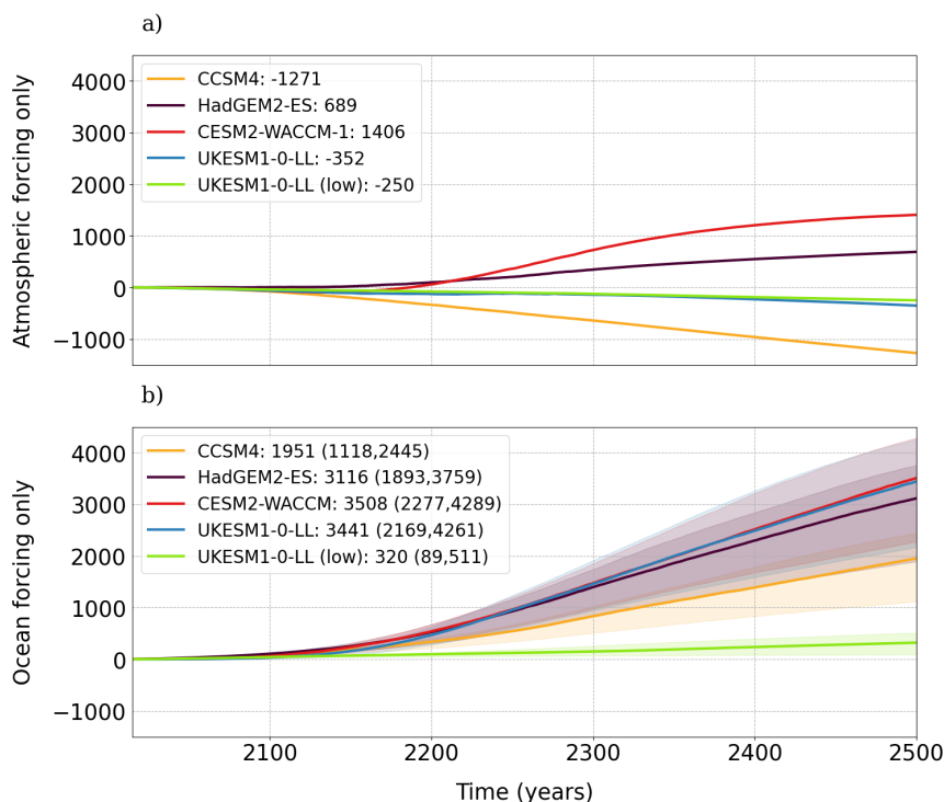
Figure 10. Sea-level contribution of the AIS (mm SLE) in the cases where only the forcing of the atmosphere (a) or the ocean (b) are considered. The shading in b) indicates the spread produced by the effect of the values of \gamma_0 , while in a), as the optimization process leads to similar initial ice sheet states regardless of \gamma_0 , the ocean fields maintain the present-day state.
