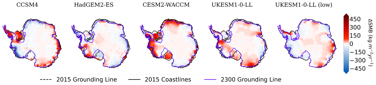
Figure A2. SMB ( \text{kg m}^{-2} \text{yr}^{-1} ) anomaly for the different GCM models between 2300 and 2015.
