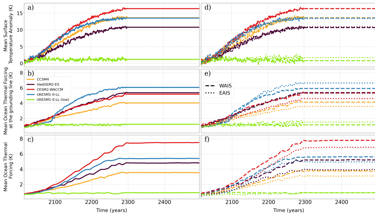
Figure 1. Mean evolution of the atmospheric (a), oceanic thermal forcing at the grounding line depth fixed in 2015 (b) and thermal forcing at the evolving grounding lines in the AIS (c) in the AIS for the five experiments carried out models considered for simulation : CCSM4 (RCP8.5), HadGEM2-ES (RCP8.5), CESM2-WACCM (SSP5-8.5), UKESM1-0-LL (SSP5-8.5) and UKESM1-0-LL (SSP1-2.6). For (d), (e) and (f), same as in (a), (b) and (c) respectively but for the WAIS and EAIS. From 2300 to 2500 a constant climate is imposed through the average climatic conditions in the period 2291-2300.
