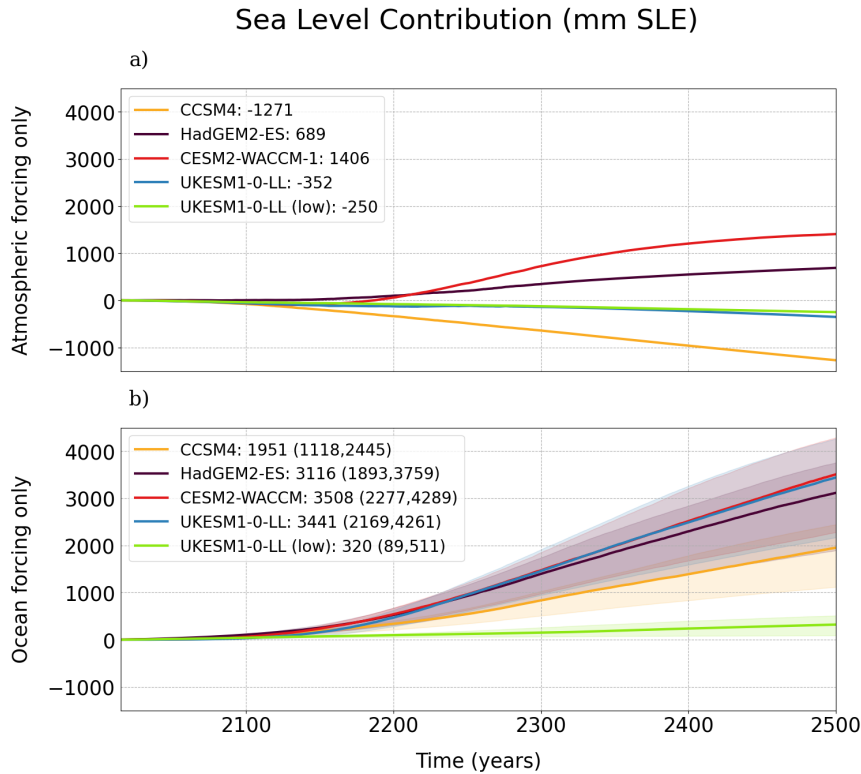
Figure 10. Sea-level contribution of the AIS (mm SLE) in the cases where only the forcing of the atmosphere (a) or the ocean (b) are considered. The shading in b) indicates the spread produced by the effect of the values of \gamma_0 , while in a), as the optimization process leads to similar initial ice sheet states regardless of \gamma_0 , the ocean fields maintain the present-day state.
