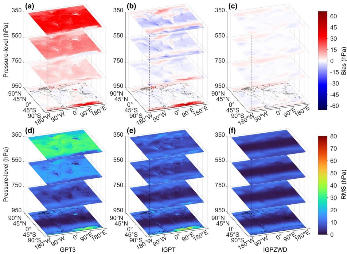
260 Figure 9: Global distribution of bias (a-c) and RMS (d-f) for the pressure predicted by the GPT3, IGPT, and IGPZWD models validated using the ERA5 pressure at the levels of 950, 750, 550 and 350 hPa in 2020.
