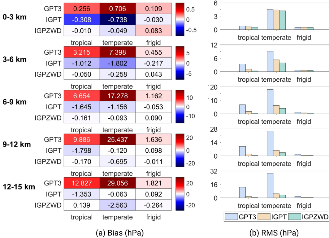
Figure 13: Mean bias (a) and RMS (b) values (d1-d5) for pressure predicted by the GPT3, IGPT and IGPZWD models validated using the radiosonde pressure data at five height ranges of the tropical, temperate, and frigid zones.
