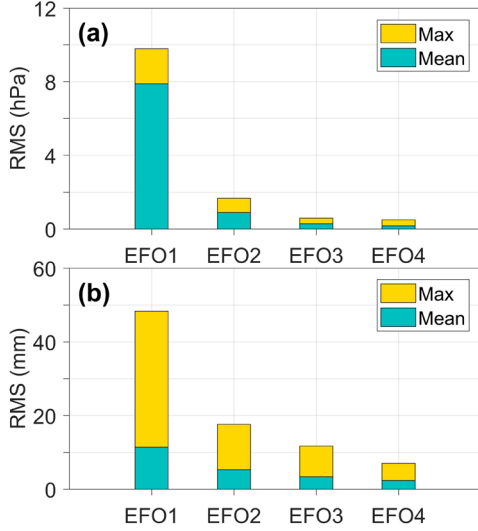
195 Figure 4: The global mean and maximum RMS values for pressure (a) and ZWD (b) fitted using EFO1, EFO2, EFO3 and EFO4.
