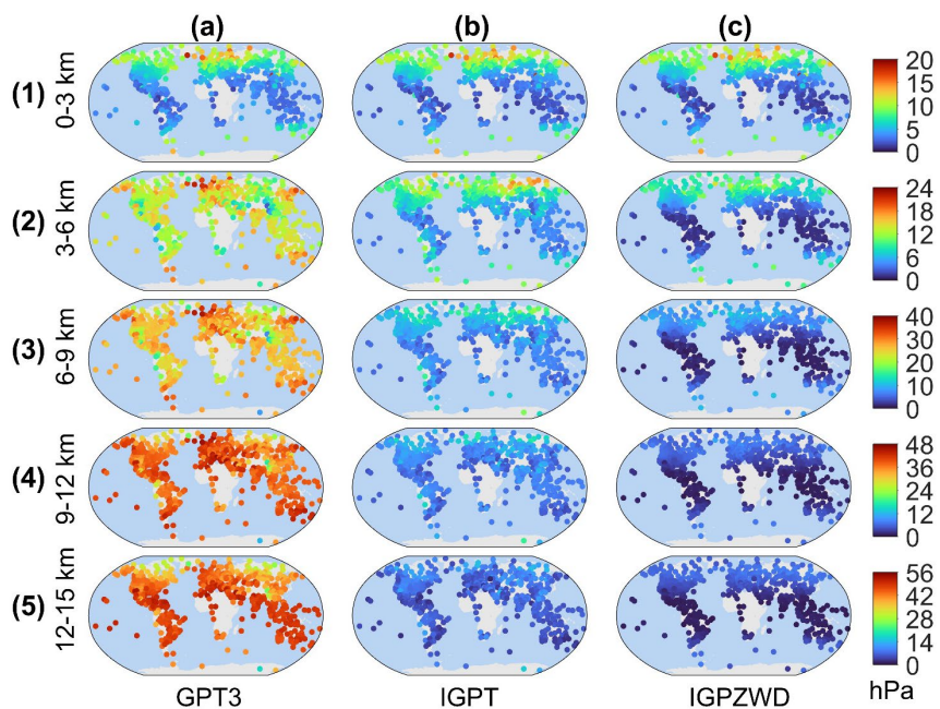
435 Figure A2: Distribution of RMS for pressure predicted by the GPT3, IGPT and IGPZWD models validated using the radiosonde pressure data at the height ranges of 0-3 (a1-c1), 3-6 (a2-c2), 6-9 (a3-c3), 9-12 (a4-c4) and 12-15 (a5-c5) km in 2020.
