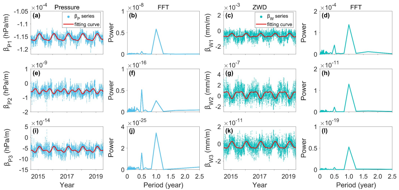
200 Figure 5: The time series, fitting curves and power spectral density of \beta_p and \beta_w of the first (a-d), second (e-h) and third (i-l) orders at the grid point of 20.5°N, 120.5°W.
