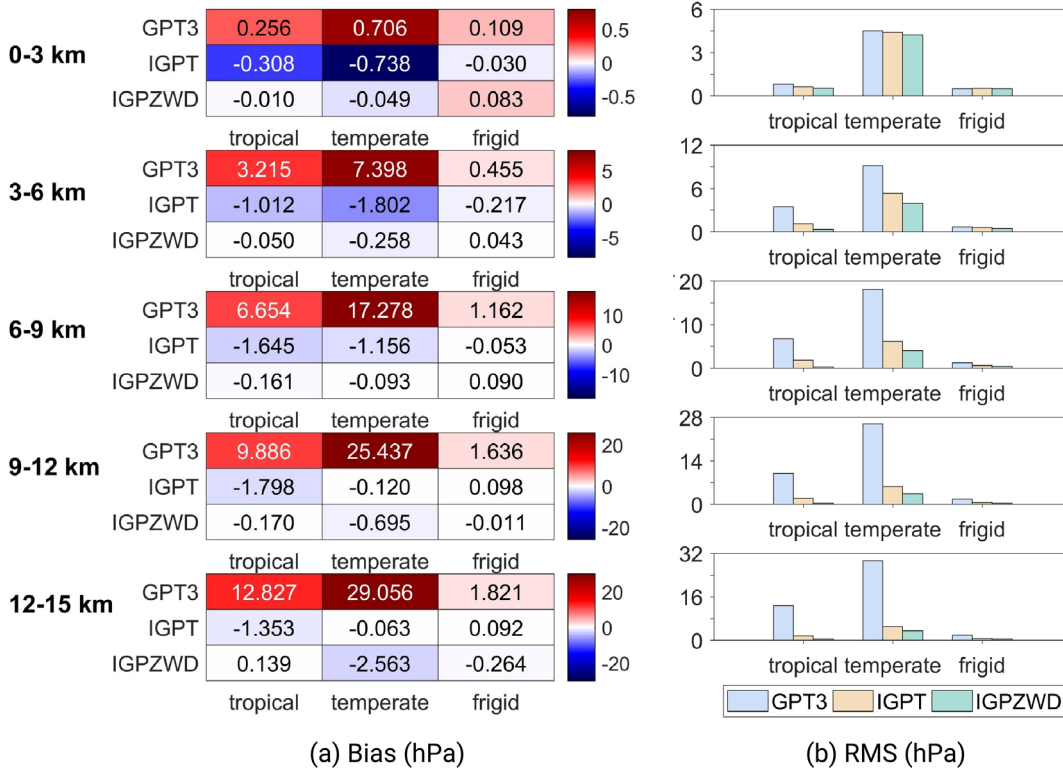
320 Figure 13: Mean bias (a) and RMS (b) values (d1-d5) for pressure predicted by the GPT3, IGPT and IGPZWD models validated using the radiosonde pressure data at five height ranges of the tropical, temperate, and frigid zones.
