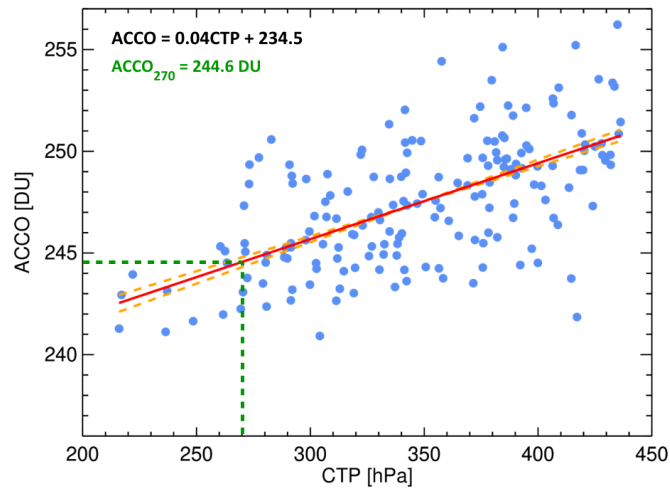
Figure 6. A scatter plot of ACCO (DU) and CTPs (hPa) with a regression line (red). Individual data points are single measurements within the auto-selected reference sector (latitude band 2.25^{\circ}\text{S} - 0.25^{\circ}\text{S} and longitude band 26.75^{\circ}\text{E} - 46.75^{\circ}\text{E} ) around Nairobi, Kenya ( 1.3^{\circ}\text{S} , 36.8^{\circ}\text{E} ) on 1st January 2019. The orange lines show the upper and lower bounds of the 95% confidence interval. The ACCO above the reference altitude 270 hPa is 244.6 DU (green dashed line). The regression line was determined using the Theil-Sen estimator.
