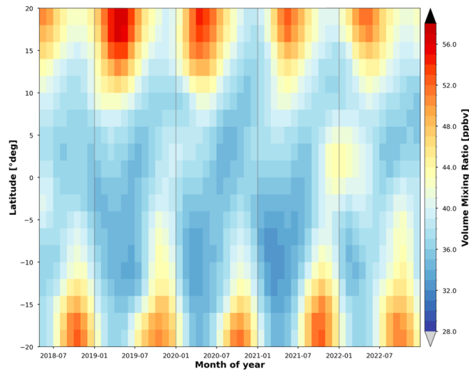
Figure 3. Monthly mean CHOVA V6.7 ozone volume mixing ratios in the upper troposphere as a function of month and latitude band. The values are computed for the global sector ( 180^\circ\text{E} to 180^\circ\text{W} ) and the period from 2018/05 to 2022/12.
