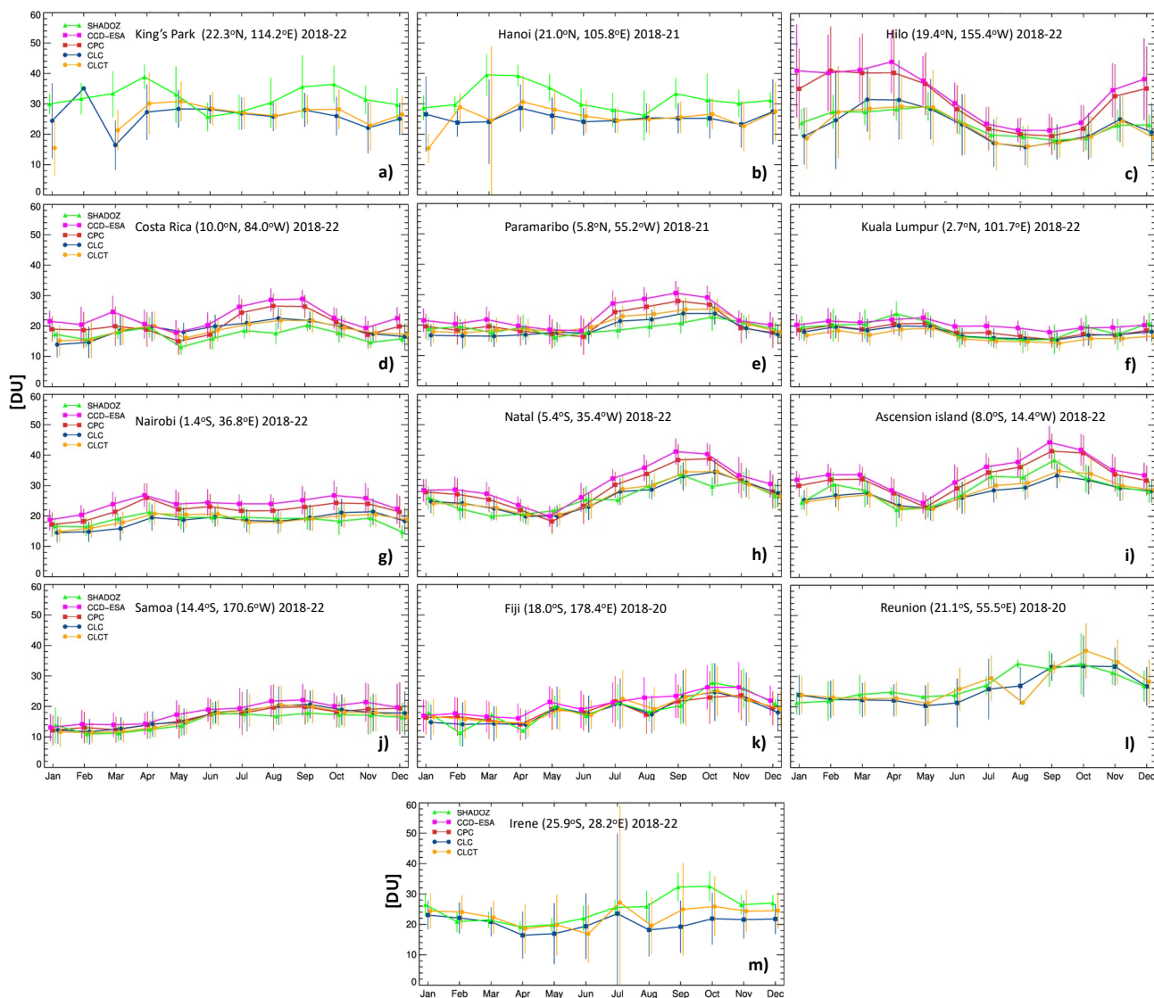
Figure 10. Seasonal variation of TROPOMI and ozonesonde tropospheric ozone columns up to 270 hPa at thirteen SHADOZ sites from 2018-2022. The green line indicates ozonesondes. The magenta line indicates TCO-CCD-ESA. The red, blue, and yellow lines are CPC, CLC, and CLCT results, respectively. The error bar is the corresponding standard deviation ( 1\sigma ) of the monthly means. No error bars are shown for stations with only one launch per month. The time period varies with stations according to the data availability.
