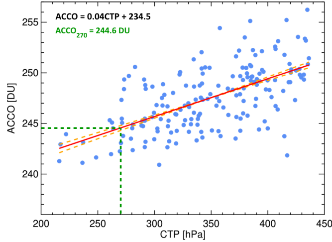
Figure 6. A scatter plot of ACCO (DU) and CTPs (hPa) with a regression line (red). Individual data points are single measurements within the auto-selected reference sector (latitude band 2.25°S - 0.25°S and longitude band 26.75°E - 46.75°E) around Nairobi, Kenya (1.3°S, 36.8°E) on 1st January 2019. The orange lines show the upper and lower bounds of the 95% confidence interval. The ACCO above the reference altitude 270 hPa is 244.6 DU (green dashed line). The regression line was determined using the Theil-Sen estimator.
