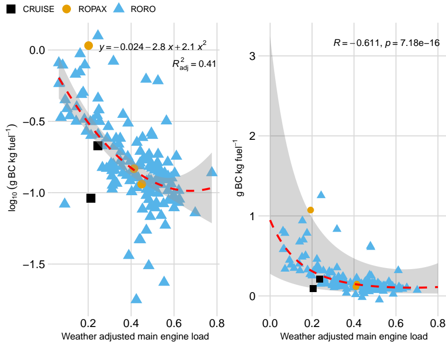
Figure 6. Left: scatterplot of \log_{10} BC emission factor ( \text{g kg fuel}^{-1} ) as a function of weather adjusted main engine load with 2^{\text{nd}} degree polynomial regression (red dashed line) and 95% confidence interval (grey area). Right: BC emission factor ( \text{g kg fuel}^{-1} ) with the same regression (red dashed line) and 95% prediction interval (grey area).
