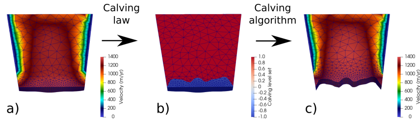
Figure 1. Illustrating the difference between the calving model, algorithm and law. a) The initial flow solution. The calving law then predicts calving based off the solved variables on the initial geometry. b) The predicted calving based on the calving law. This prediction is in the form of a level set variable which is then fed to the calving algorithm. Nodes with a negative value (in blue) show areas to be calved and those with positive values (in red) show the remaining glacier domain. c) The new geometry with all the variables interpolated across (from a)) showing the interpolated velocity field. The calving model represents the combination of both the calving law and algorithm allowing you to go from a) to c).
