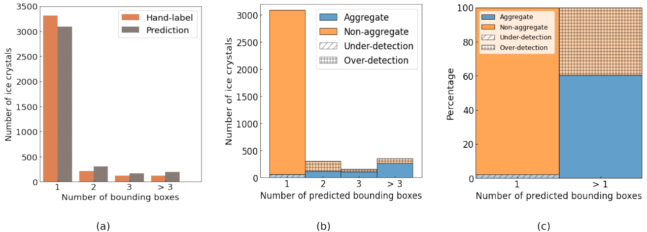
Figure 3. (a) Histogram of the number of hand-labeled (orange) and model-predicted (brown) bounding boxes (average over five models). Instances with more than three bounding boxes are combined into a single category and instances with zero detected bounding boxes (11) are excluded. (b) Histogram with the number of predicted bounding boxes for hand-labeled aggregated (blue) and non-aggregated (orange) ice crystals. The shaded orange and blue regions denote areas of over-detection and under-detection, respectively. (c) Same as panel (b), but all bounding boxes larger than one are combined, thereby providing an intuitive visualization of the percentages of over-detection and under-detection.
