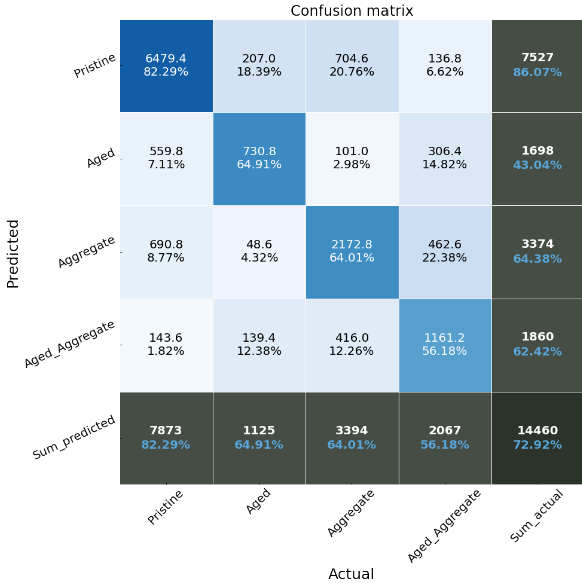
Figure 10. Similar confusion matrix as Fig. 6, but for generalization dataset.
