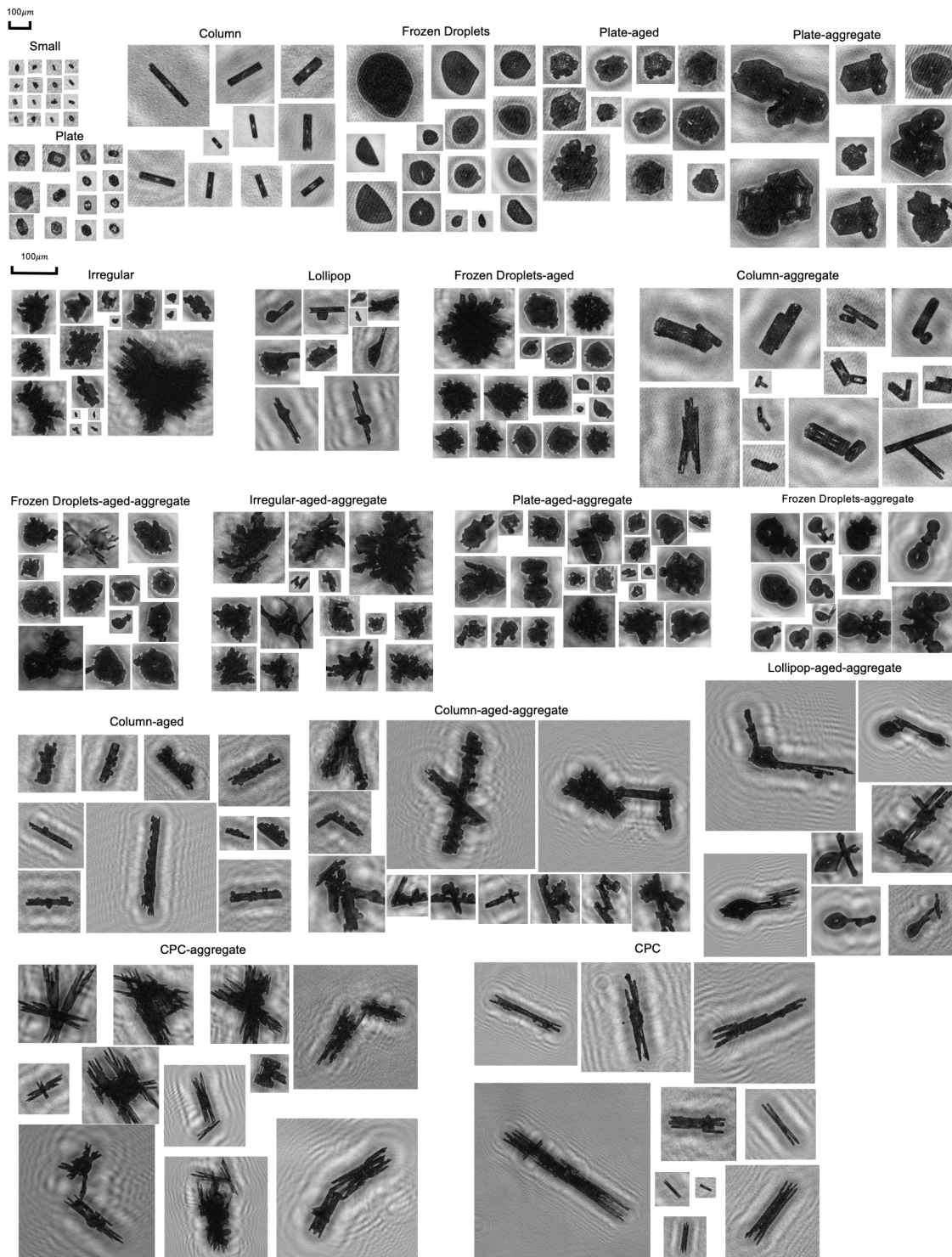
Figure B2. A randomly selected sample of ice crystal images from each category
