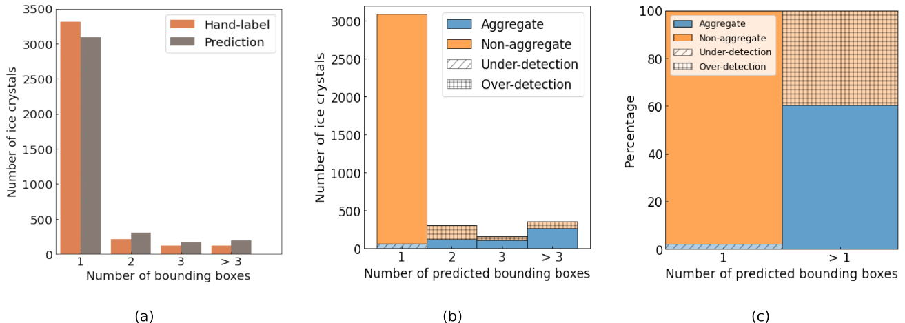
Figure 4. (a) Histogram of the number of hand-labeled (orange) and model-predicted (brown) bounding boxes (average over five models). Instances with more than three bounding boxes are combined into a single category and instances with zero detected bounding boxes (11) are excluded. (b) Histogram with the number of predicted bounding boxes for hand-labeled aggregated (blue) and non-aggregated (orange) ice crystals. The shaded orange and blue regions denote areas of over-detection and under-detection, respectively. (c) Same as panel (b), but all bounding boxes larger than one are combined, thereby providing an intuitive visualization of the percentages of over-detection and under-detection.
