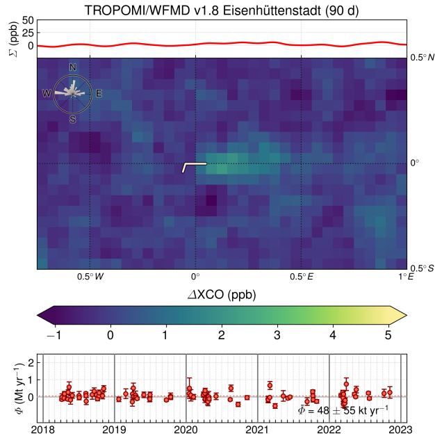
Figure 7. As previous figures but for Eisenhüttenstadt.
