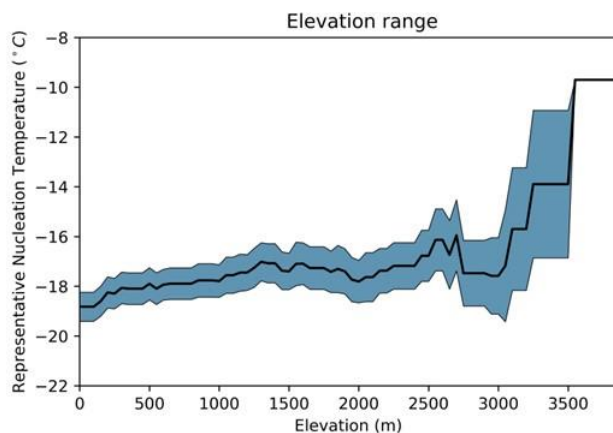
240 Figure 4. Plot of possible growth elevation plotted against representative nucleation temperature ( T at n_m(T) = 100000 \text{ g}^{-1} ), the values for which are reported in Table S1. The black line represents the mean across species and the blue shaded area denotes the standard error.
