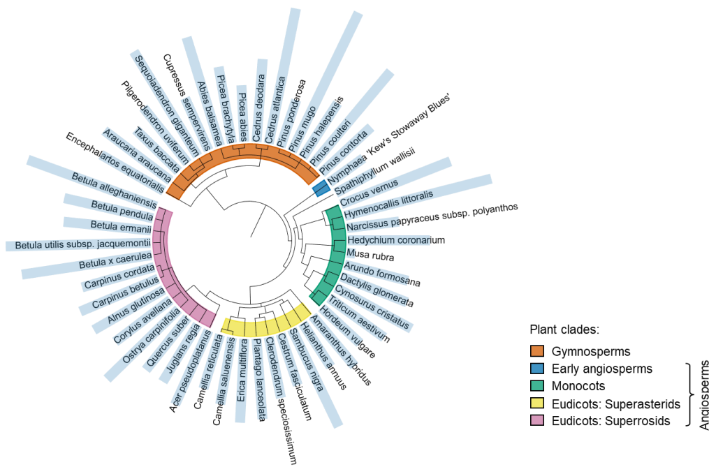
160 Figure 2. Phylogenetic tree showing the level of IN activity associated with the named species pollen indicated by the length of the blue bars; short bar indicates low IN activity and vice versa. The length of the blue bar is calculated from the representative nucleation temperature of the named species' pollen minus the lowest representative nucleation temperature value ( Musa rubra T_{rep} ) plus one. The main plant clades of species sampled for this study are indicated by coloured arcs. Orange for gymnosperms and other colours for angiosperms: blue (early angiosperms), green (monocots), yellow (eudicots: superasterids), pink (eudicots: superrosids).
