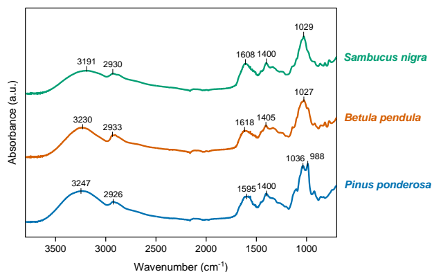
285 Figure 5. Fourier-transform infrared absorption spectra for water-soluble material from pollen of three plant species: Pinus ponderosa (low IN activity), Betula pendula (moderate IN activity), and Sambucus nigra (high IN activity). The absorption spectra have been normalised and offset along the y-axis for ease of comparison.
