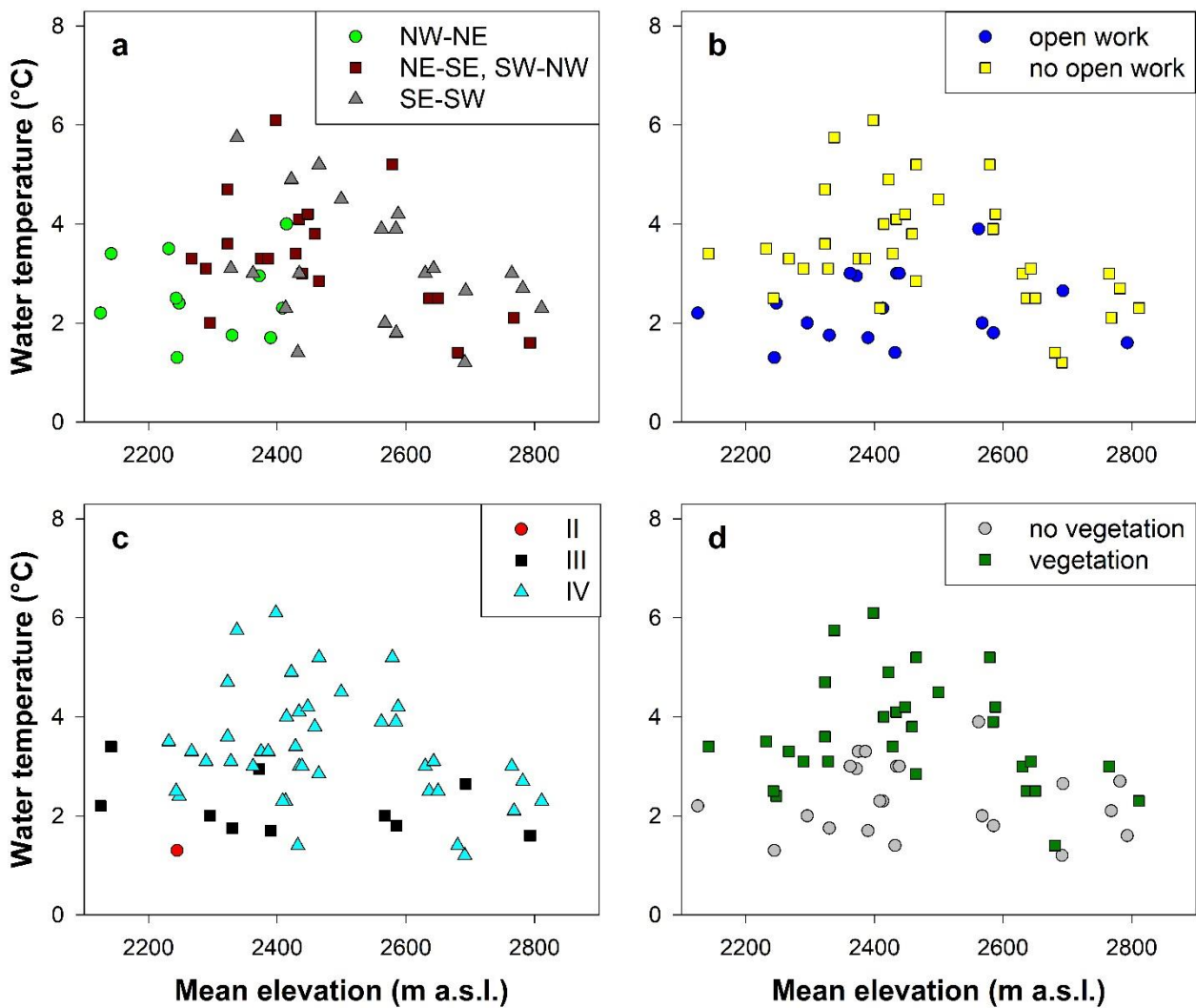
386 Figure 7: Relationship between spring-water temperature of relict rock glaciers and mean catchment elevation clustered 387 in a) three classes of mean catchment aspect, b) two classes of open work deposits in the spring upslope area, c) three 388 classes of rock glacier front characteristics, and d) two classes of rock glacier vegetation cover. Classes are described in 389 Table 3.
