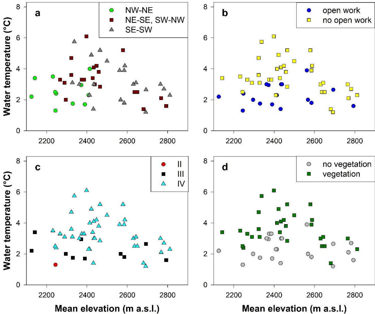
381 Figure 7: Relationship between spring-water temperature of relict rock glaciers and mean catchment elevation clustered 382 in a) three classes of mean catchment aspect, b) two classes of open work deposits in the spring upslope area, c) three 383 classes of rock glacier front characteristics, and d) two classes of rock glacier vegetation cover. Classes are described in 384 Table 3.
