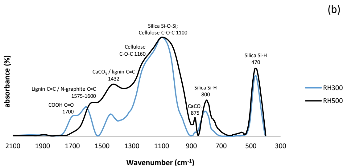
272 Fig. 2. FTIR spectra the biochars in the wave number range of 400-2000 \text{cm}^{-1} . Notes: SM300, sheep 273 manure biochar produced at 300 °C; SM500, sheep manure biochar produced at 500 °C; RH300, rice husk biochar 274 produced at 300 °C; RH500, rice husk biochar produced at 500 °C.
