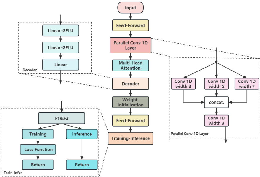
Figure 43: The model framework and network structure of Transformer_CNN.
