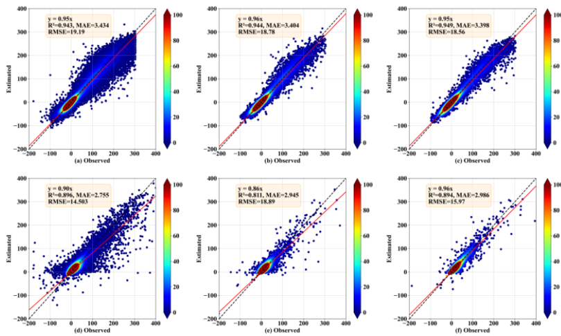
Figure 54: Scatter density plots of observed values and Transformer_CNN estimated values, where a) and d) are for the training dataset, b) and e) are for the validation dataset, and c) and f) are for the test dataset. a), b), and c) are estimates for H, while d), e), and f) are estimates for LE.
