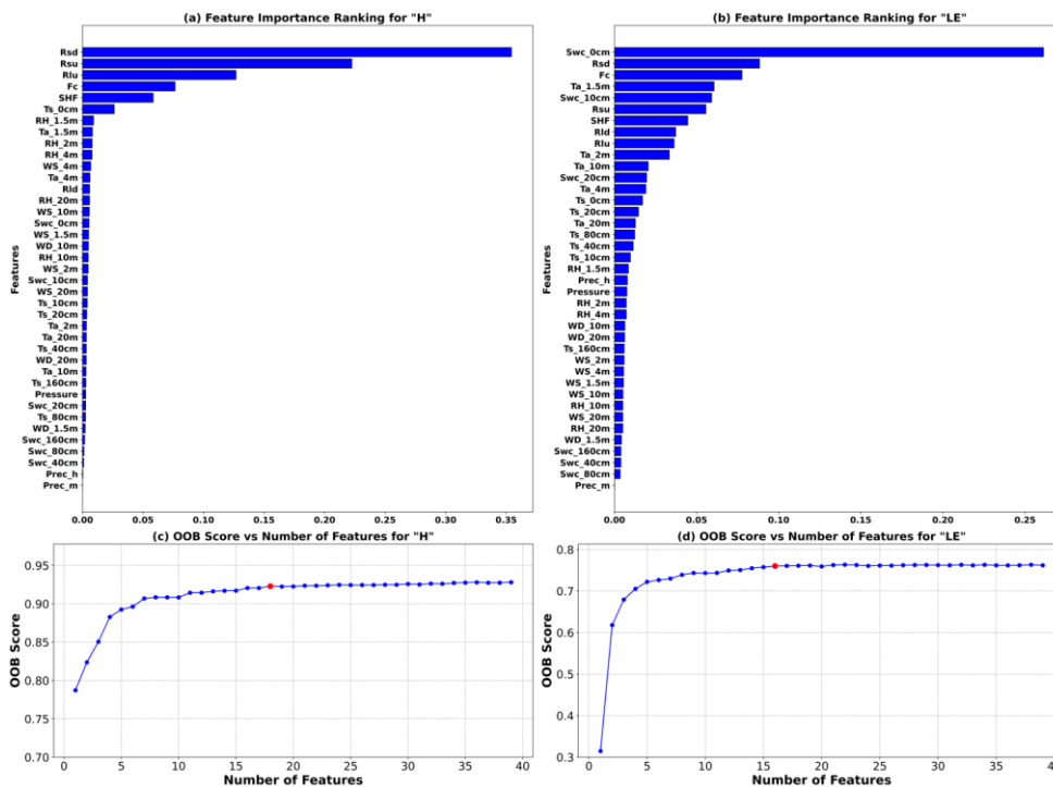
Figure 22: (a) Importance index for sensible heat flux (H), (b) Importance index for latent heat flux (LE), (c) OOB scores for different feature combinations of sensible heat flux based on Random Forest (the red dot indicates the maximum value), (d) OOB scores for different feature combinations of latent heat flux based on Random Forest (the red dot indicates the maximum value).
