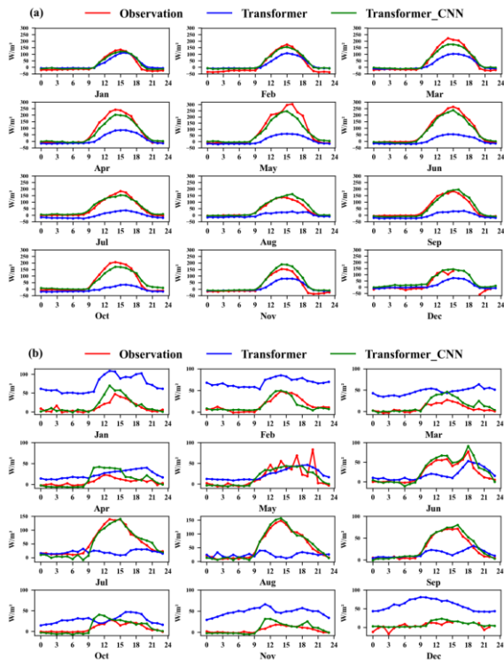
Figure 65: Observed values, Transformer estimated values, and Transformer_CNN estimated values for the monthly average diurnal variation curves in the test set (2012) are shown (x-axis is in hours). Specifically, (a) represents the sensible heat flux (H), and (b) represents the latent heat flux (LE).
