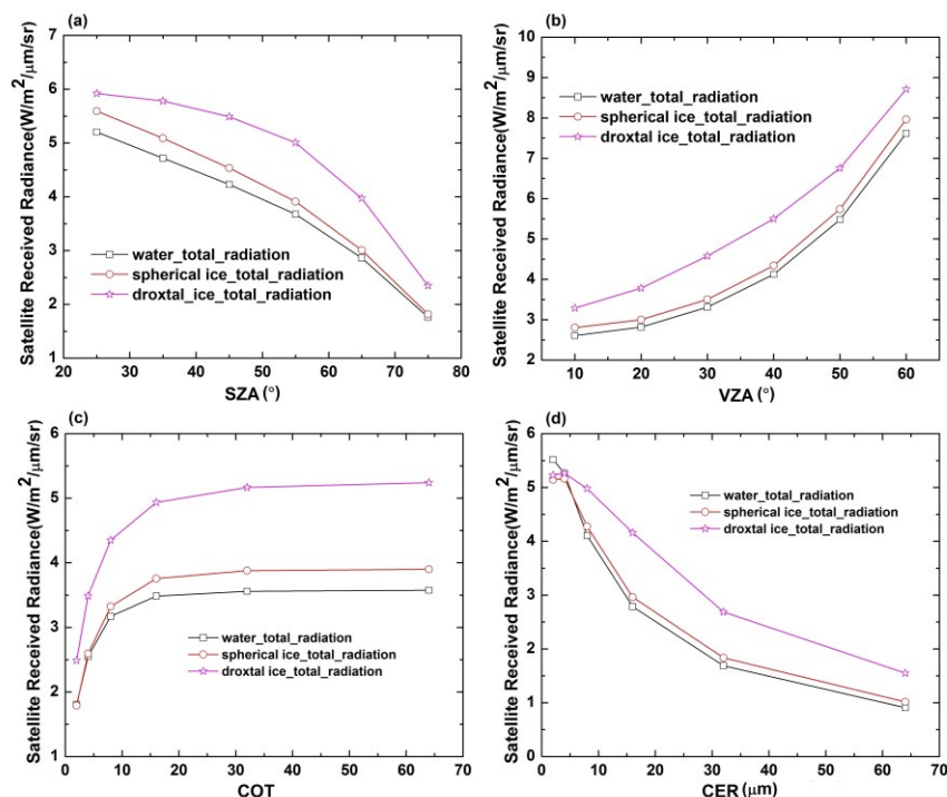
Figure 1: Sensitivity of satellite radiance at 2.3 \mu\text{m} channel for liquid droplets, spherical ice particles, and droxtals to different parameters. a. VZA=30°, RAA=180°, COT=10, CER=12 \mu\text{m} . b. SZA=60°, RAA=180°, COT=10, CER=12 \mu\text{m} . c. SZA=60°, VZA=30°, RAA=180°, CER=12 \mu\text{m} . d. SZA=60°, VZA=30°, RAA=180°, COT=10. For all cases surface albedo=0.1, cloud bottom and top height 3–5 km.
