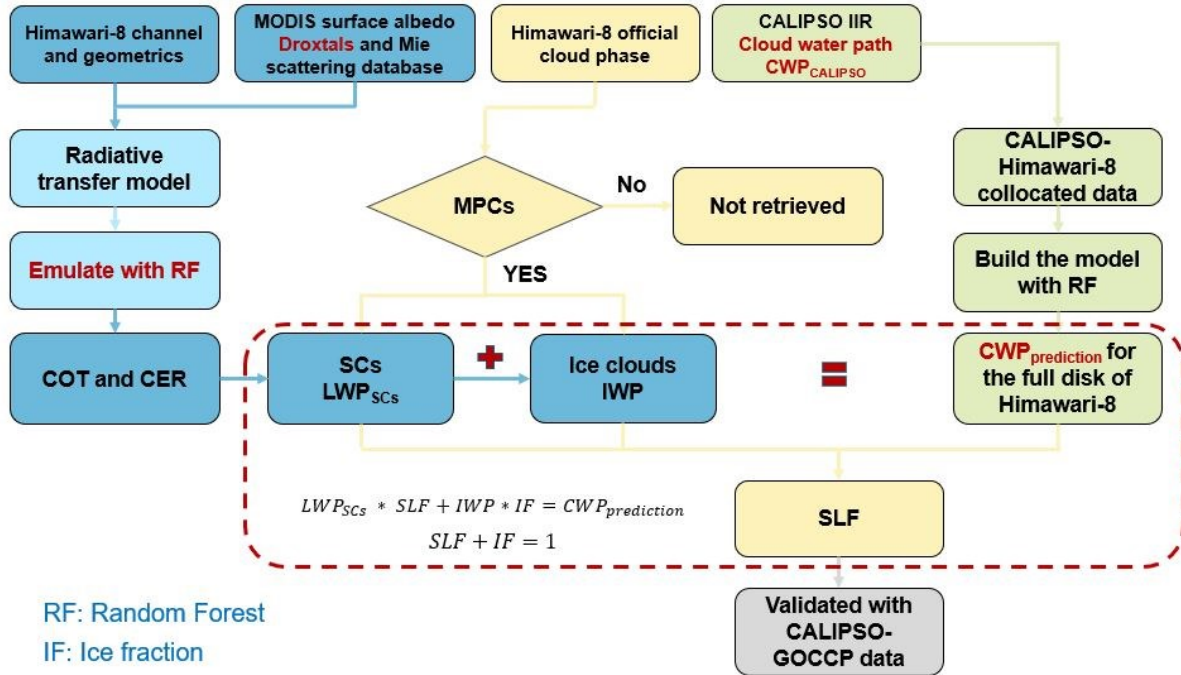
170 Figure 2: Roadmap of the SLF retrieval process and subsequent validation. The retrieval process is delineated into three distinct steps, each indicated by color-coded rectangles: blue, green, and yellow.
