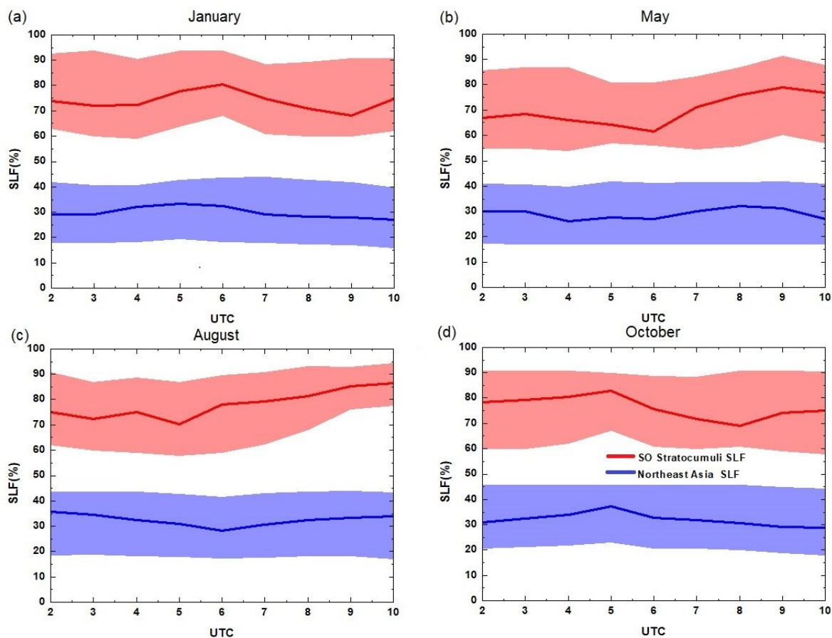
310 Figure 7: The diurnal cycle of the SLF (maximum, average, minimum) in MPCs over a larger range in the SO (red pattern) and Northeast Asia (blue pattern) represented by two rectangles in Fig. 3 in (a) January, (b) May, (c) August and (d) October of 2017.
