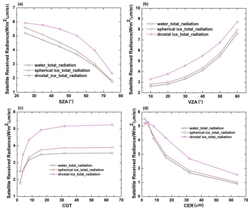
155 Figure 1: Sensitivity of satellite radiance at 2.3 \mu\text{m} channel for liquid droplets, spherical ice particles, and droxtals to different parameters. a. VZA=30^\circ , RAA=180^\circ , COT=10 , CER=12\mu\text{m} . b. SZA=60^\circ , RAA=180^\circ , COT=10 , CER=12\mu\text{m} . c. SZA=60^\circ , VZA=30^\circ , RAA=180^\circ , CER=12\mu\text{m} . d. SZA=60^\circ , VZA=30^\circ , RAA=180^\circ , COT=10 . For all cases surface albedo=0.1, cloud bottom and top height 3–5 km.
