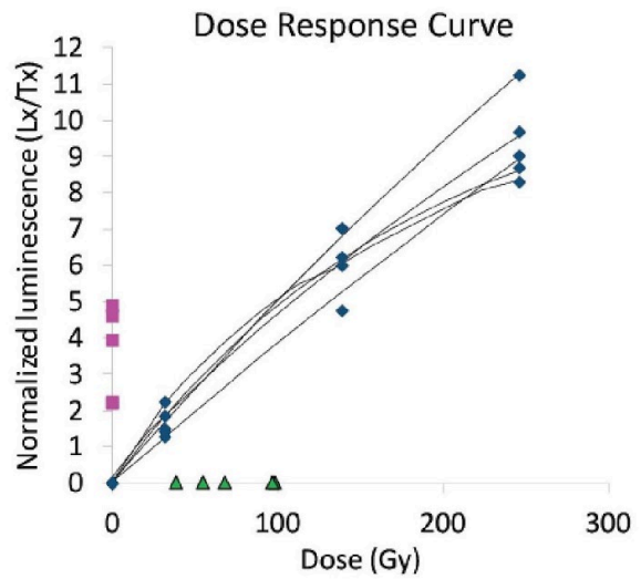
47 Figure S7. Example luminescence signal decay (left) and dose-response curves from 5 aliquots from each of the 48 luminescence samples.
