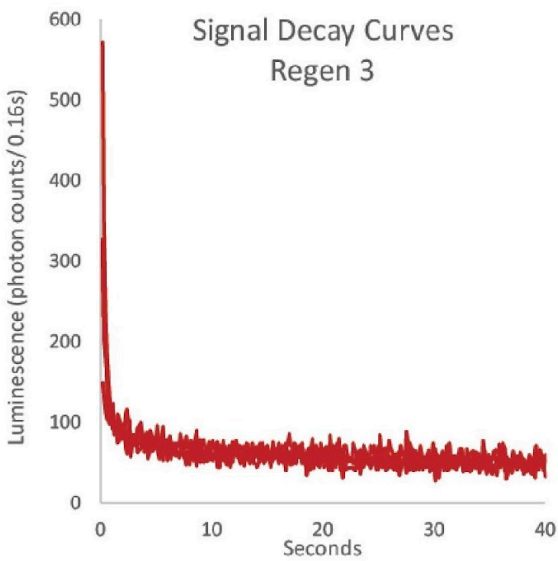
47 Figure S7. Example luminescence signal decay (left) and dose-response curves from 5 aliquots from each of the 48 luminescence samples.
