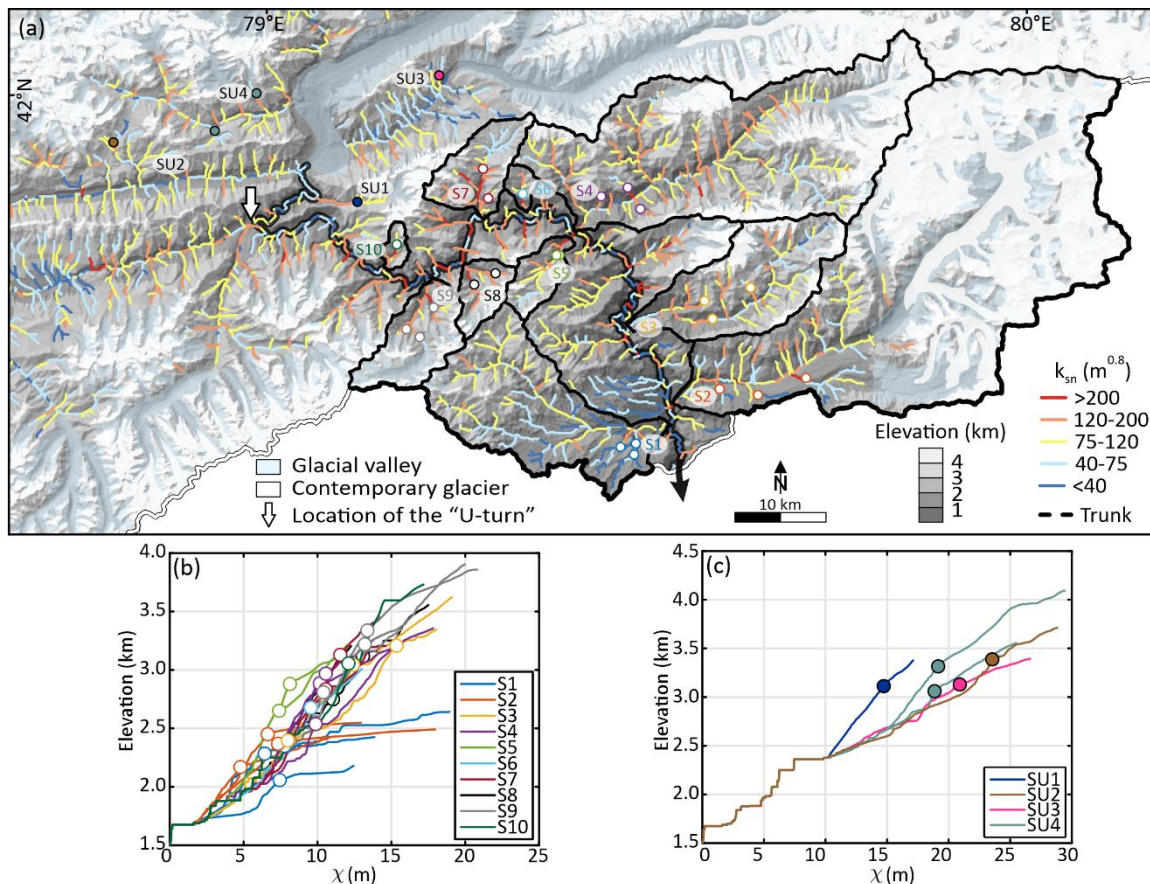
Figure 5 (a) Ten sub-catchments (outlined in black) downstream of the “U-turn” in Saryjaz (outlined in white with black edges) with transient knickpoints both downstream (label starts from S) and upstream (label starts from SU); \chi - z plots of transient knickpoints (b) downstream of the “U-turn”, and (c) upstream of the “U-turn”. Black shadow beneath the colored stream indicates the flow direction of the trunk. Labels indicate the sub-catchment number, following information from Table S1.
