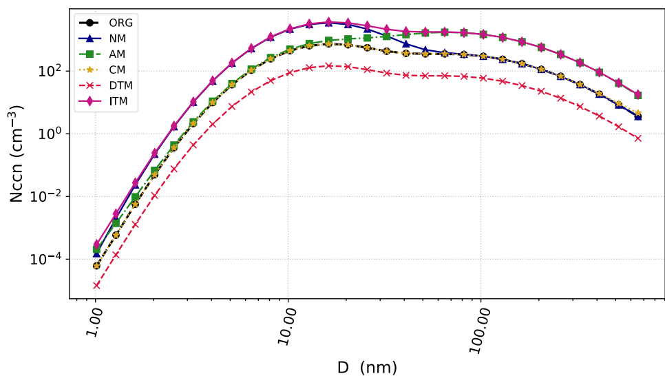
Figure 3: Initial aerosol number concentration (unit: \text{cm}^{-3} ) as a function of particle diameters (unit: nm).
