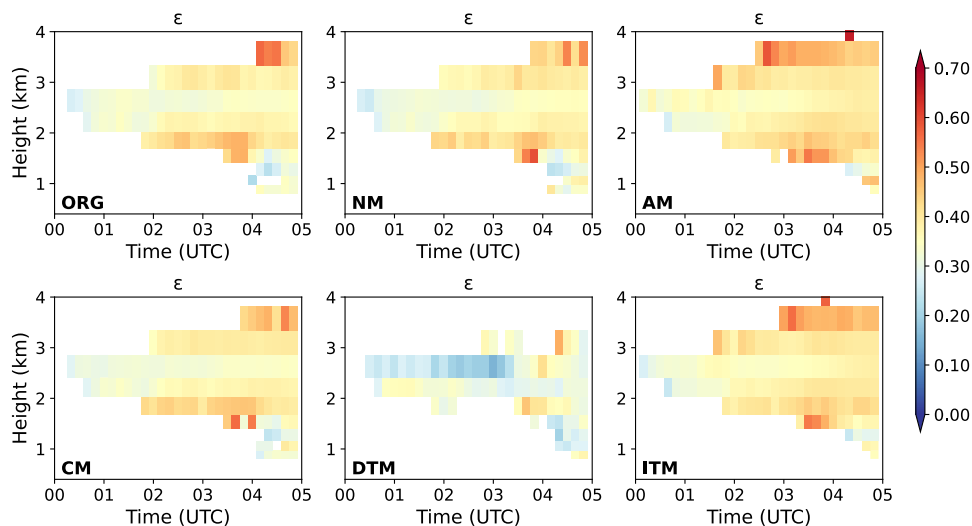
Figure 15: Distribution of relative dispersion ( \epsilon ) of cloud droplet spectrum over time (UTC) and altitude (km). The color shading indicates the magnitude of relative dispersion values.
