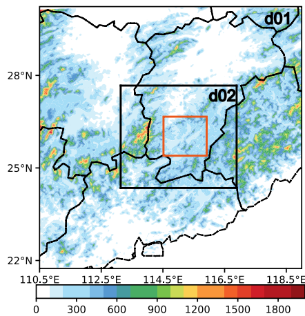
155 Figure 1: Simulated Region and Nesting Configuration. The shading represents the elevation (m) of the terrain, and the area within the red box is the analysis range.
