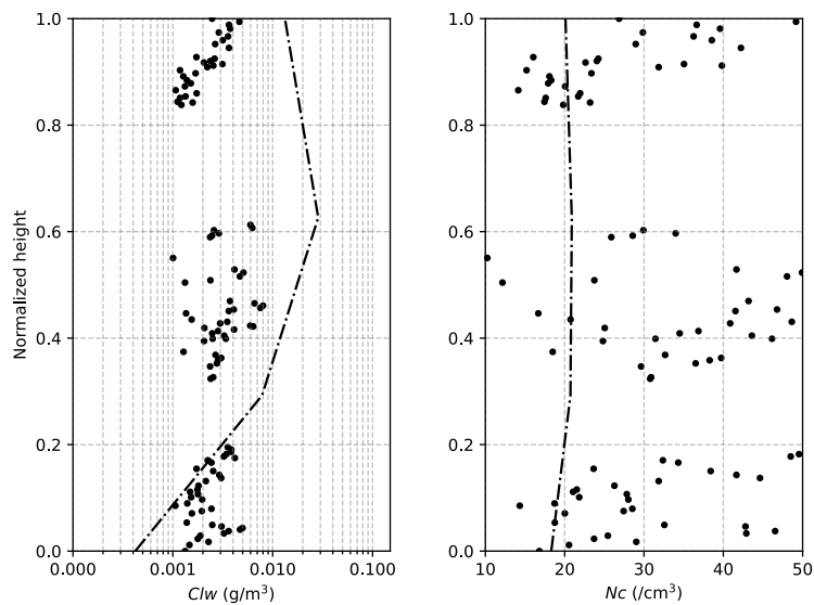
Figure 5: Aircraft observations (scatter points) of cloud liquid water content (Clw, in \text{g/m}^3 ), cloud droplet number concentration ( N_c , in \text{cm}^{-3} ) on December 25, 2014, compared with model simulations (black dashed lines) of Clw and N_c .
