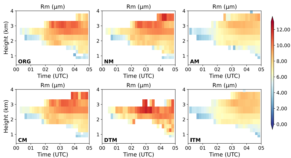
Figure 9: The variations of averaged cloud droplet radius ( R_m , in \mu\text{m} ) with time (UTC) and altitude (km) within the study area of different experiments.
