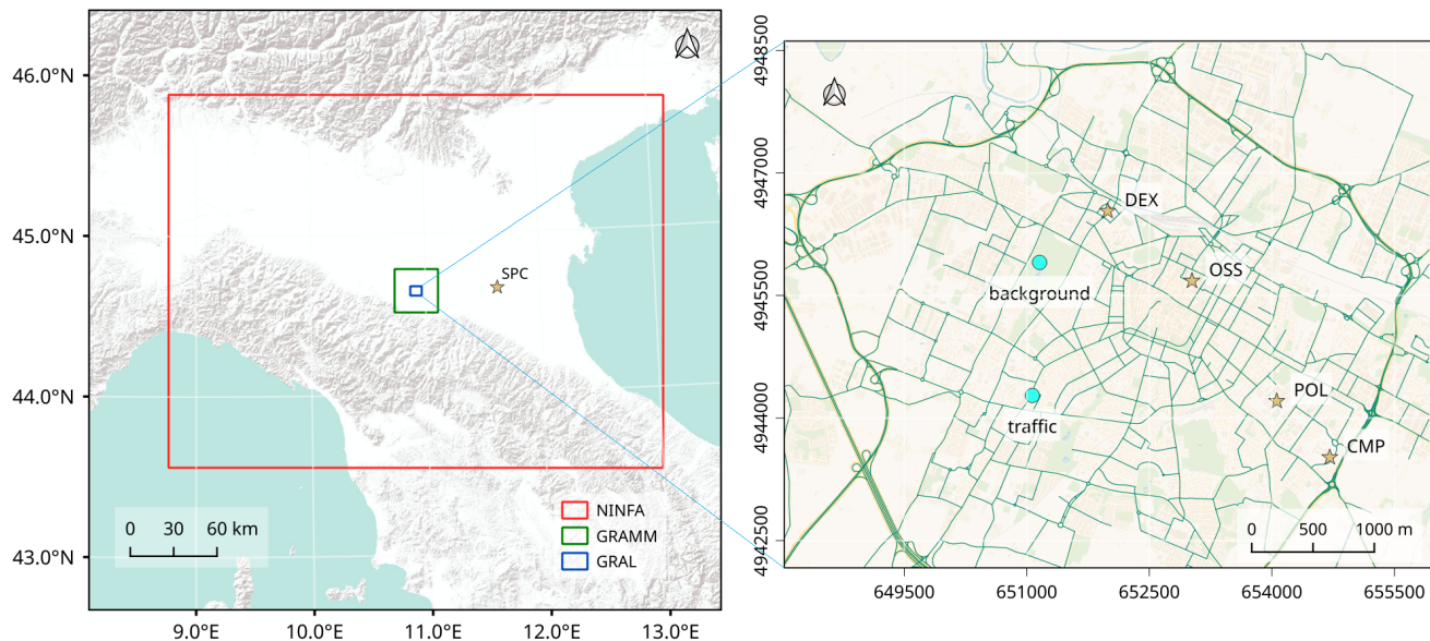
Figure 1. Spatial representation of the NINFA and GRAMM domains on the left, and the GRAL investigation domain on the right. The GRAL domain includes the positions of two urban air quality stations denoted by lightblue dots, specifically one located at the urban traffic (traffic) site and another at the urban background (background) site. Additionally, four meteorological stations used for meteorological validation and for selecting the meso-scale meteorological situation are indicated by yellow stars within the GRAL domain.
