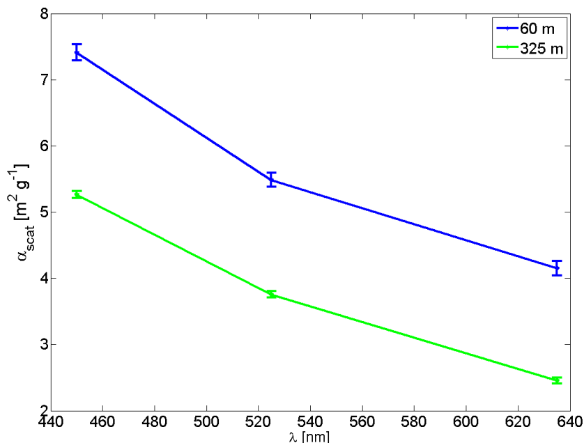
Figure 8. Mass scattering efficiency, \alpha_{scat}(\lambda) , as a function of wavelength for measurements at 60 and 325 m height. Error bars are the standard error.
