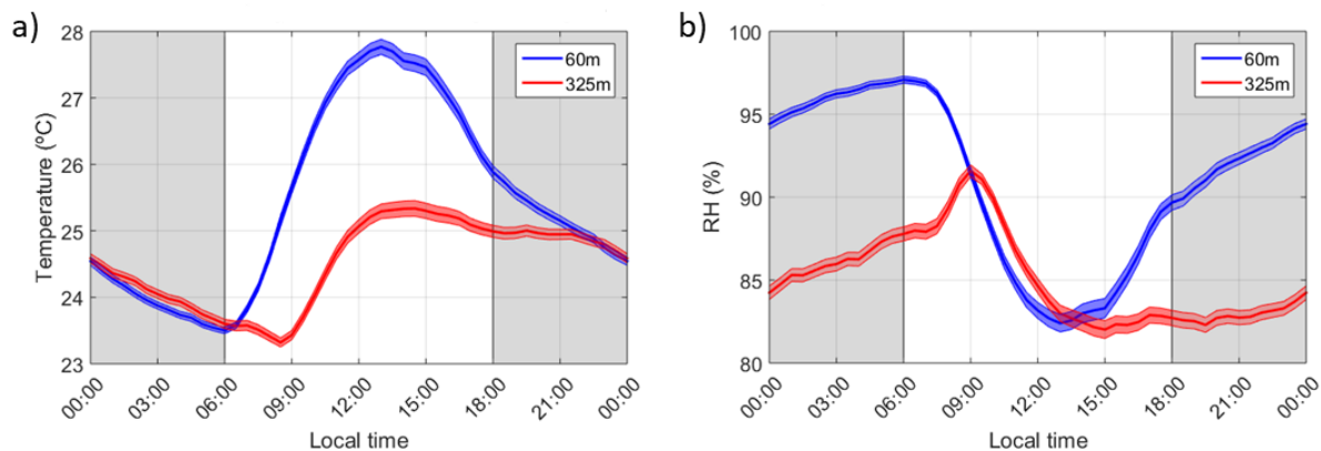
Figure 3. Diurnal cycle of a) temperature and b) relative humidity (RH) at two different heights at the ATTO site during April and May. The blue and red lines represent the averages of the measurements at 60 and 325 m height, respectively, and the shaded areas represent the standard error of the mean. The 60 m measurements were performed between 2013 and 2018, and the 325 m measurements from 2018 to 2022.
