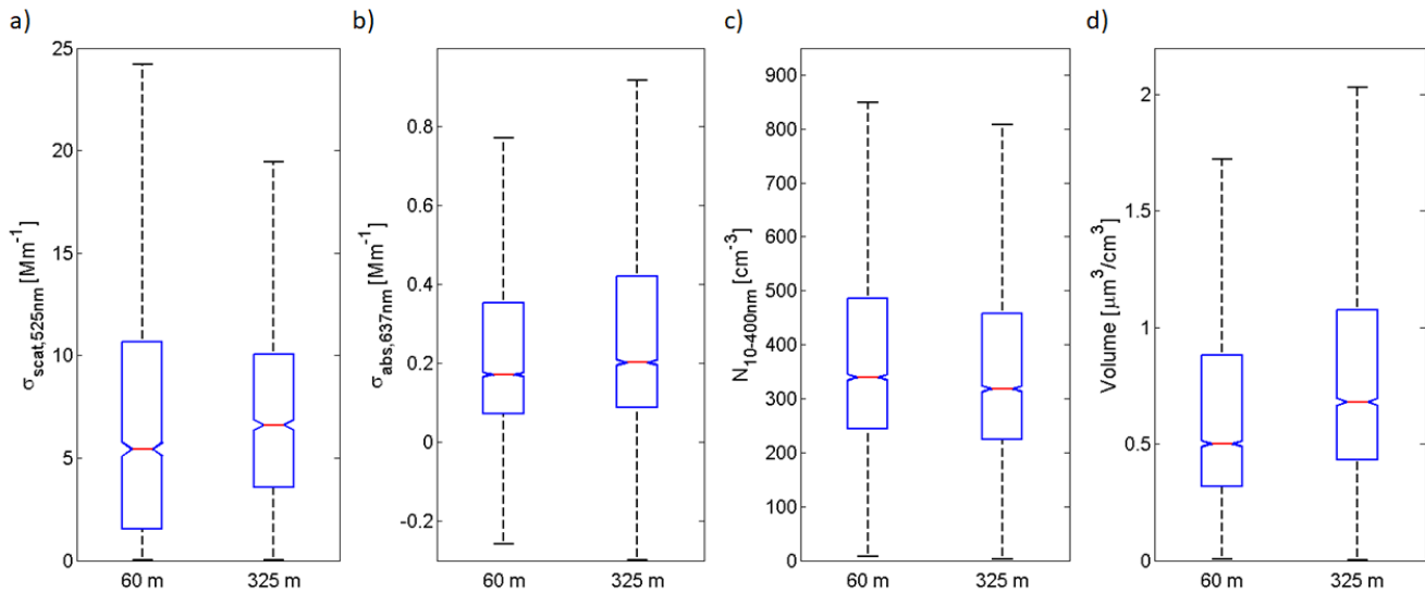
Figure 4. Box-and-whisker plots of the optical aerosol properties during the wet seasons of 2019 and 2020, showing a) \sigma_{scat,525nm} and b) \sigma_{abs,637nm} , c) particle number concentration, and d) aerosol volume at 60 and 325 m height. The boxes represent the quartiles, the whiskers represent the 90th and 10th percentiles, and the horizontal line represents the median.
