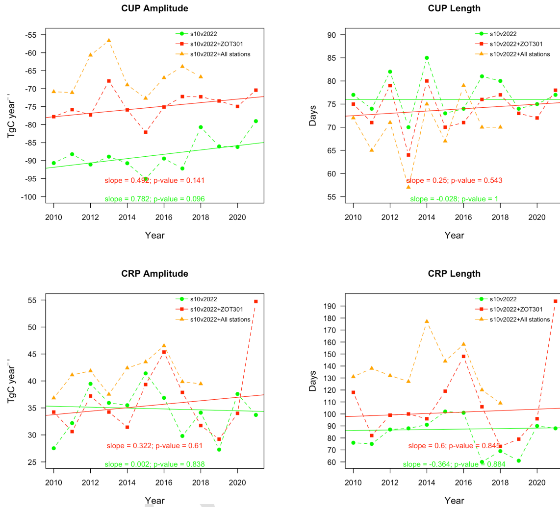
Figure G2. Time series of the intensities of CRP and CUP derived from three inversions with different station sets are listed in Table 1.
