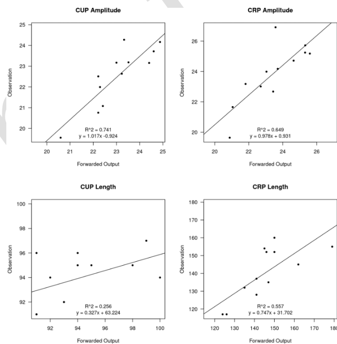
Figure H4. Regression of intensity (i.e. amplitude of length) of CUP and CRP analyses derived from observational data against model forward output mole fraction.
