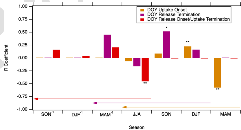
Figure 6. The partial correlation coefficient between seasonal temperature anomalies and the timing of release start (or uptake termination), release termination, and uptake onset controlling for the effects of precipitation and cloud cover over the 2010–2021 period. The timings are correlated with the seasons they fall in and also with three preceding seasons (demonstrated as the length and direction of the arrow of the respective colour). We calculate the partial correlations by selecting every subset of 10 years in the 11-year 2010–2021 period (omitting 1 year in each calculation) and taking their standard deviation as the error bar. Errors bars are small and therefore not visible in this figure. Bars marked with asterisks (*) and double asterisks (**)) indicate that the partial correlation coefficient is significant at p < 0.1 and p < 0.05 , respectively.
