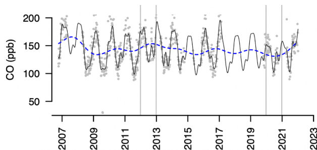
Figure E1. Flask dataset (grey dots) for CO concentration from ZOTTO 301 m a.g.l. The black line is the smoothed curve for the dataset, and the dashed blue line is the running mean.
