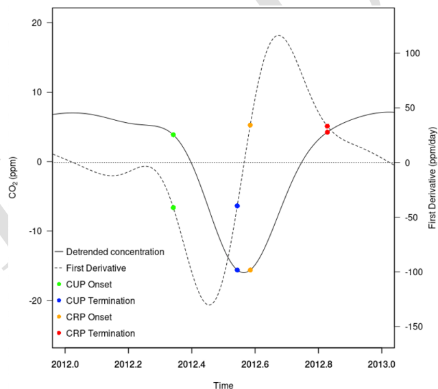
Figure 3. A complete CO 2 seasonal cycle for 2012 (solid line) and its first derivative representing the rate of CO 2 uptake or release (dashed line). The blue and green points mark the time of 30 % of the minimum of the first derivative, while the red and orange points are 30 % of the maximum of the first derivative.
