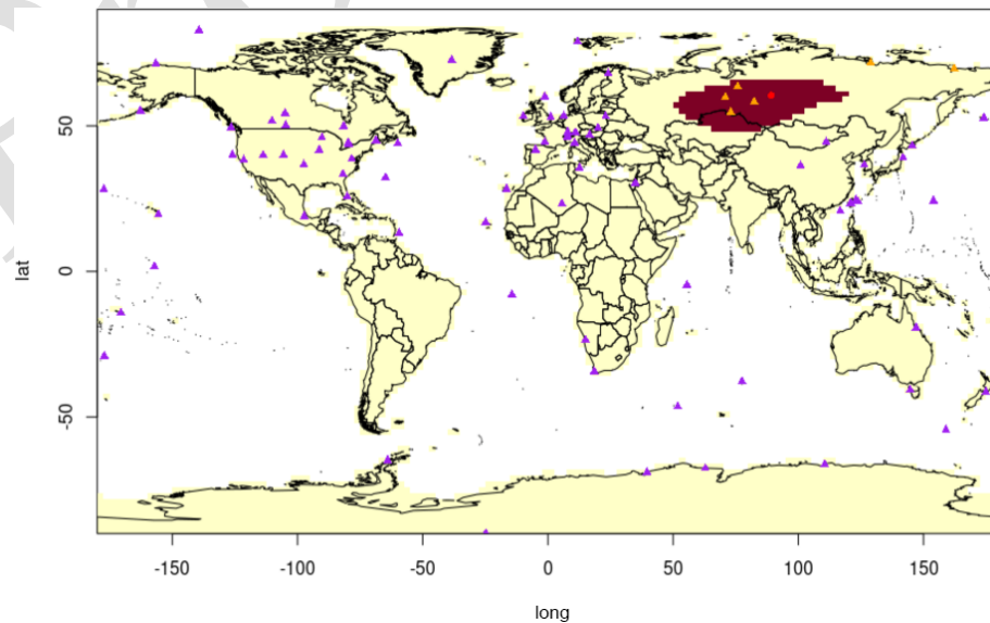
Figure D1. Locations of the stations in the s10v2022 set (purple triangles), ZOTTO (red dot), and the additional six stations (orange triangles) in the s10v2021 + Allstations set. The red shading is the averaged influencing region for the ZOTTO observational dataset.
