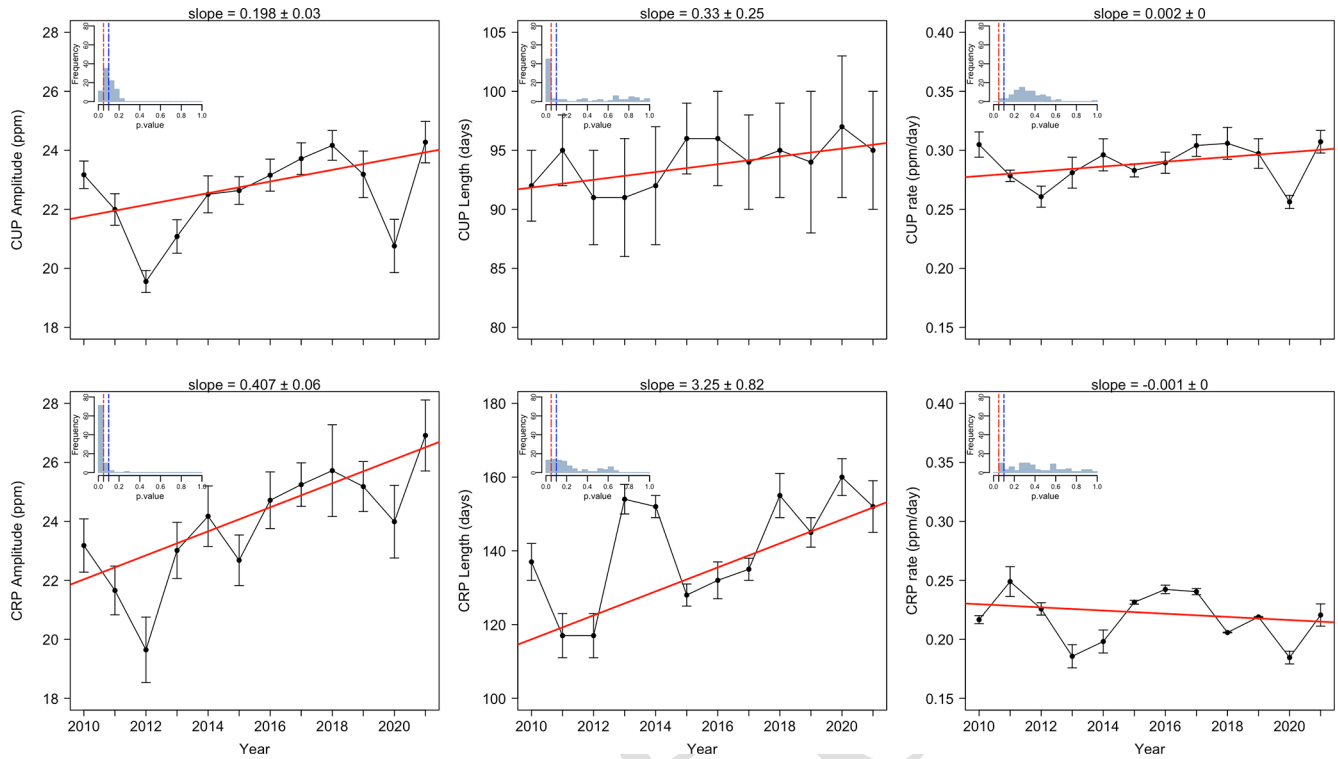
Figure 7. Time series of the length and amplitude of CRP and CUP. Inset histograms show the frequency of p values of the Theil–Sen regressions of the 100-member curve-fitting ensemble, with dashed vertical red and blue lines, respectively, indicating the 0.05 and 0.1 significant difference from 0 of the slope. Error bars are the standard deviations from the mean of the 100-member curve-fitting ensemble.
