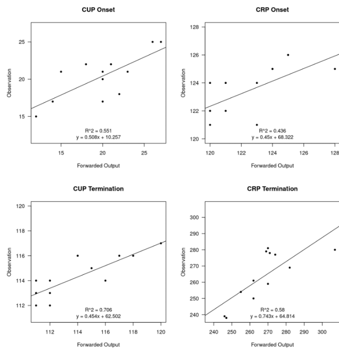
Figure H3. Regression of the timing of the CUP and CRP onset and termination derived from observational data against model forward output mole fraction.
