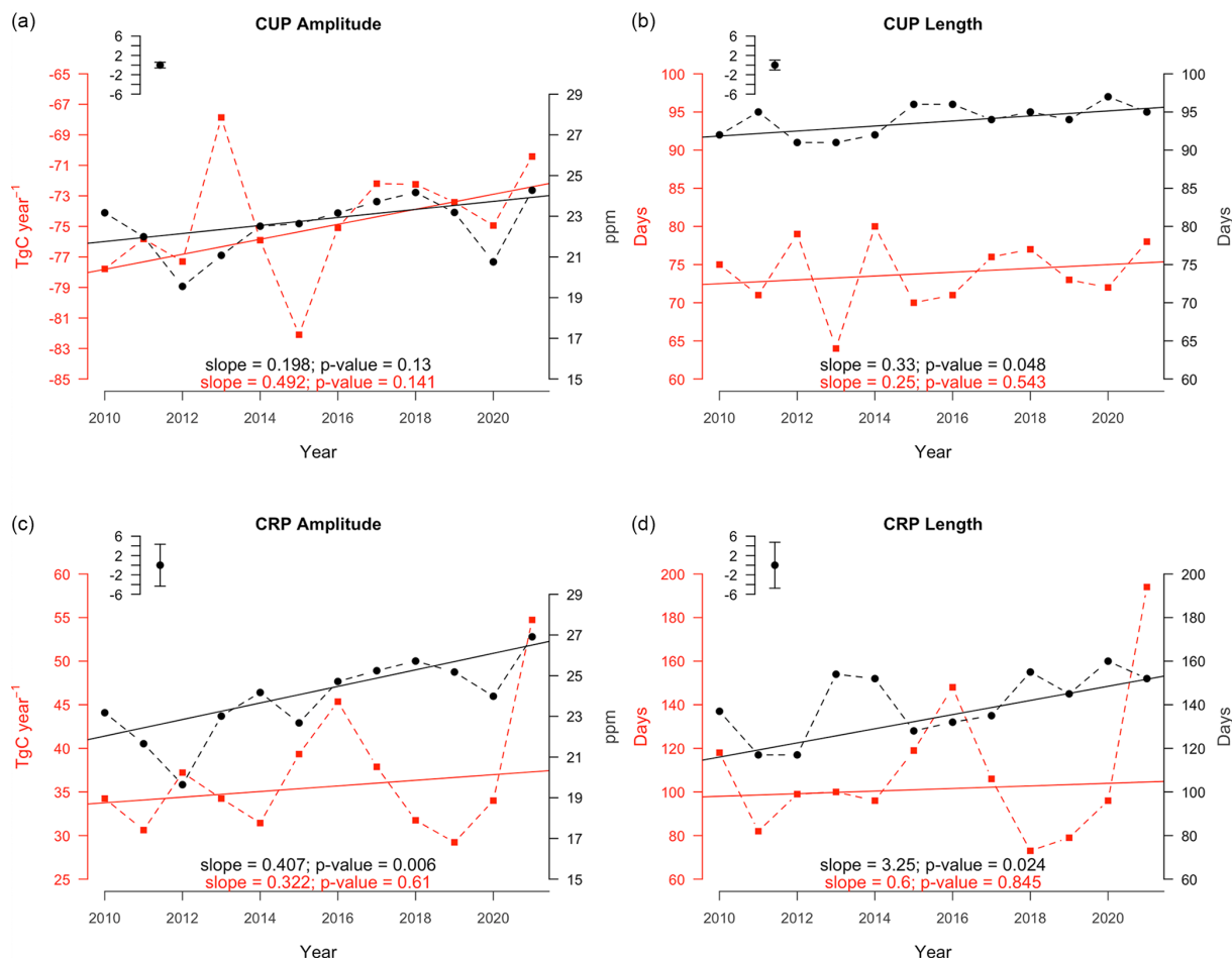
Figure 10. Time series of the amplitudes and lengths of CRP and CUP derived from atmospheric mole fractions (black circle) and regional fluxes (red square). The small bar plot on the top left of each panel indicates the 2010–2021 averaged error in the observational analysis.
