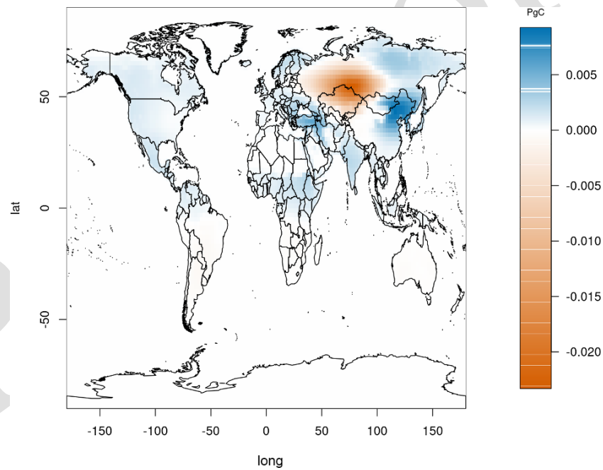
Figure G4. Spatial differences in the 2010–2021 mean NEE between the inversions using station sets s10v2021 and s10v2021 + ZOT.
