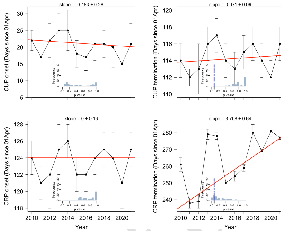
Figure 5. Time series of the timings of the CRP and CUP onset and termination. Inset histograms show the frequency of p values of the Theil–Sen regressions of the 100-member curve-fitting ensemble, with dashed vertical red and blue lines, respectively, indicating the 0.05 and 0.1 significant difference from 0 of the slopes. Error bars are the standard deviations from the mean of the 100-member curve-fitting ensemble.
