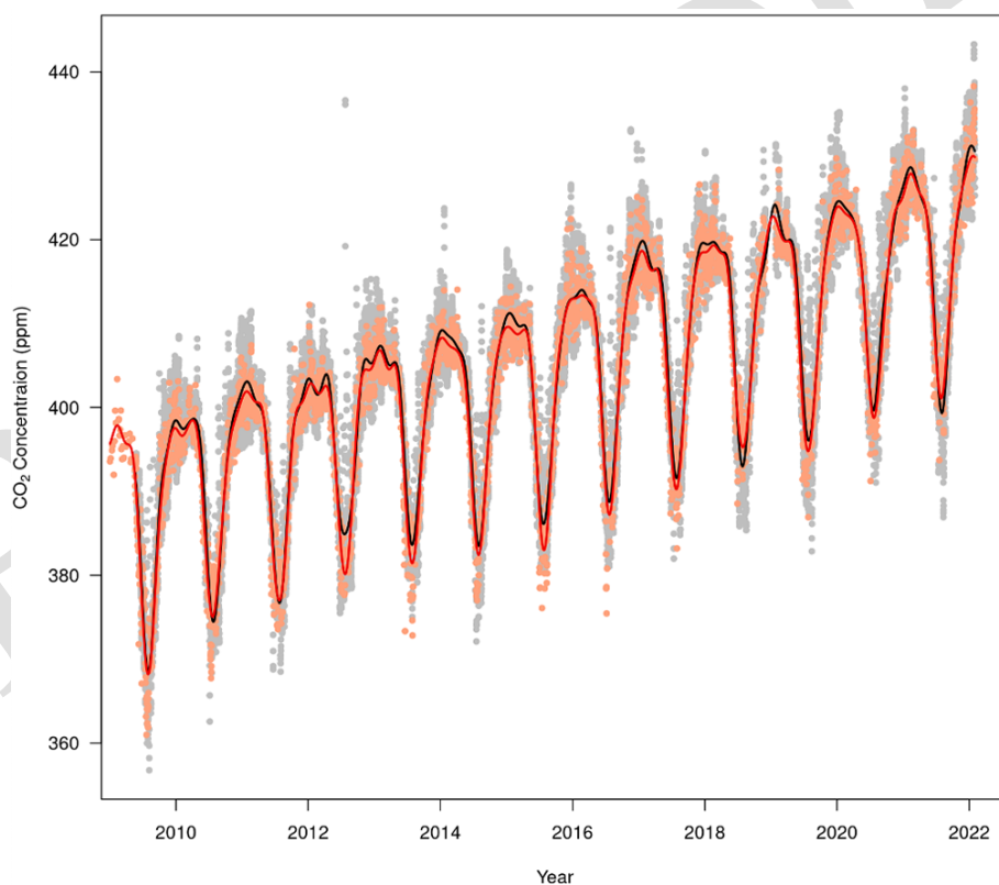
Figure F1. Observed CO 2 mole fraction time series of ZOTTO (grey dots) and corresponding inversion forward simulation (s10v2022 + ZOT) (light salmon dots); smoothed CO 2 concentration time series of ZOTTO-observed data (black line) and inversion model forward outputs (red line) obtained from the Thoning et al. (1989) algorithm using short-term cut-off = 88 d, long-term cut-off = 667 d, number of harmonics = 2, and degree of polynomial = 3.
