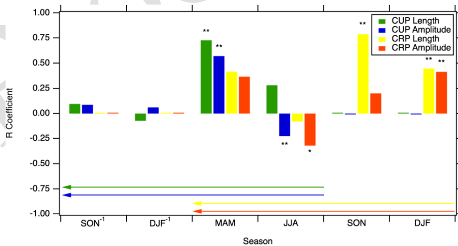
Figure 8. The partial correlation coefficients between seasonal temperature anomalies and the amplitude and length of CUP and CRP, controlling for the effects of precipitation and cloud cover over the 2010–2021 period. The amplitude and length are correlated with the season when CRP and CUP end and also with three preceding seasons (demonstrated as the length and direction of the respective colour). We calculate the partial correlations by selecting every subset of 10 years in the 11-year 2010–2021 period (omitting 1 year in each calculation) and taking their standard deviation as the error bar. Errors bars are small and therefore not visible in this figure. The asterisks (*) and **) indicate that the partial correlation coefficient is significant at P < 0.1 and P < 0.05 , respectively.
