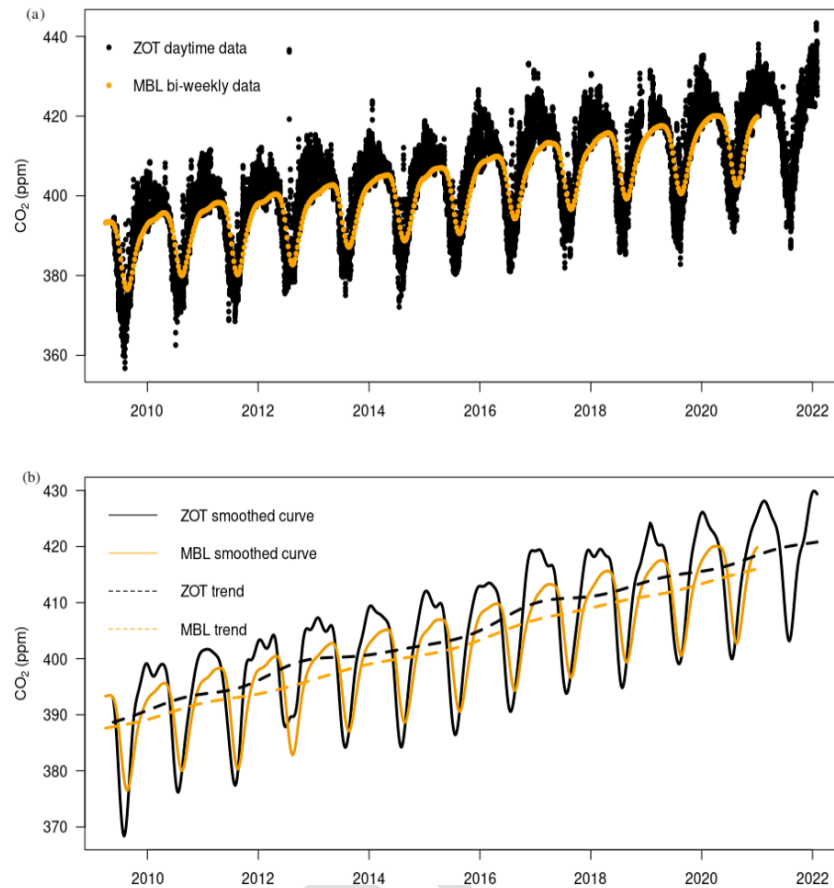
Figure 4. (a) Daytime CO 2 time series of the continental ZOTTO station in comparison to the bi-weekly marine boundary layer (MBL). (b) Time series of panel (a) smoothed by the Thoning et al. (1989) algorithm.
