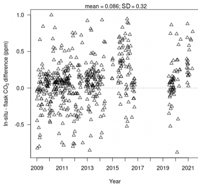
Figure 2. Differences between deconvolved (Sect. 2.1) in situ and flask data for CO 2 .
