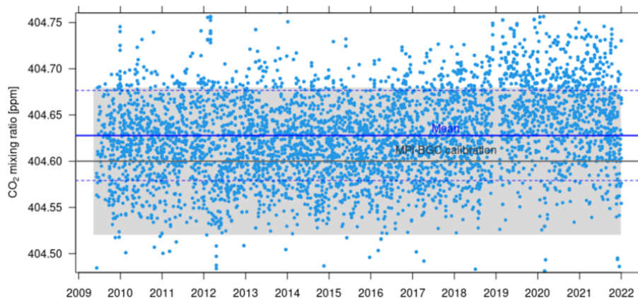
Figure 1. Target tank time series (solid and dashed blue lines represent the mean \pm standard deviation; solid grey line and grey shading is the Jena GasLab standard \pm error).
