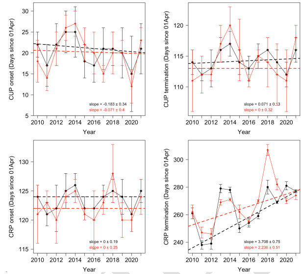
Figure H1. Time series of the timing of CRP and CUP derived from observation (in black) and model forward (s10v2022 + ZOT simulation) (in red) mole fraction analysis.
