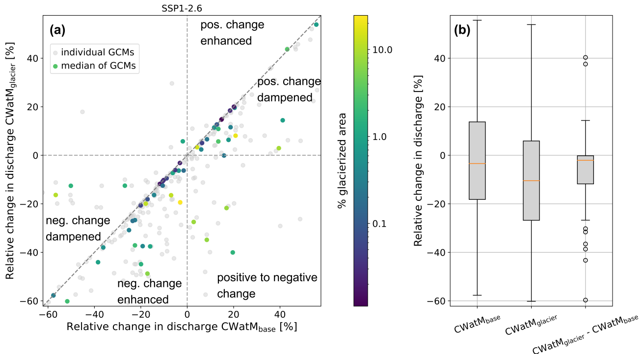
Figure 9. Comparison of relative future discharge change for the month with largest absolute glacier-sourced melt contribution in the past, at end of the 21 st century, considering both CWatM_{base} and CWatM_{glacier} , across 56 glacierized river basins for SSP1-2.6. (a) Colored dots show the median of all GCMs and grey dots show individual GCMs. (b) Boxplots show the relative future change of all basins for CWatM_{base} and CWatM_{glacier} and the difference between the two.
