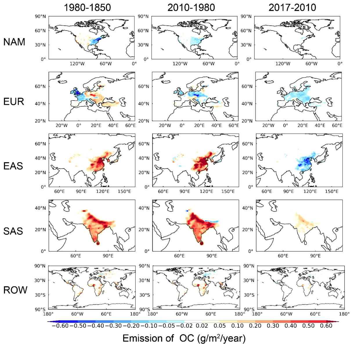
28 Figure S2. Changes in anthropogenic emissions of organic carbon (OC) between 29 1850 and 1980 (left), between 1980 and 2010 (middle), and between 2010 and 2017 30 (right) in the 5 tagged source regions (NAM, EUR, EAS, SAS and ROW from top to 31 bottom).
