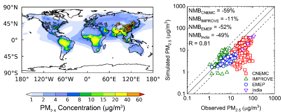
Figure 1. Spatial distribution (left panel) and scatter plot (right) between the simulated and observed annual mean near-surface PM 2.5 concentrations ( \mu\text{g m}^{-3} ) in 2017. Observational data are from IMPROVE (triangle), EMEP (circle), India (inverted triangle) and CNEMC (square). The solid line marks the 1:1 ratio and dashed lines mark the 1:2 and 2:1 ratios. Normalized mean bias (NMB) and correlation coefficient (R) between observation and simulation are shown on the right panel. \text{NMB} = 100\% \times \sum(M_i - O_i) / \sum O_i , where M_i and O_i are the modeled and observed values at site i , respectively.
