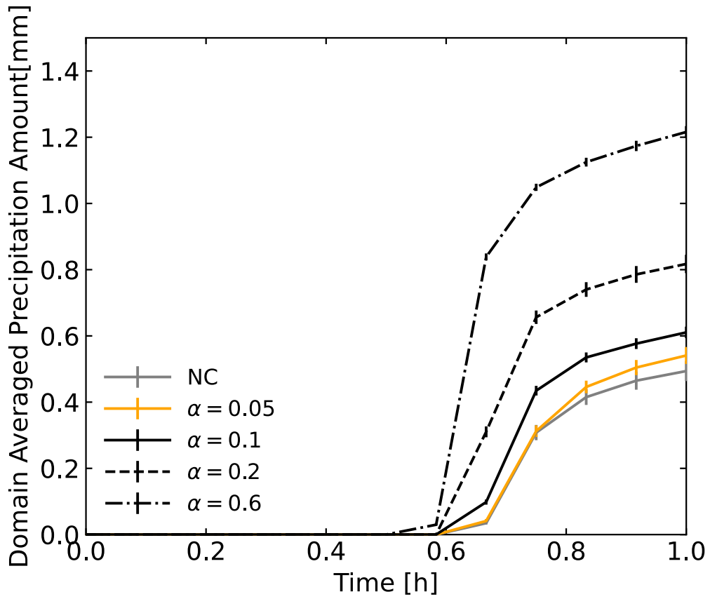
870 Figure 6: A comparison of the evolution of the domain-averaged precipitation amount with variable droplet charging rate \alpha is 0.05 (orange solid line), 0.1 (black solid line), 0.2 (black dashed line), and 0.6 (black dashed-dotted line), and the electric force is evaluated with the CS setting. The grey solid line represents the NC setting.
