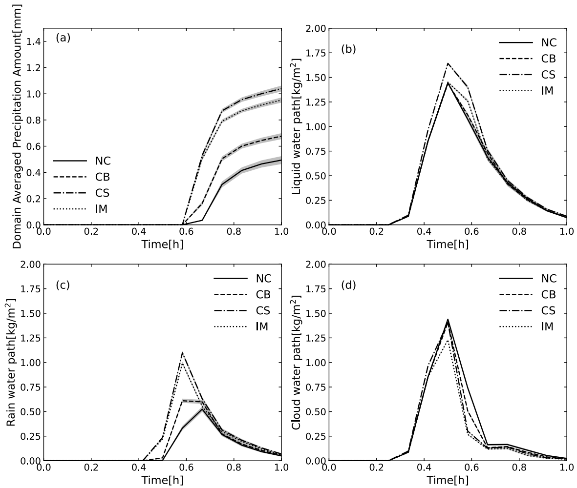
835 Figure 3: The time evolution of the domain-averaged precipitation amount (a) and the domain-averaged water path of the liquid water path (b), rainwater path (c) and cloud water path (d), which is consistent with Figure 2. The solid line represents NC setting, the dashed line represents CB setting, and the dashed-dotted line represents CS setting. The grey shade indicates the standard deviation calculated from 50 members of the random ensemble.
