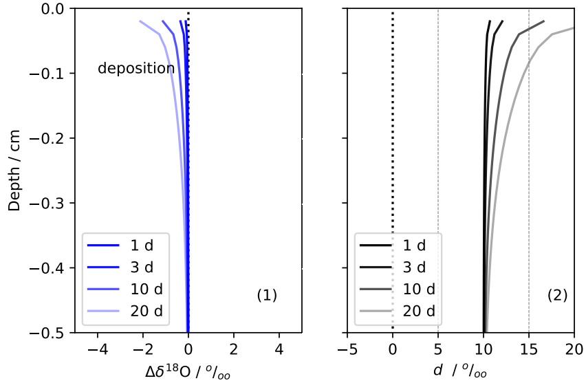
(a) FV_{dep} , T_{snw} = -15\text{ }^{\circ}\text{C} , T_{atm} = -10\text{ }^{\circ}\text{C} , u = 5\text{ m s}^{-1}
