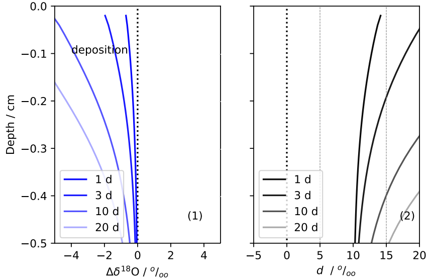
(a) FV_{dep} , T_{snw} = -15\text{ }^{\circ}\text{C} , T_{atm} = -10\text{ }^{\circ}\text{C} , u = 20\text{ m s}^{-1}
