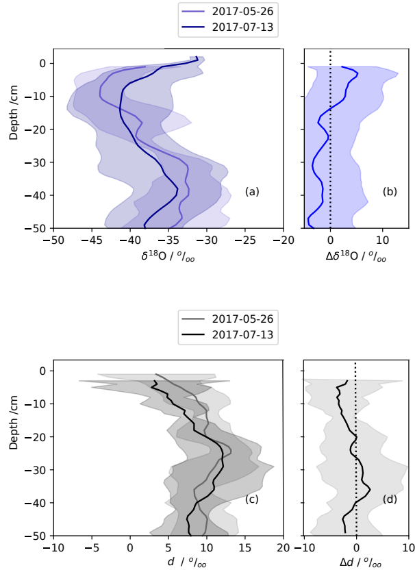
Figure 4. The mean isotopic change in near-surface from a low accumulation period during summer (25 May 2017 and 13 July 2017). Panels (a) and (c) are the mean snow profiles of \delta^{18}\text{O} and d computed from four snow profiles each. Panels (b) and (d) show the isotopic change over this time period. Error bars are 2\sigma standard error.
